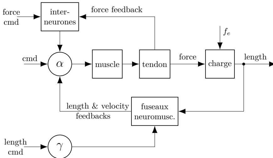
Figure 1.8: Spinal stretch reflex control action
