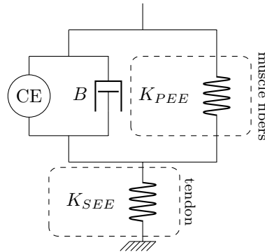
Figure 1.7: Hill's muscle model
