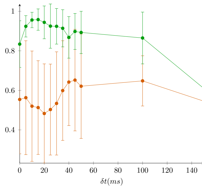
FIGURE 13 – Mean R^2 related to the identification of the KBI model, against \delta t delay, for impedance evaluations both for the 11 perturbed trajectories selected (green) and non perturbed trajectories at the same position in the next cycle (orange). Standard deviation are indicated with bars.
