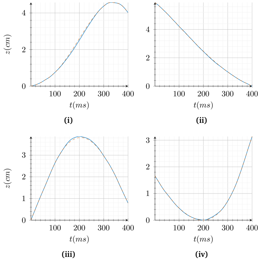
FIGURE 8 – Real trajectories (solid blue lines) and estimated trajectories (dashed orange lines), for the 4 different phases, i) rising, ii) decreasing, iii) upper peak ; iv) lower peak. The interpolation is done using the trajectories both before 100 ms and after 300 ms. The estimated window is therefore, the data between 100 ms and 300 ms.
