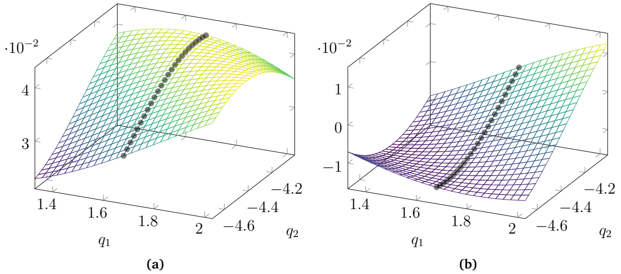
FIGURE 13 – Variation of terms from matrix (40), for q_3 = 1.5 , q_1 = 1.68 is notified by the circular black markers (a) Diagonal term on x , (b) Coupling term on x multiplied by f_z . Joint values are provided in radians.
