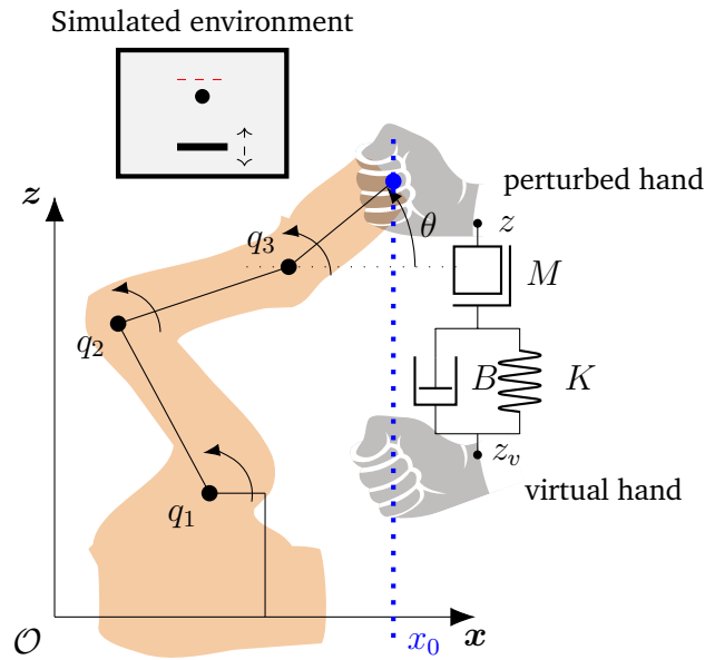
FIGURE 2 – Proposed interactive system for impedance estimation : a human interacts with the 3 DOF robot thanks to a handle. q_i are the joint positions of the robot, \theta is the endpoint orientation, z is the endpoint position along the z axis, represented here after a perturbation responsible for the hand deviation from it's nominal trajectory denoted by z_v , the virtual position.
