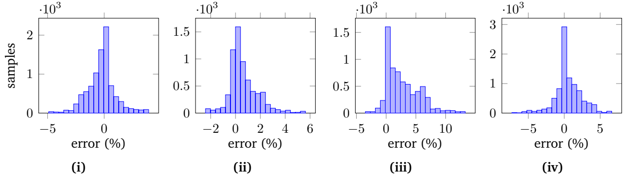
FIGURE 9 – Normalized position error histograms
