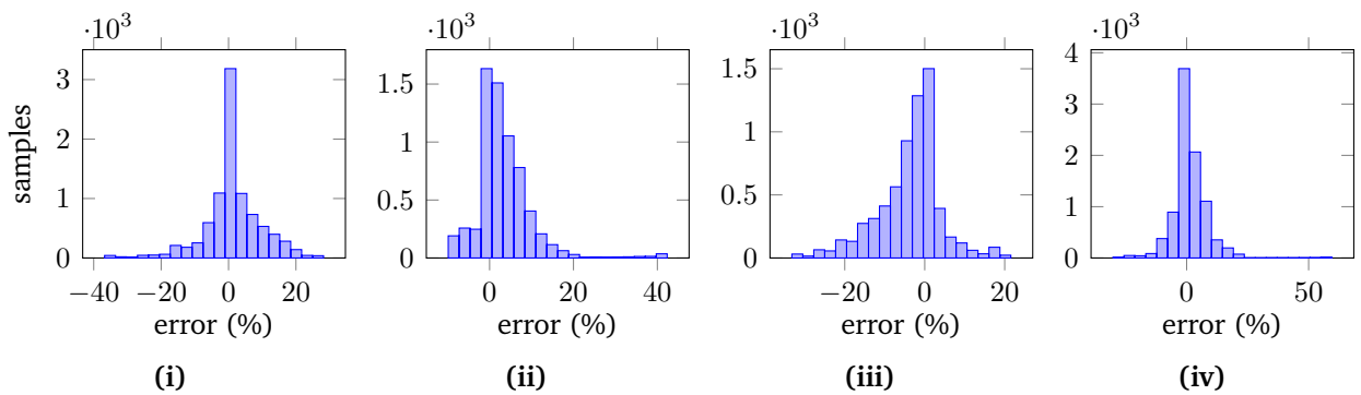
FIGURE 10 – Normalized force error histograms
