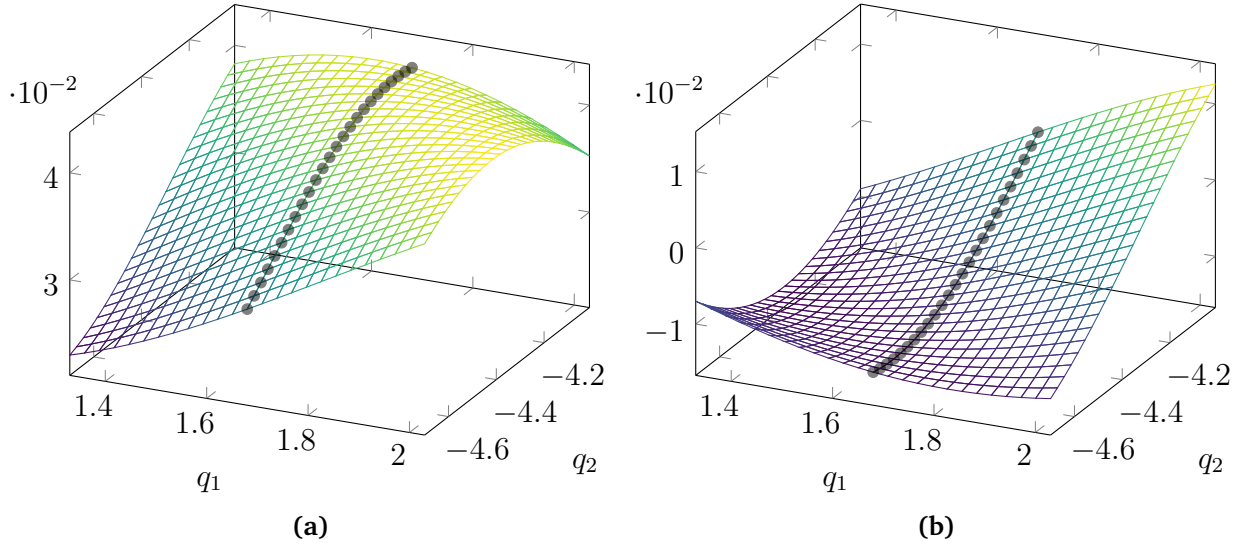
FIGURE 17 – Variation of terms from matrix (41), for q_3 = 1.5 , q_1 = 1.68 is notified by the circular black markers (a) Diagonal term on x , (b) Coupling term on x multiplied by f_z . Joint values are provided in radians.
