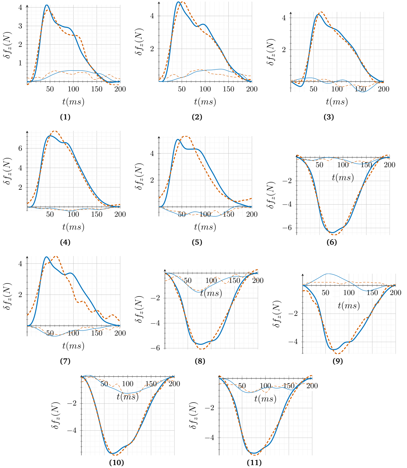
FIGURE 15 – Reconstructed forces for the 11 perturbations selected. Solid lines represent \delta f_z and dashed lines represent the reconstructed force using the identified parameters of KBI model. Thinner lines are for the evaluation when no perturbation occurred.
