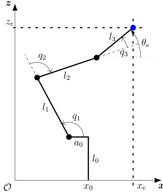
FIGURE 16 – Simplified model of the robot, with 3 actuated joints, and 3 degrees of freedom.
