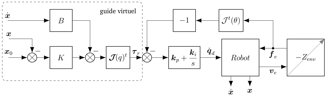
FIGURE 4 – Cartesian virtual fixture using proportional derivative control, added to the natural admittance controller.
