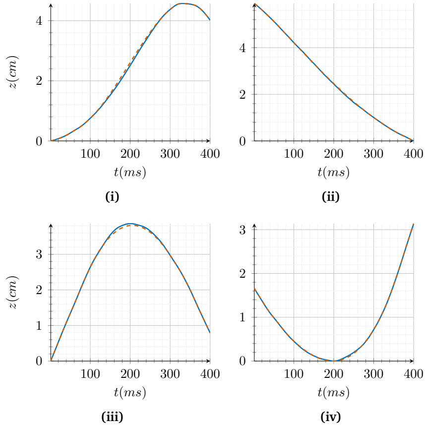
FIGURE 8 – Real trajectories (solid blue lines) and estimated trajectories (dashed orange lines), for the 4 different phases, i) rising, ii) decreasing, iii) upper peak; iv) lower peak. The interpolation is done using the trajectories both before 100 ms and after 300 ms. The estimated window is therefore, the data between 100 ms and 300 ms.
