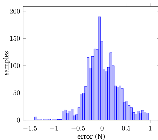
FIGURE 14 – Force reconstruction error histogram.
