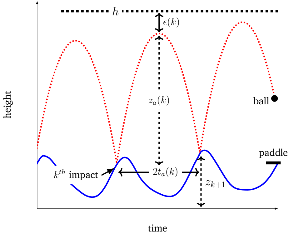
FIGURE 1 – Paddle (solid blue line) and ball (red dotted line) trajectories during the ball bouncing task with target height h (black dashed line).
