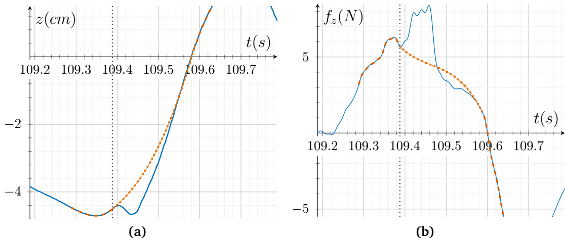
FIGURE 7 – (a) Hand position and (b) Interaction force, both along the z -axis : realized perturbed trajectories (blue solid lines), versus estimated virtual trajectories (orange dotted lines), with the onset time of the perturbation of 30ms duration (vertical black dotted lines).
