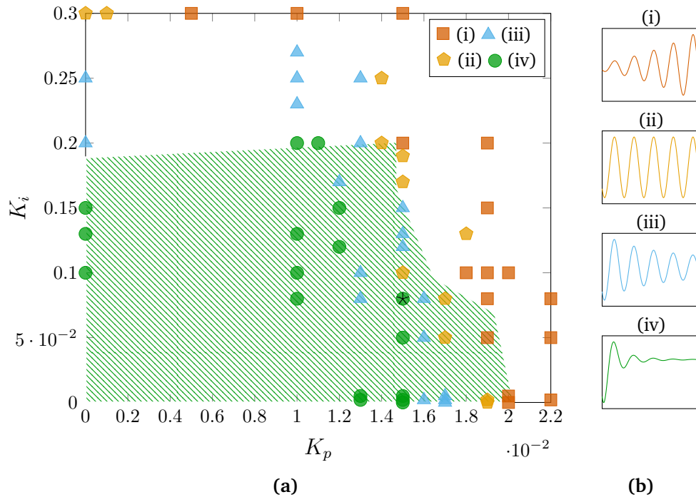
FIGURE 6 – (a) Experimental stability mapping depending on the admittance control gains. Condition 1 : co-manipulation with intentionally high co-contractions of both hand and arm (shapes). Condition 2 : co-manipulation with normal co-contractions of both hand and arm during ball bouncing (green hatched area for comfortable manipulation (iv)). The gains used in the experimental set up are indicated with a star. (b) Categories of typical force responses.
