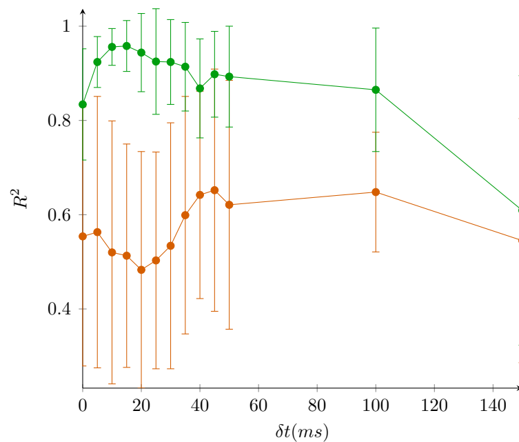
FIGURE 13 – Mean R^2 related to the identification of the KBI model, against \delta t delay, for impedance evaluations both for the 11 perturbed trajectories selected (green) and non perturbed trajectories at the same position in the next cycle (orange). Standard deviations are indicated with bars.
