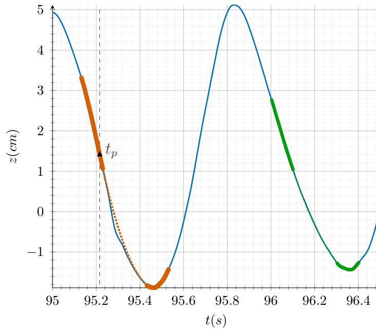
FIGURE 12 – Example of the mocap position trajectory reconstruction, with and without perturbation. Motion capture position is given in blue, thick colored curves indicate the portion used for the spline interpolation, while the colored dotted curves notify the results of the interpolation. The black triangle shows the timing the perturbation was introduced.
