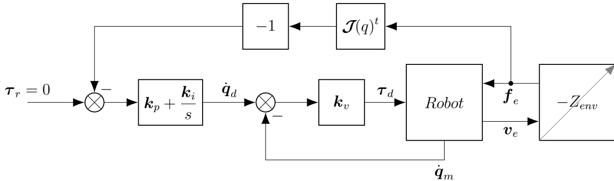
FIGURE 3 – Bloc diagram of the admittance control with a force sensor, proposed by Lamy et al. (2009)
