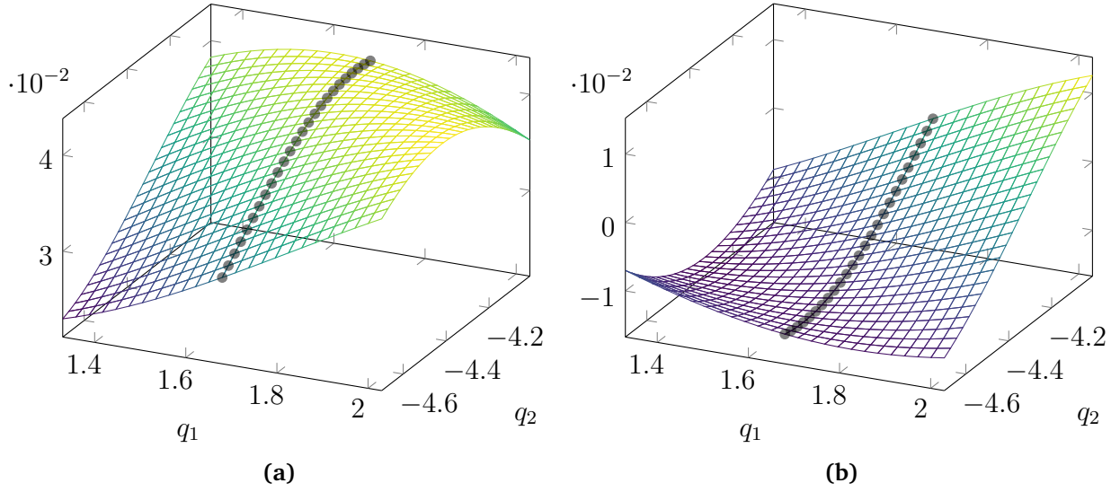
FIGURE 17 – Variation of terms from matrix (C.2), for q_3 = 1.5 , q_1 = 1.68 is notified by the circular black markers (a) Diagonal term on x , (b) Coupling term on x multiplied by f_z . Joint values are provided in radians.
