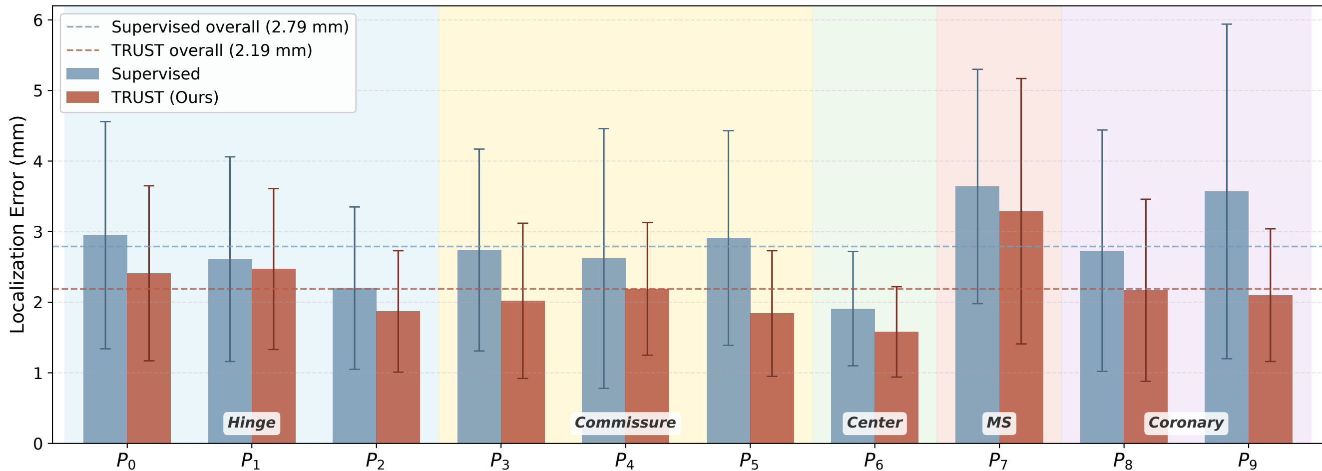
Per-Landmark Localization Error: Supervised vs. TRUST
