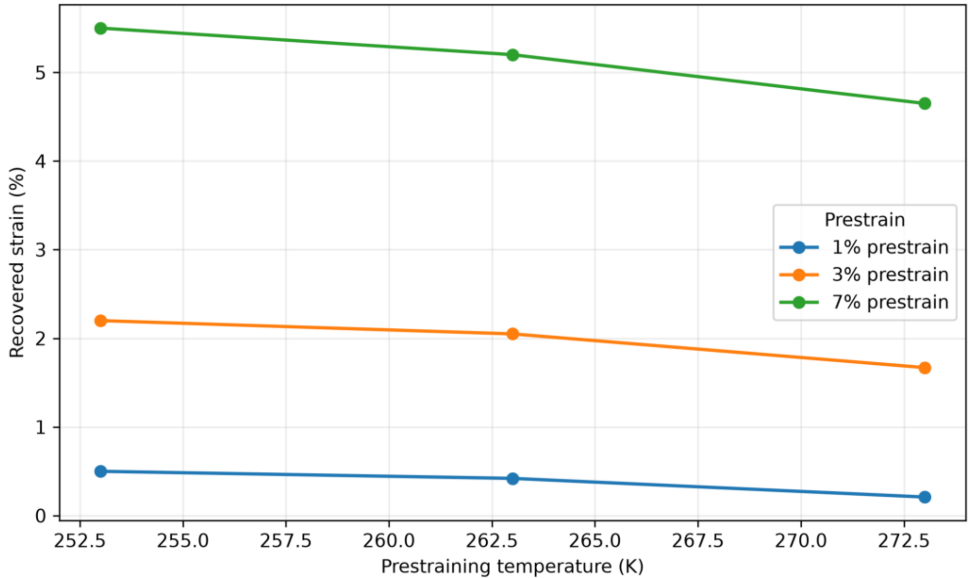
Recovered Strain vs Prestraining Temperature
