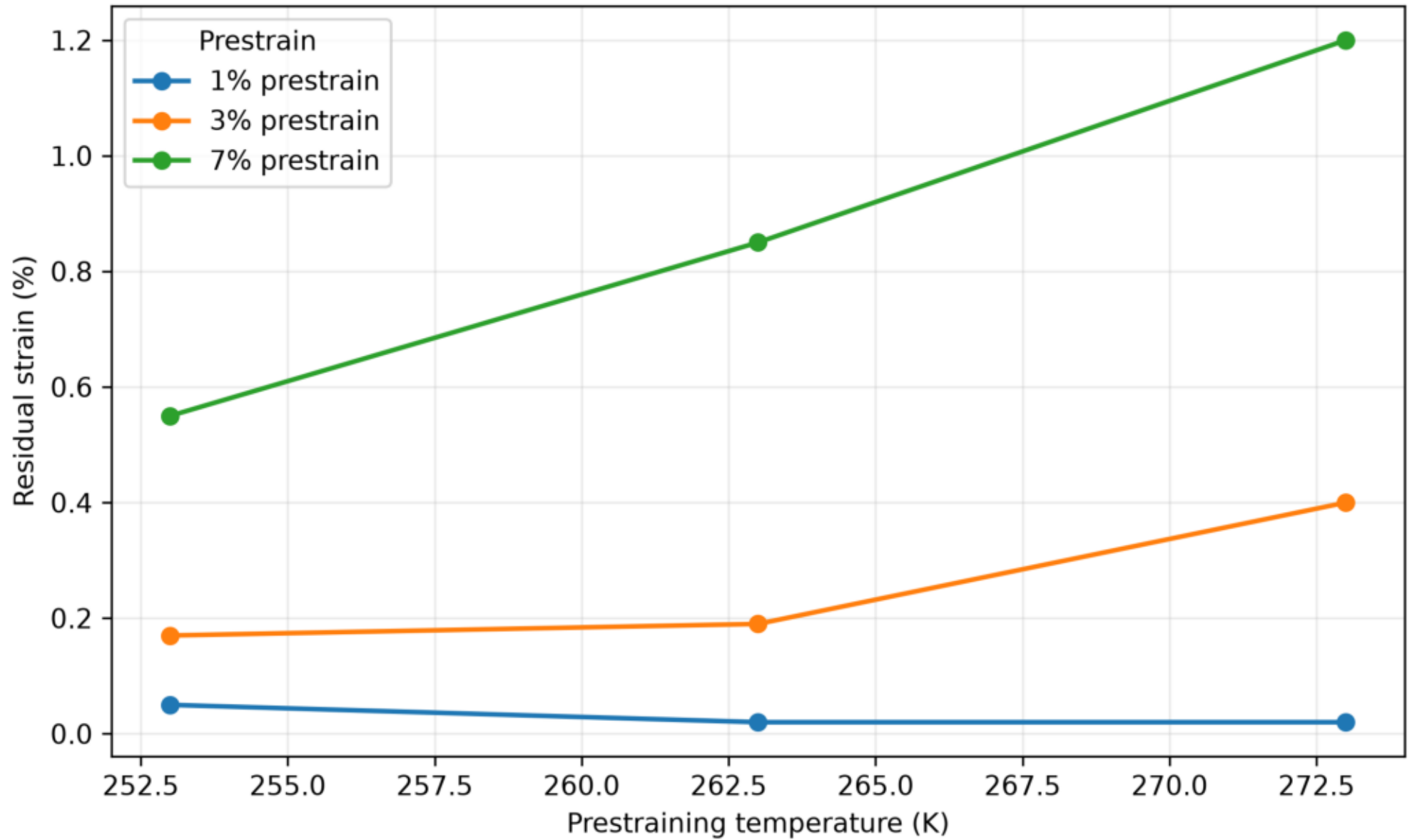
Residual Strain vs Prestraining Temperature
