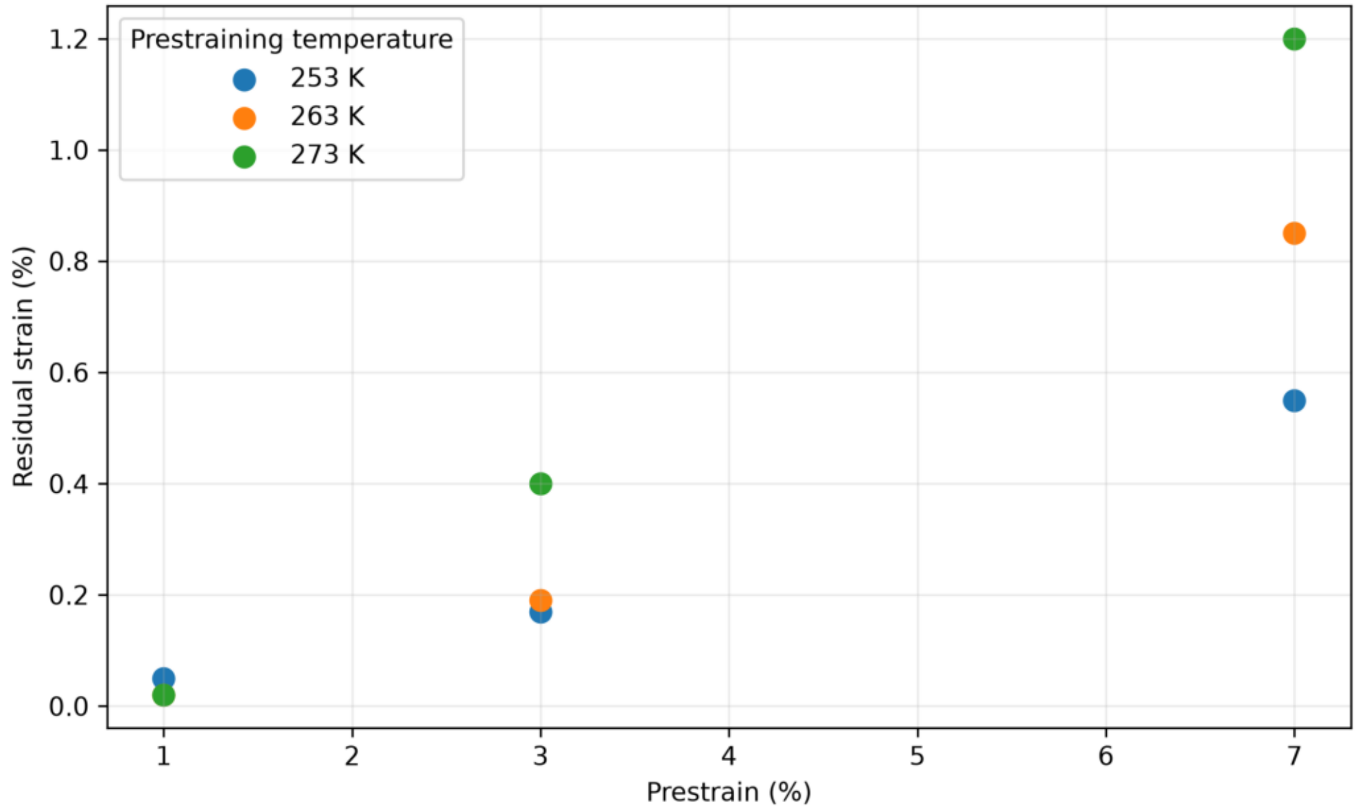
Prestrain vs Residual Strain
