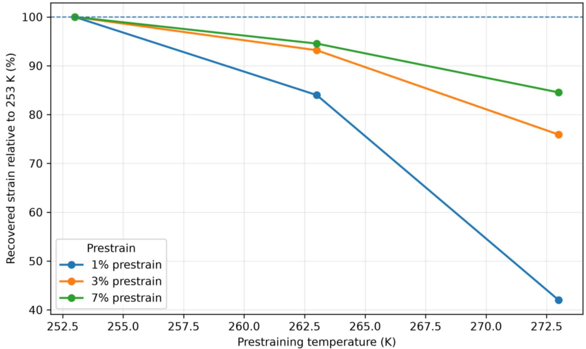
Within-Group Temperature Sensitivity of Recovery
