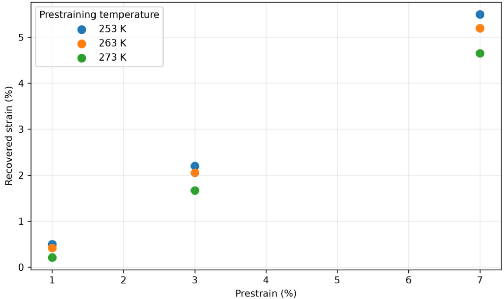
Prestrain vs Recovered Strain
