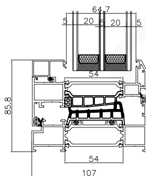
Triple Glazed
