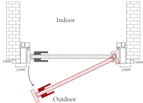
Single Casing / Outward Flush Outward / LH Lock
