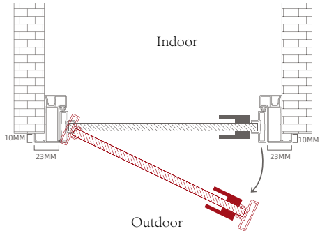
Single Casing / Outward Flush Outward / RH
