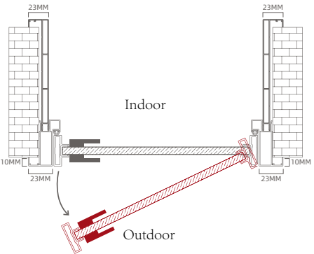
Double Casing / Outward Flush Outward / LH Lock
