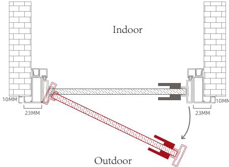
Single Casing / Outward Flush Outward / RH
