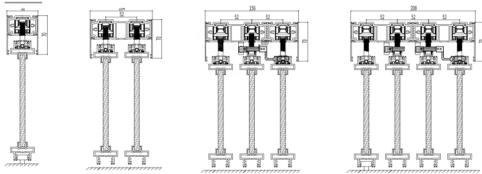
Single Track: 52mm
