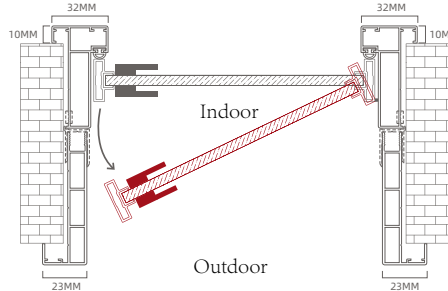
Double Casing / Inward Flush Outward / LH Lock
