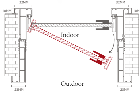
Double Casing / Inward Flush Outward / RH Lock
