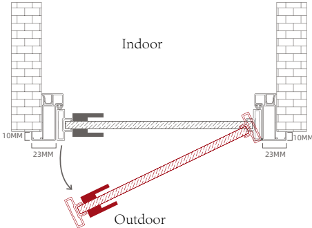
Single Casing / Outward Flush Outward / LH Lock
