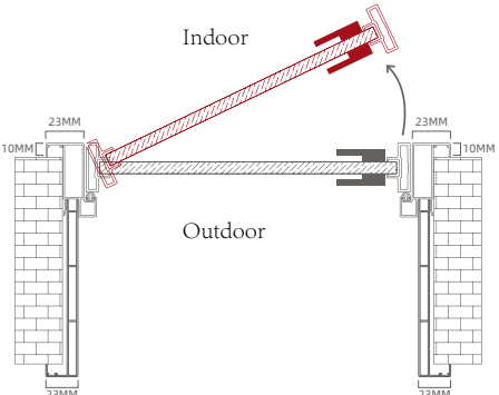
Double Casing / Intward Flush Intward / RH Lock
