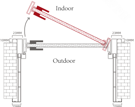
Double Casing / Inward Flush Intward / LH Lock
