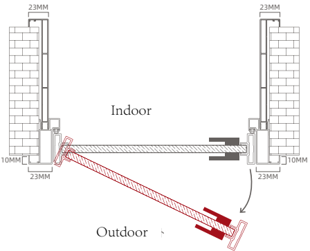
Double Casing / Outward Flush Outward / RH Lock
