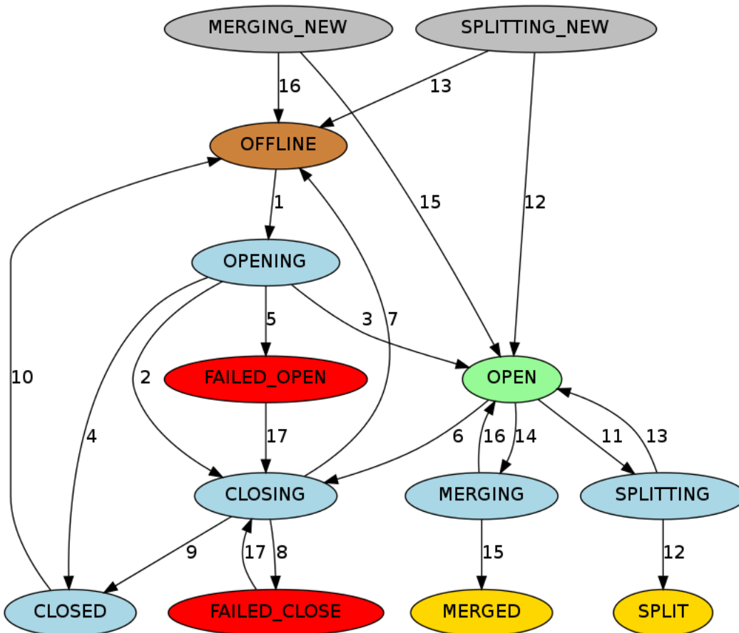
Figure 3. Region State Transitions
