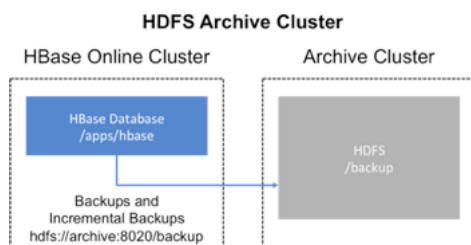
Figure 6. Dedicated HDFS Cluster Backup
