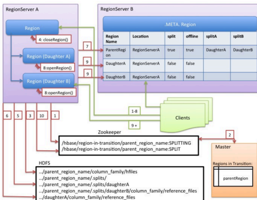
Figure 1. RegionServer Split Process
