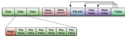
Figure 22. HFile V1 Format
