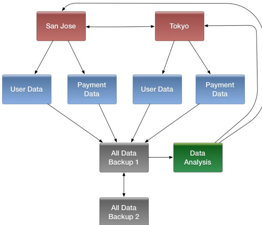
Figure 17. Example of a Complex Cluster Replication Configuration
