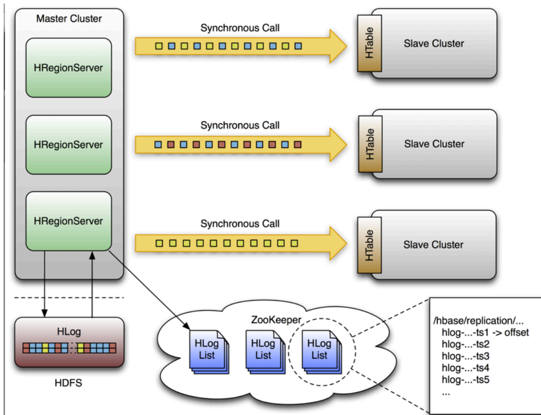
Figure 18. Replication Architecture Overview
