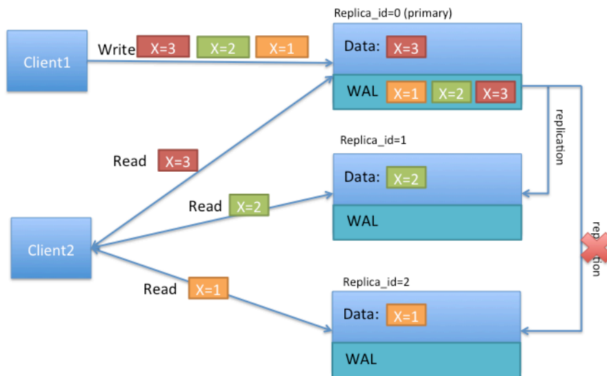
Figure 4. Timeline Consistency
