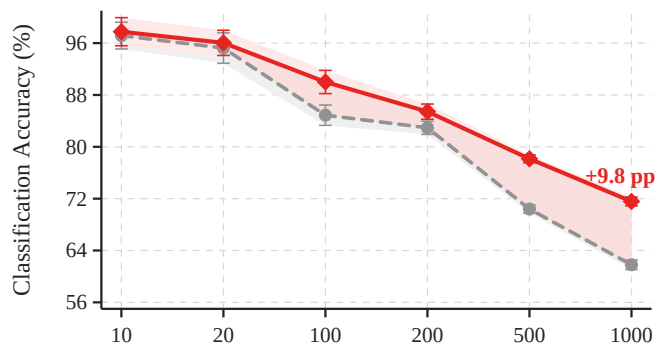
(a) Qwen2.5-VL-7B-Instruct
