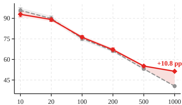
(b) Qwen3-VL-2B-Instruct
