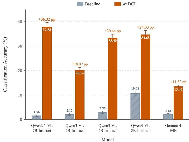
(a) Locally deployed open-source models
