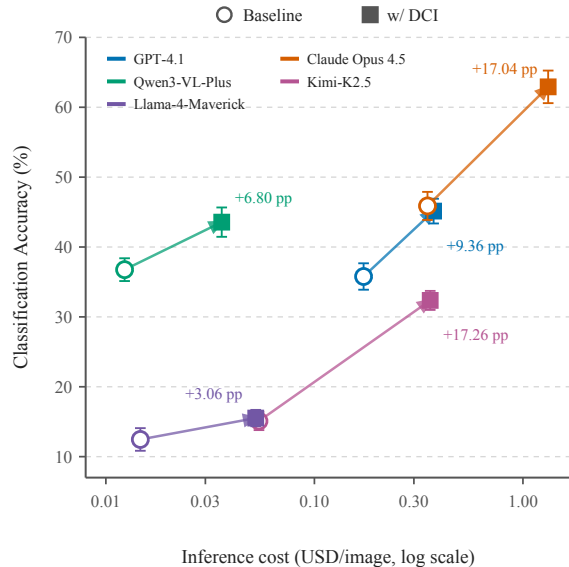
(b) API-served models: accuracy-cost trade-off
