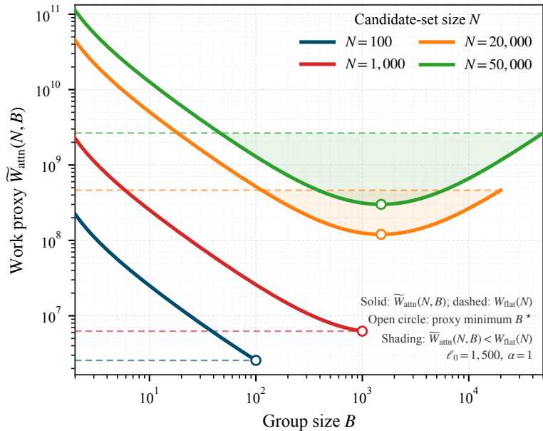
(b) Fixed- N scalability profiles
