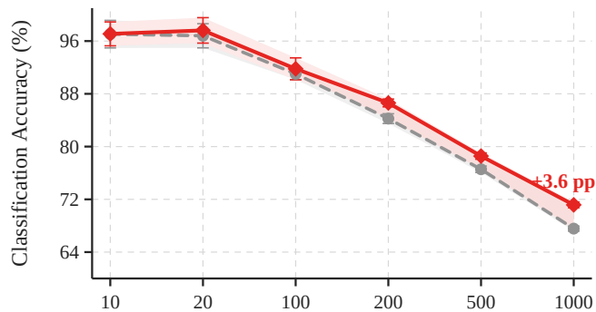
(c) Qwen3-VL-8B-Instruct
