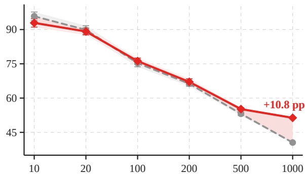
(b) Qwen3-VL-2B-Instruct
