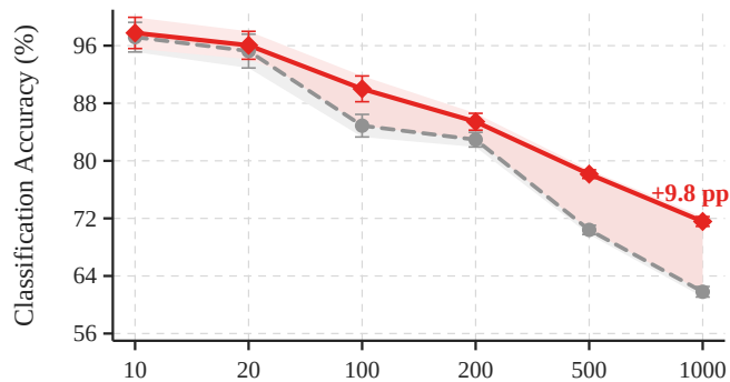
(a) Qwen2.5-VL-7B-Instruct
