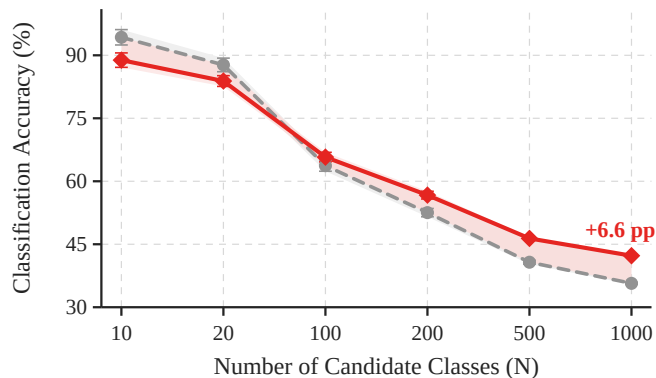
(e) Kimi-VL-A3B-Instruct
