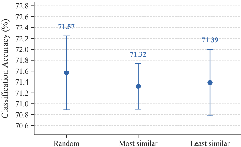
(a) Qwen2.5-VL-7B-Instruct
