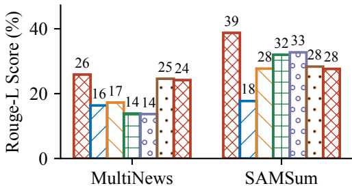
% LongBench Summarization
