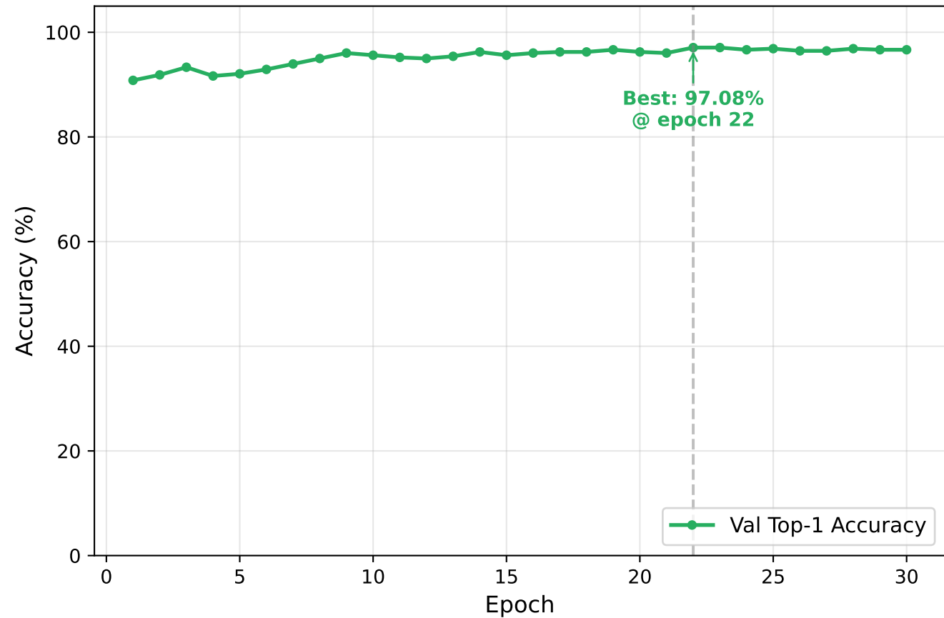
Validation Accuracy
