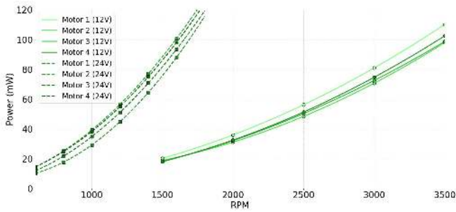
Fig. 7. Comparative power-RPM profiles for 12V and 24V DC motors under 470\ \Omega resistive load. Solid lines represent 12V motors (operating range 1500–3500 RPM), while dashed lines represent 24V motors (operating range 600–1600 RPM). The 24V motors achieve equivalent power output at approximately half the RPM, reducing the required gear amplification and associated mechanical complexity. Data points (markers) represent actual measurements.
