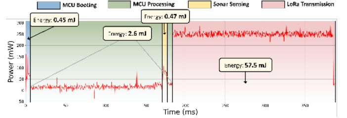
Fig. 5. Power consumption waveform of the Cleanify sensor node showing distinct phases: MCU boot-up, MCU processing, ultrasonic sensing, and LoRa transmission during a complete sensing and data transmission cycle.
