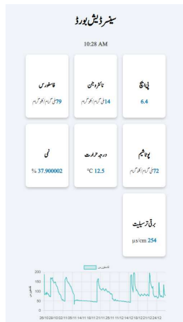
Fig. 9: Dashboard.
