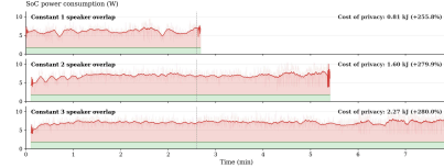
Fig. 11. Measured SoC power consumption under sustained one-, two-, and three-speaker workloads.
