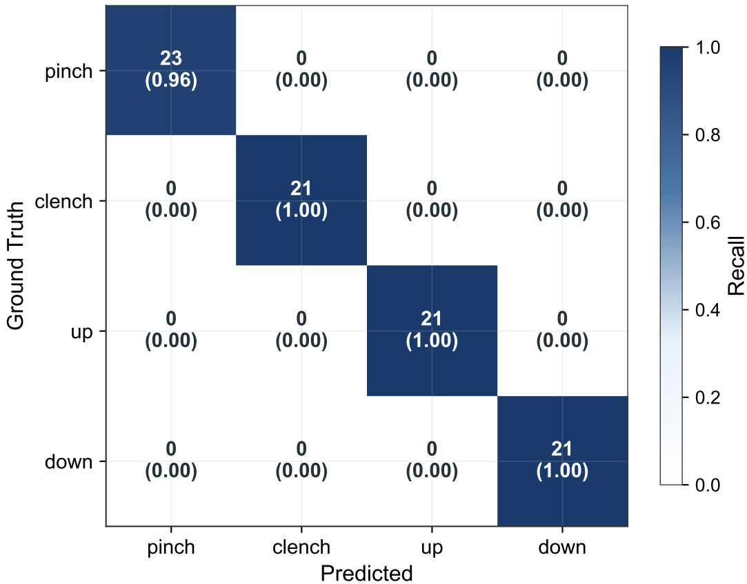
QEMU Confusion Matrix
