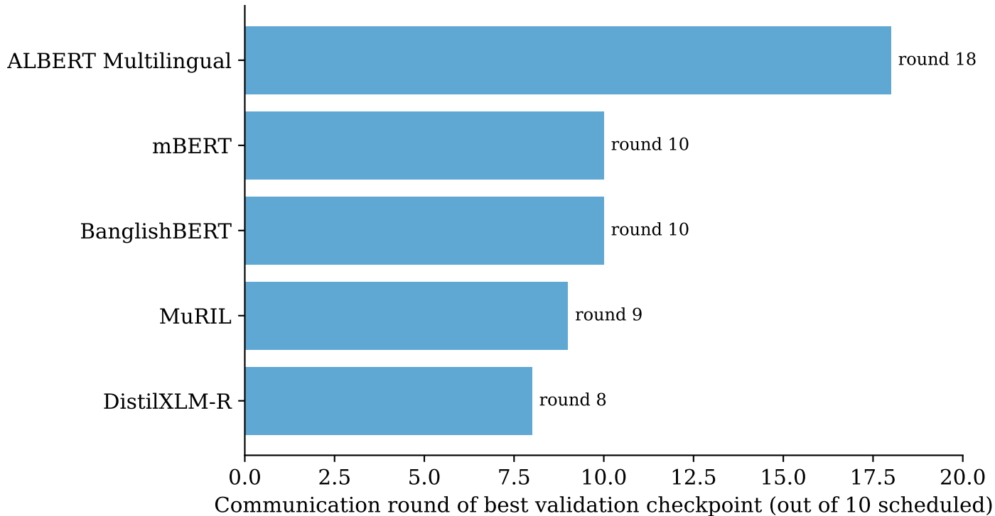
Federated Convergence Speed by Backbone (lower = converged faster to its best checkpoint)
