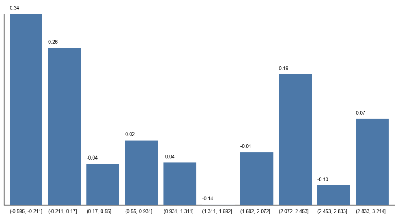
Model diagnostic residual pattern, Kyrgyzstan
