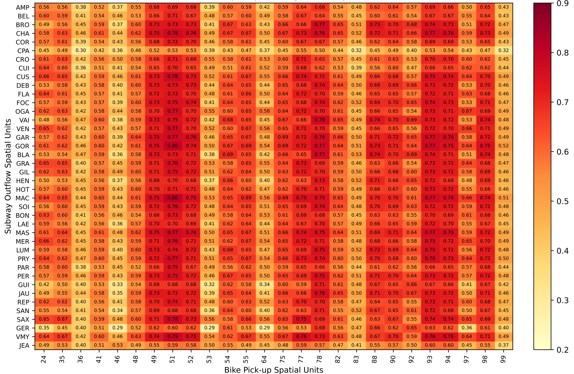
Lag: 15min - Correlation between Subway Outflow and lagged Bike Pick-up time-series - Lyon. Does Bike Pick-up help Subway Outflow prediction?
