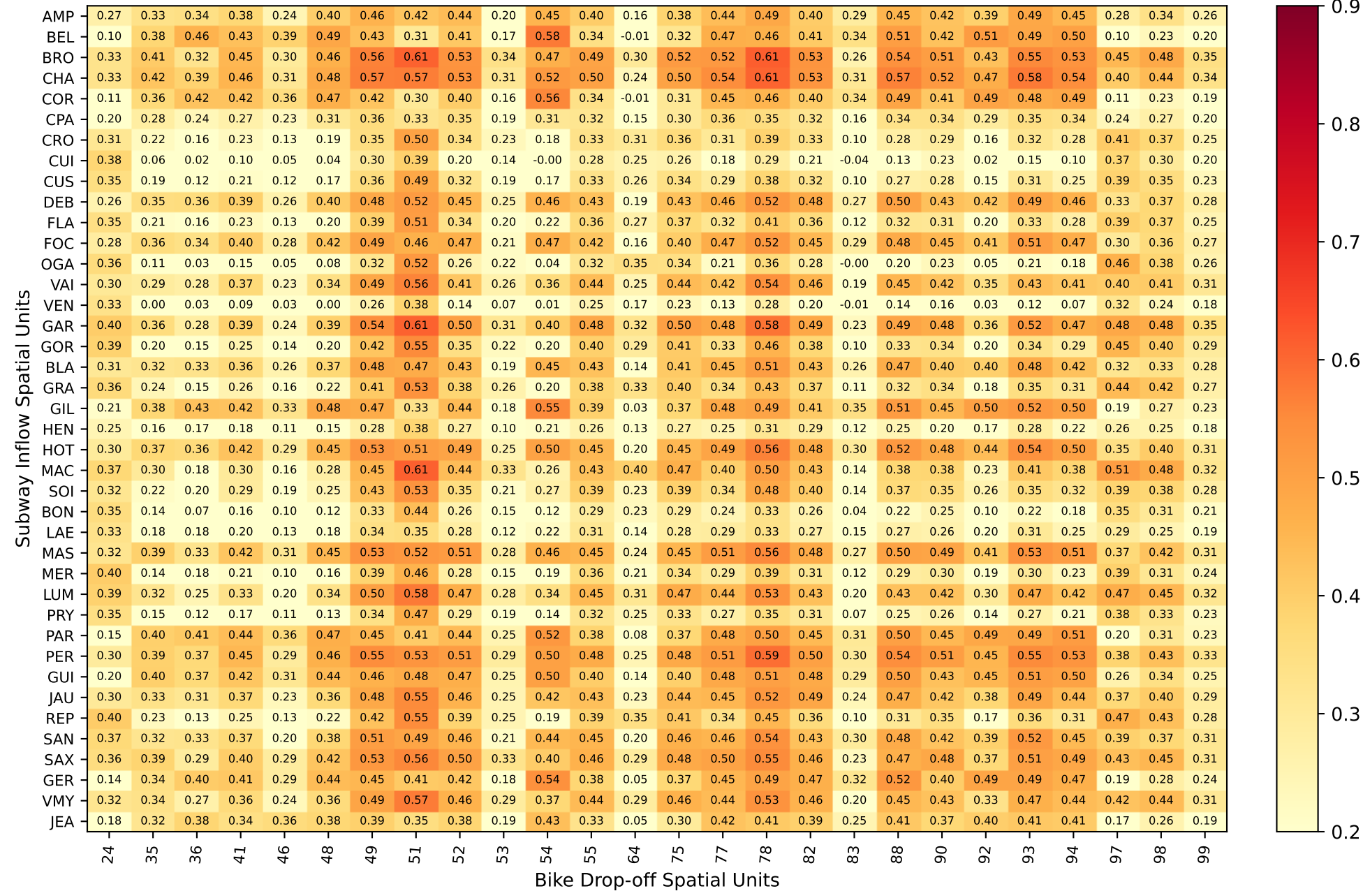
Lag: 15min - Correlation between Subway Inflow and lagged Bike Drop-off time-series - Lyon. Does Bike Drop-off help Subway Inflow prediction?
