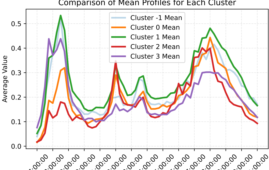
Comparison of Mean Profiles for Each Cluster
