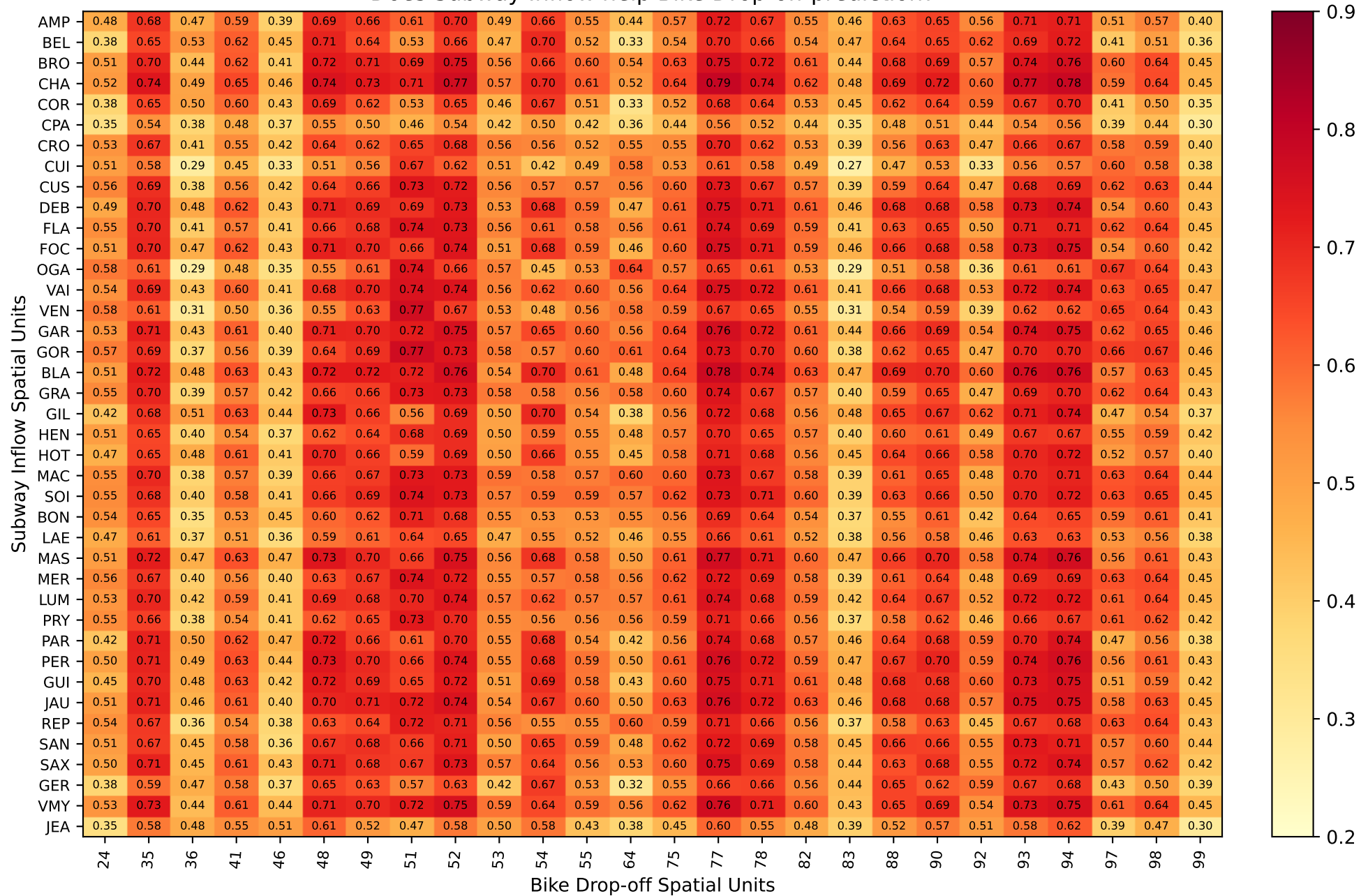
Lag: -2 - Correlation between Subway Inflow and lagged Bike Drop-off time-series - Lyon. Does Subway Inflow help Bike Drop-off prediction?
