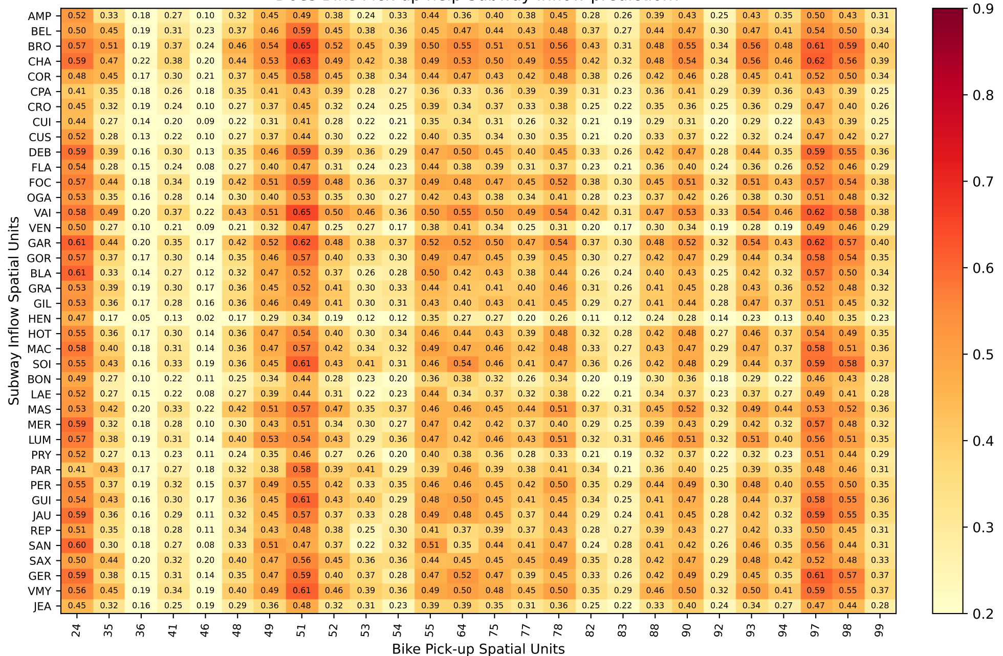
Lag: 15min - Correlation between Subway Inflow and lagged Bike Pick-up time-series - Lyon. Does Bike Pick-up help Subway Inflow prediction?
