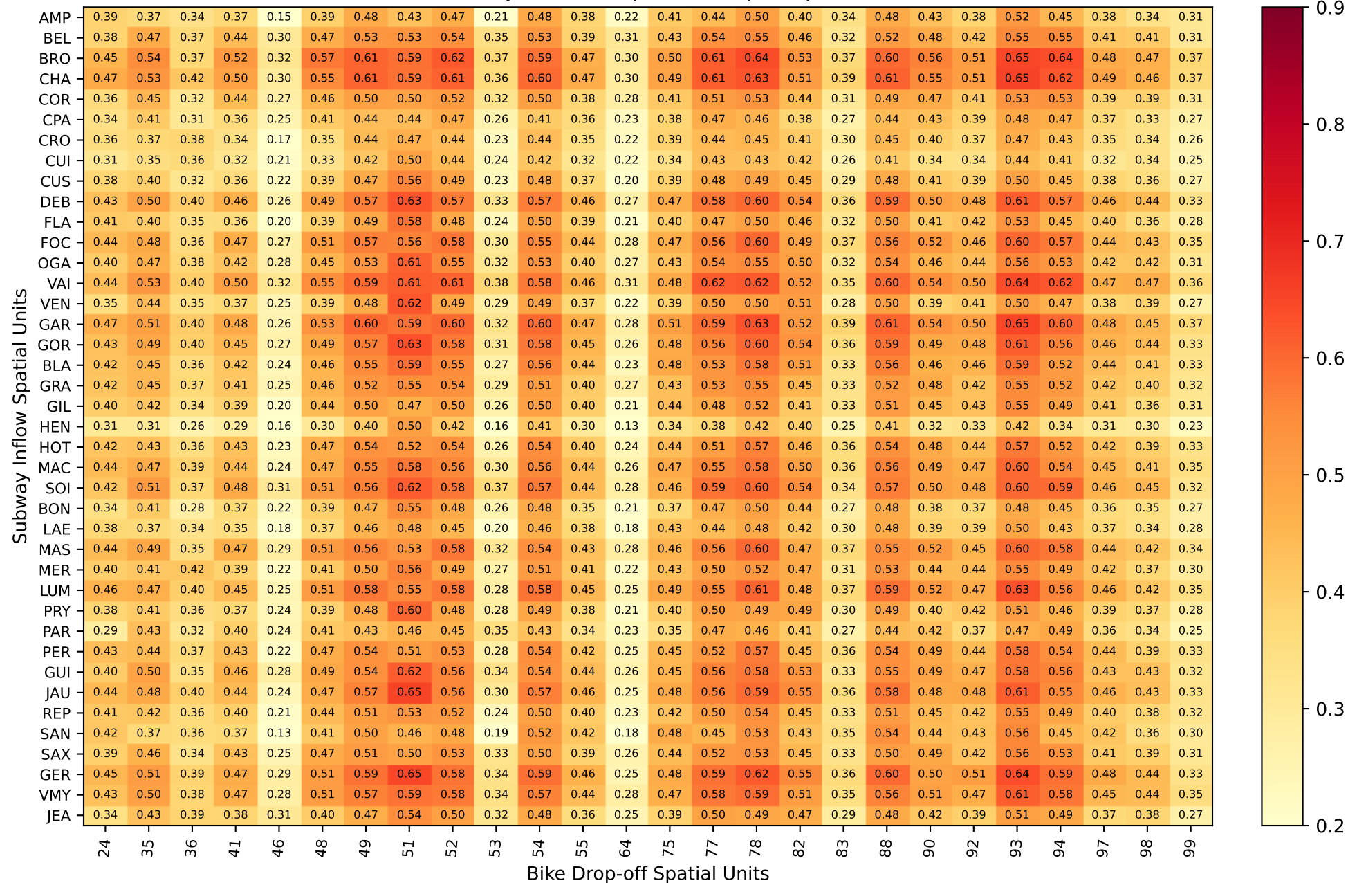
Lag: -15min - Correlation between Subway Inflow and lagged Bike Drop-off time-series - Lyon. Does Subway Inflow help Bike Drop-off prediction?
