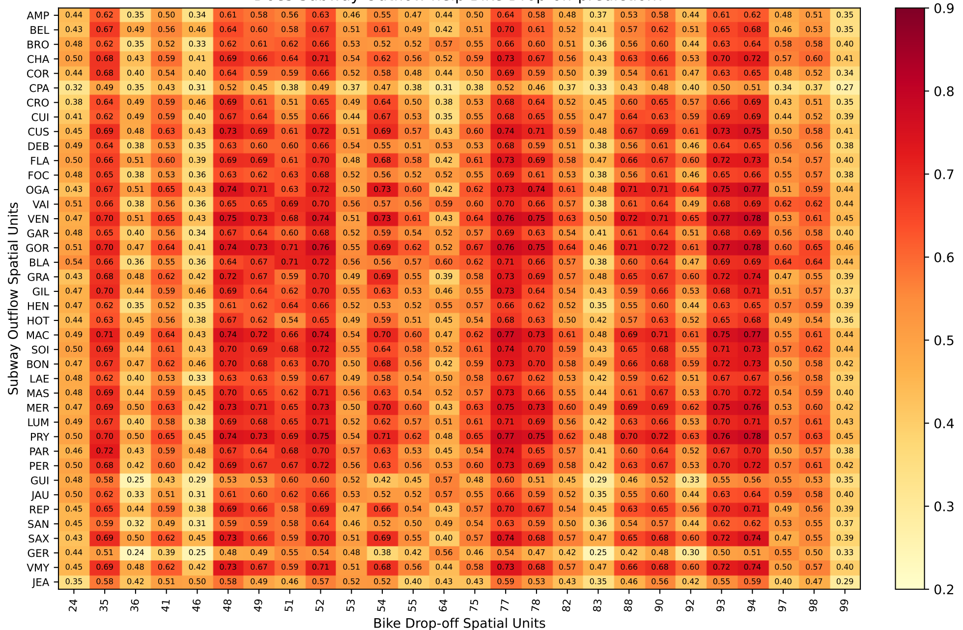
Lag: -2 - Correlation between Subway Outflow and lagged Bike Drop-off time-series - Lyon. Does Subway Outflow help Bike Drop-off prediction?
