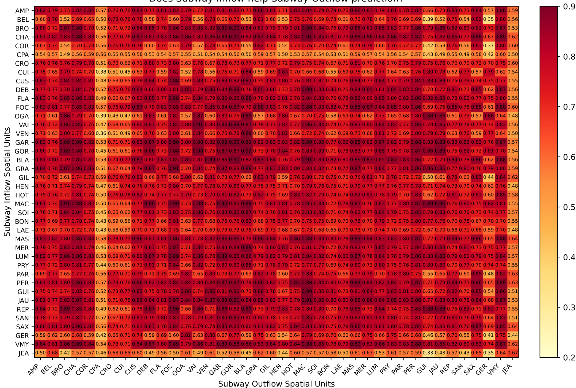
Lag: -15min - Correlation between Subway Inflow and lagged Subway Outflow time-series - Lyon. Does Subway Inflow help Subway Outflow prediction?
