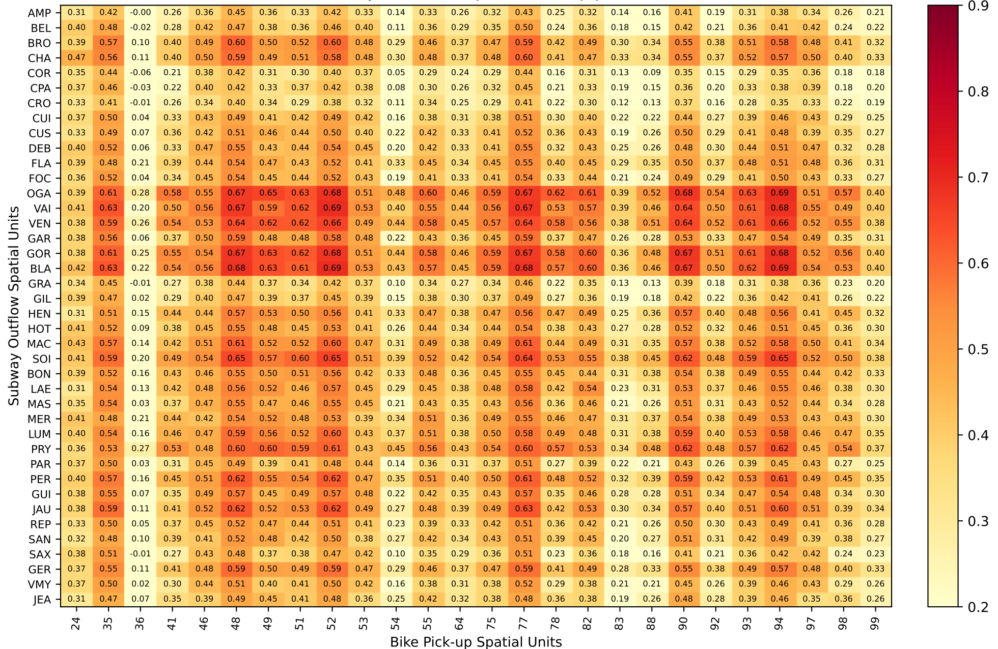
Lag: -15min - Correlation between Subway Outflow and lagged Bike Pick-up time-series - Lyon. Does Subway Outflow help Bike Pick-up prediction?
