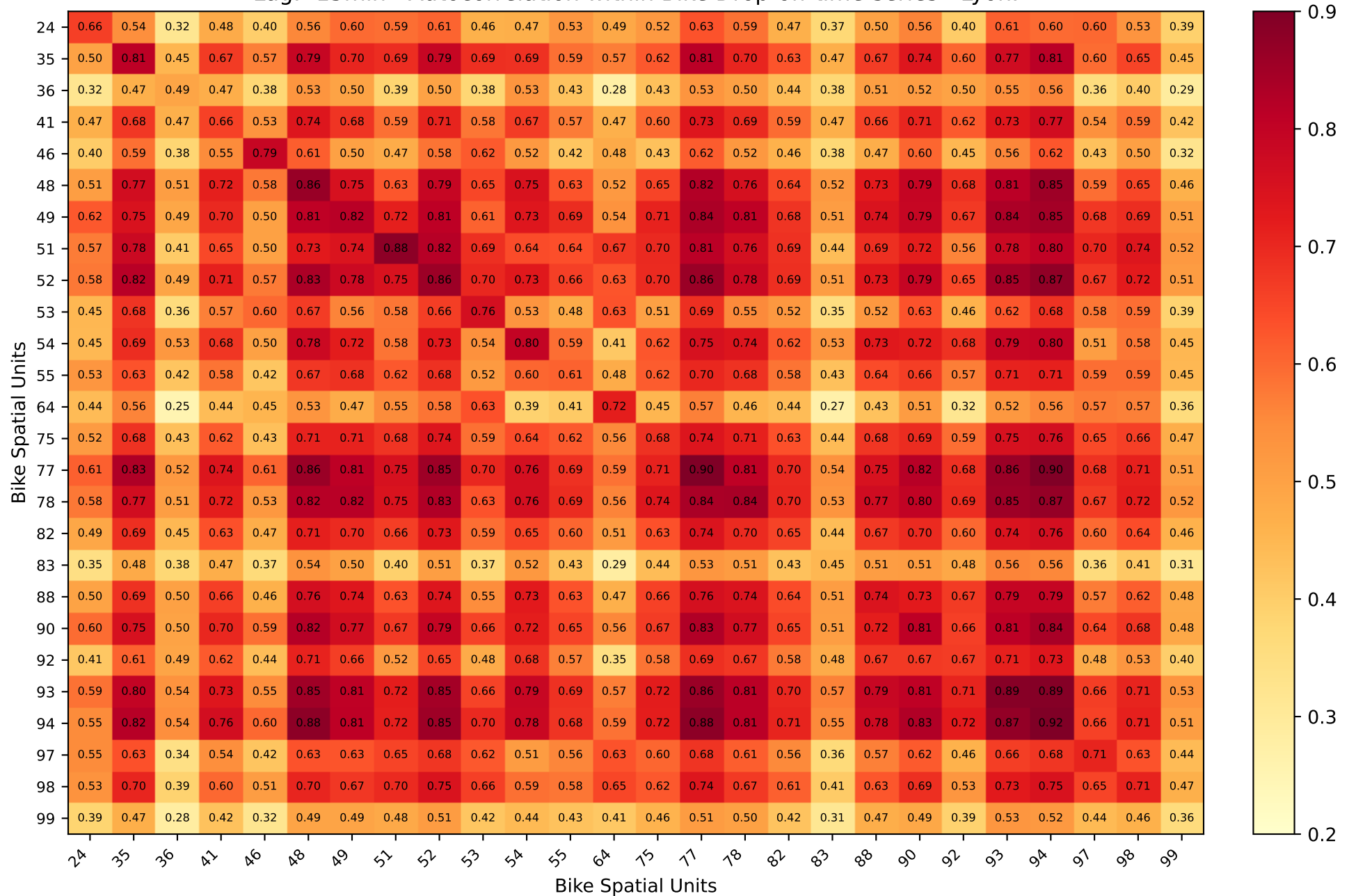
Lag: -15min - Autocorrelation within Bike Drop-off time-series - Lyon.
