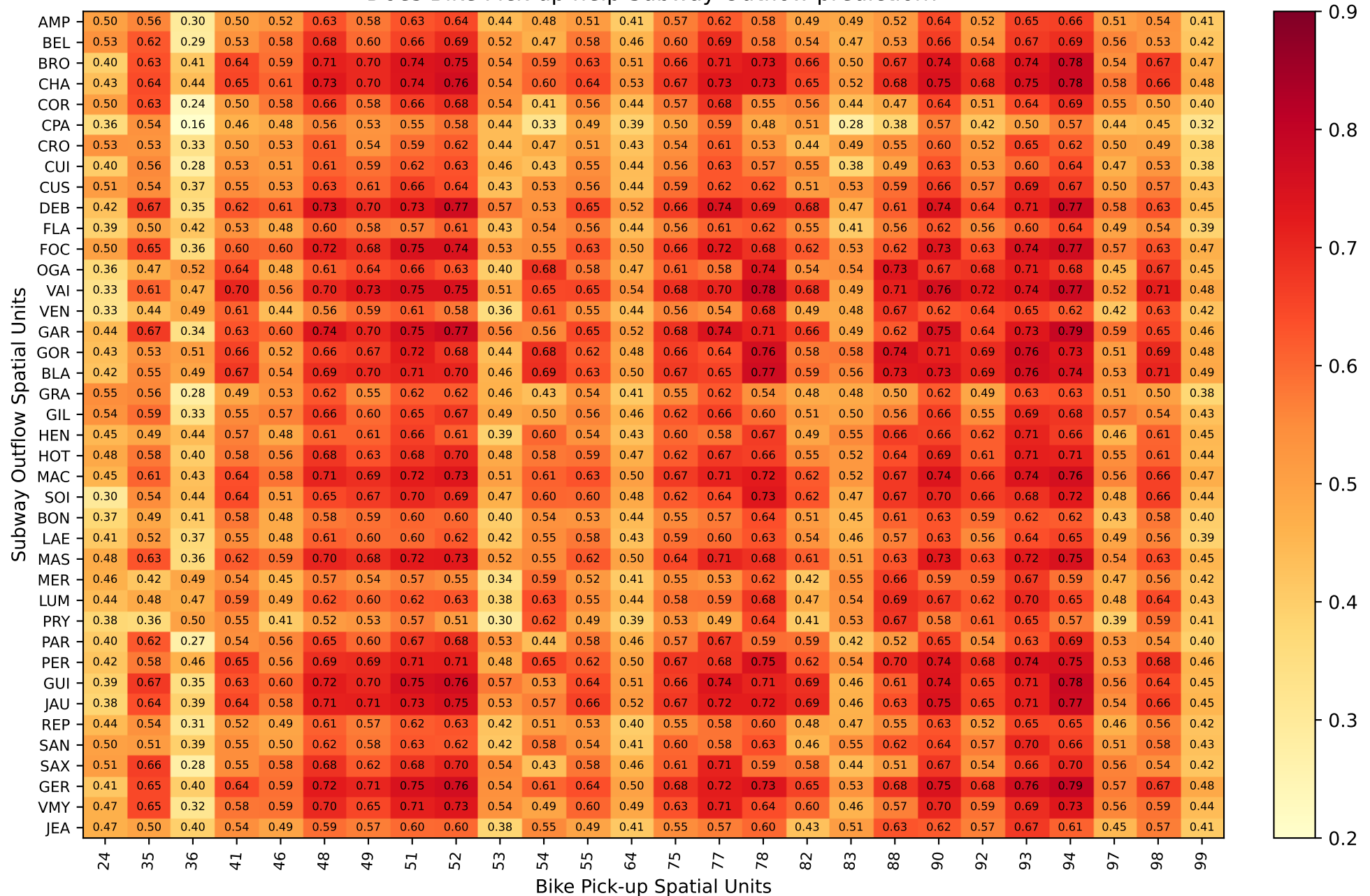
Lag: 15min - Correlation between Subway Outflow and lagged Bike Pick-up time-series - Lyon. Does Bike Pick-up help Subway Outflow prediction?
