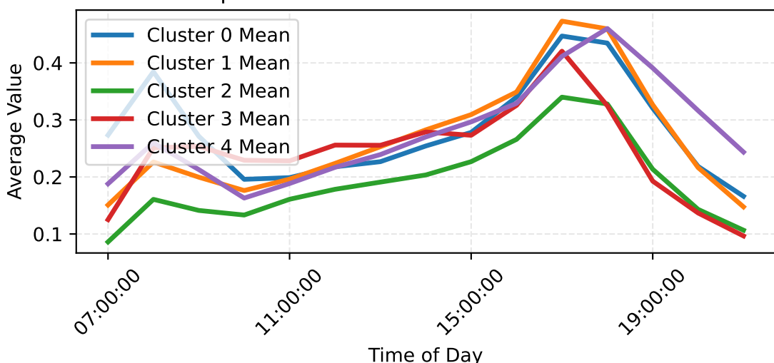
Comparison of Mean Profiles for Each Cluster
