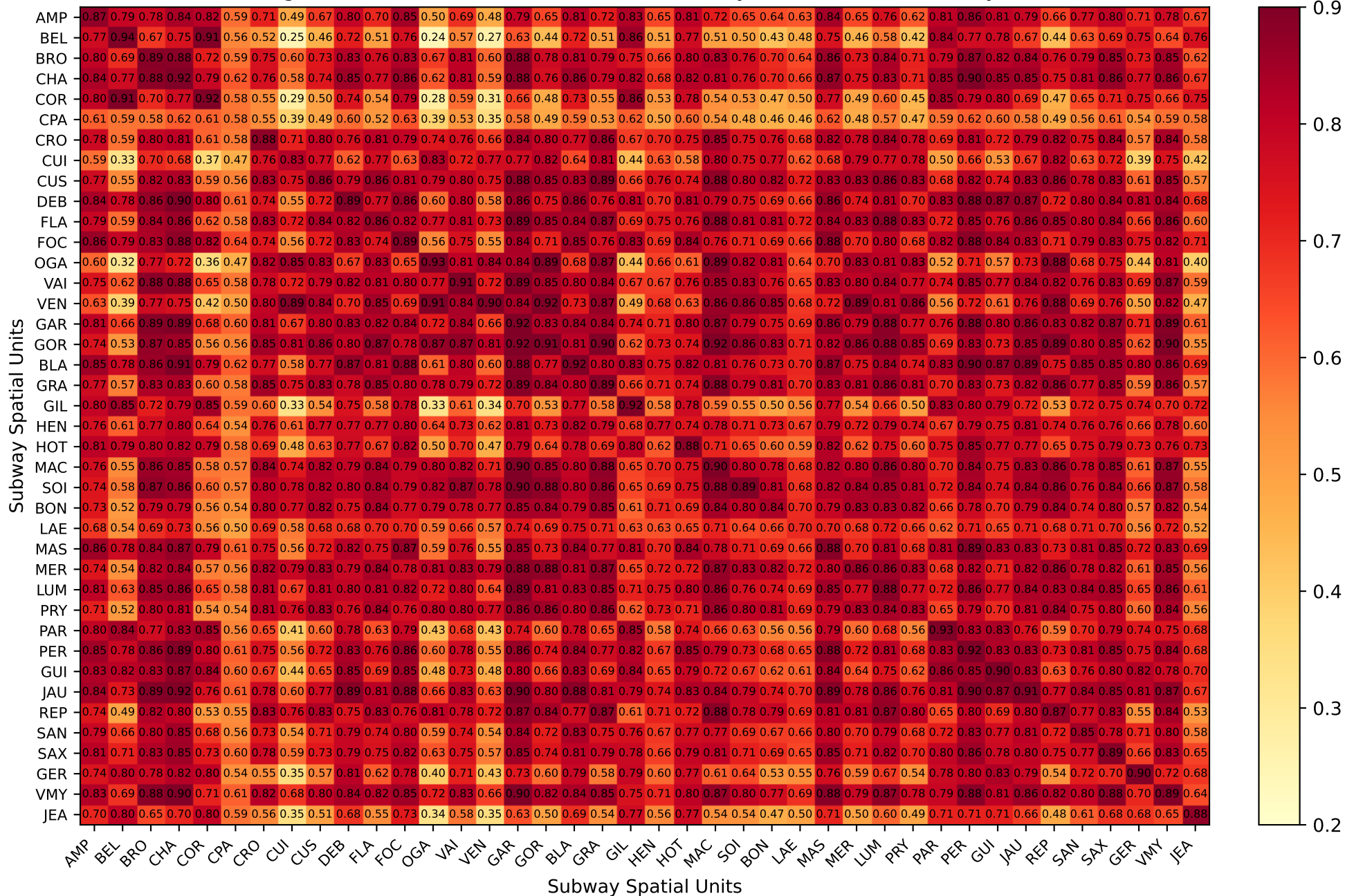
Lag: -15min - Autocorrelation within Subway Inflow time-series - Lyon.
