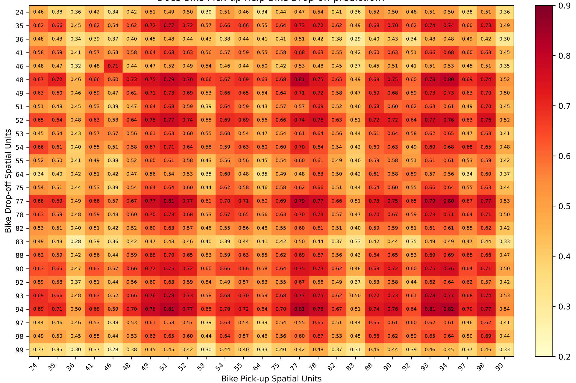
Lag: 3 - Correlation between Bike Drop-off and lagged Bike Pick-up time-series - Lyon. Does Bike Pick-up help Bike Drop-off prediction?
