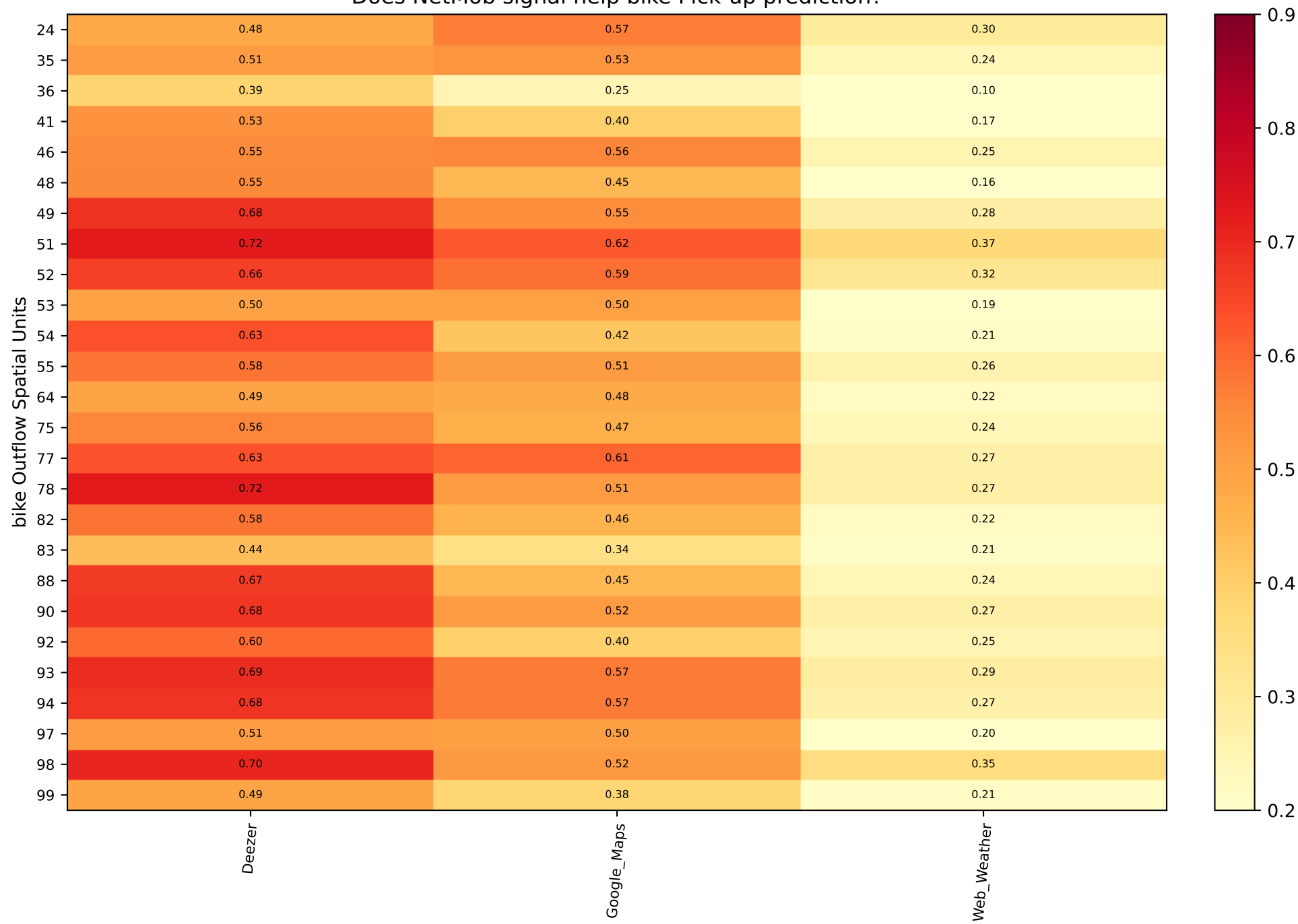
Lag: -15min - Correlation between bike Outflow and lagged NetMob time-series - Lyon. Does NetMob signal help bike Pick-up prediction?
