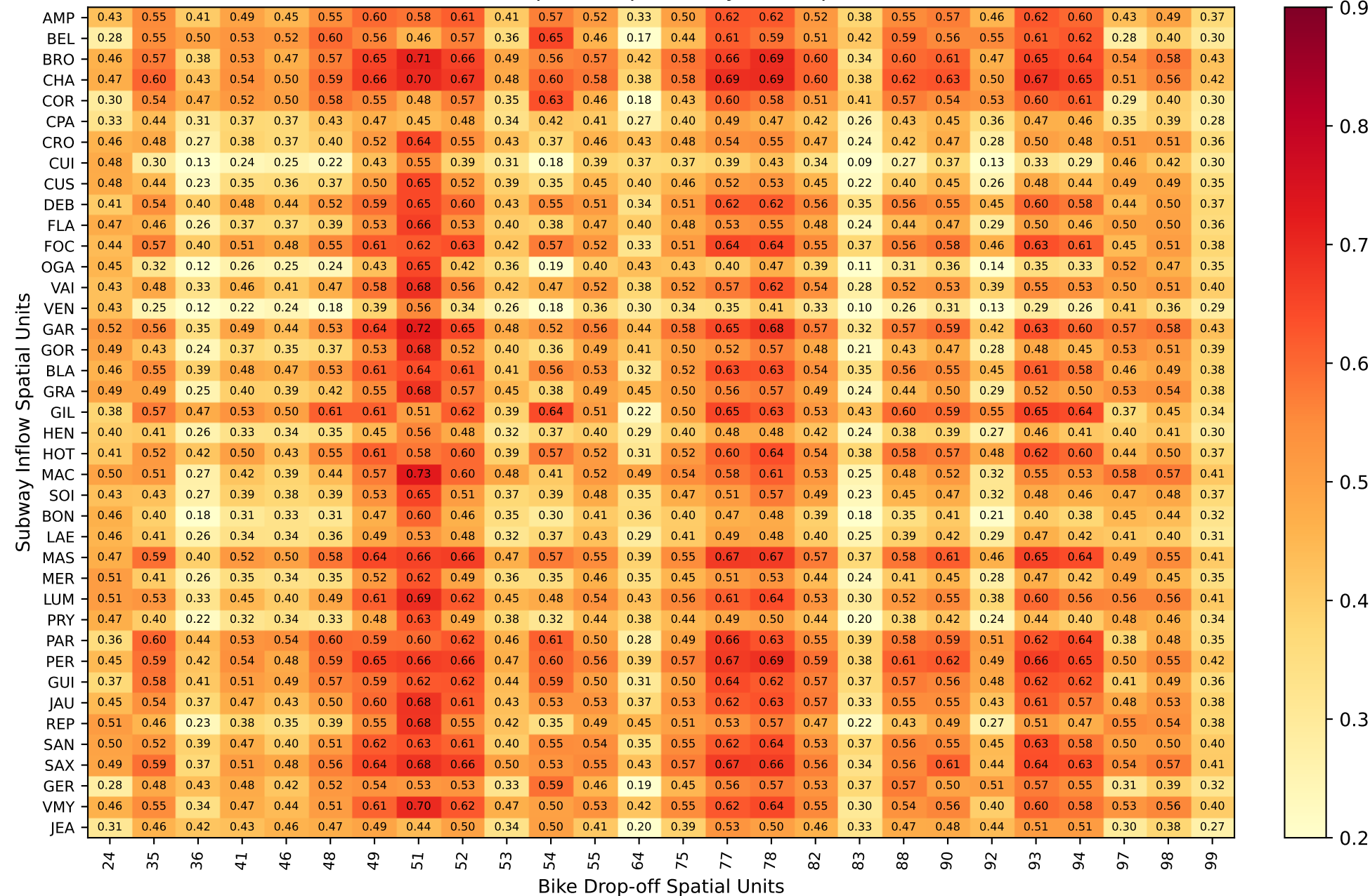
Lag: 15min - Correlation between Subway Inflow and lagged Bike Drop-off time-series - Lyon. Does Bike Drop-off help Subway Inflow prediction?
