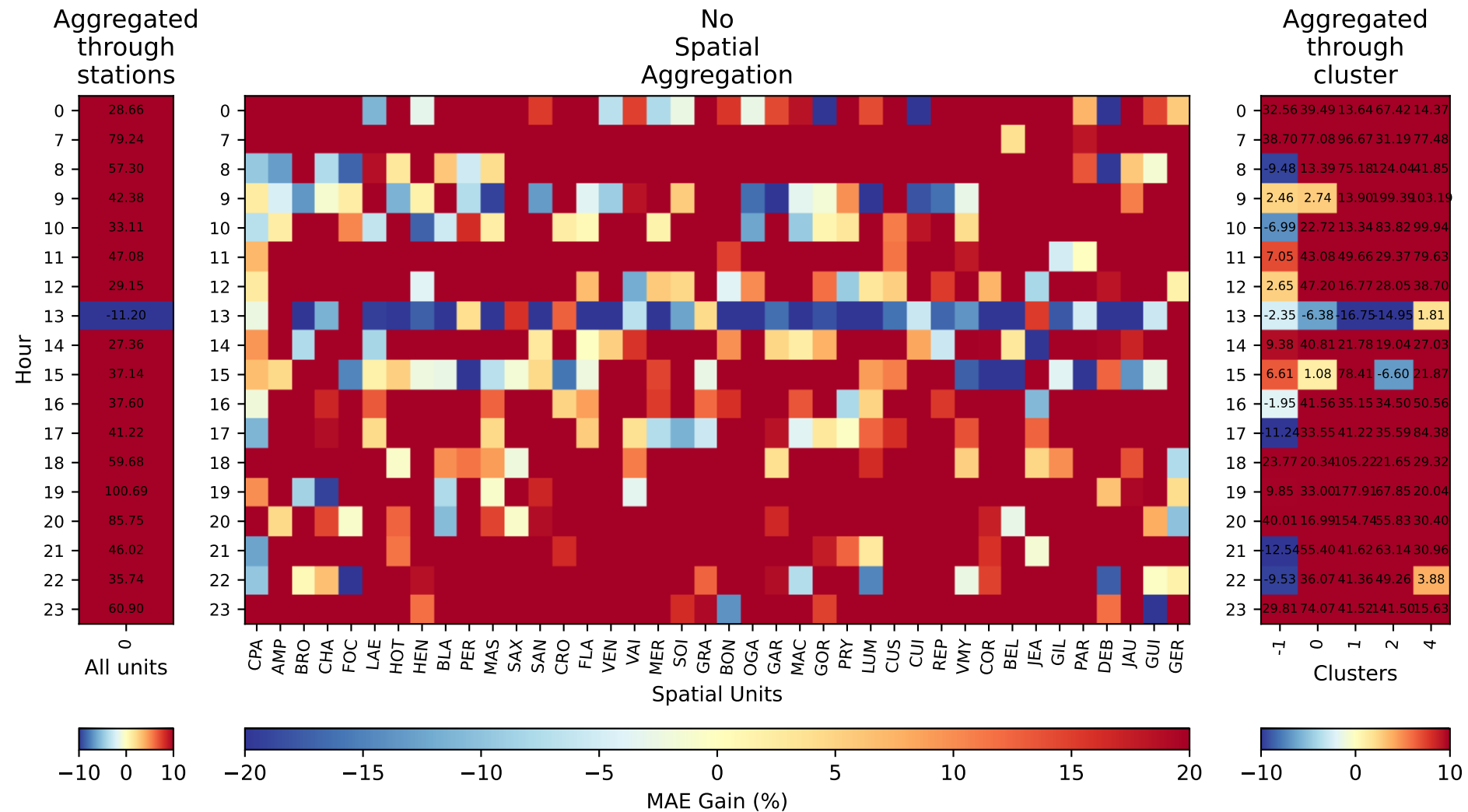
Average MAE Gain(%) per Hour on Business Day
