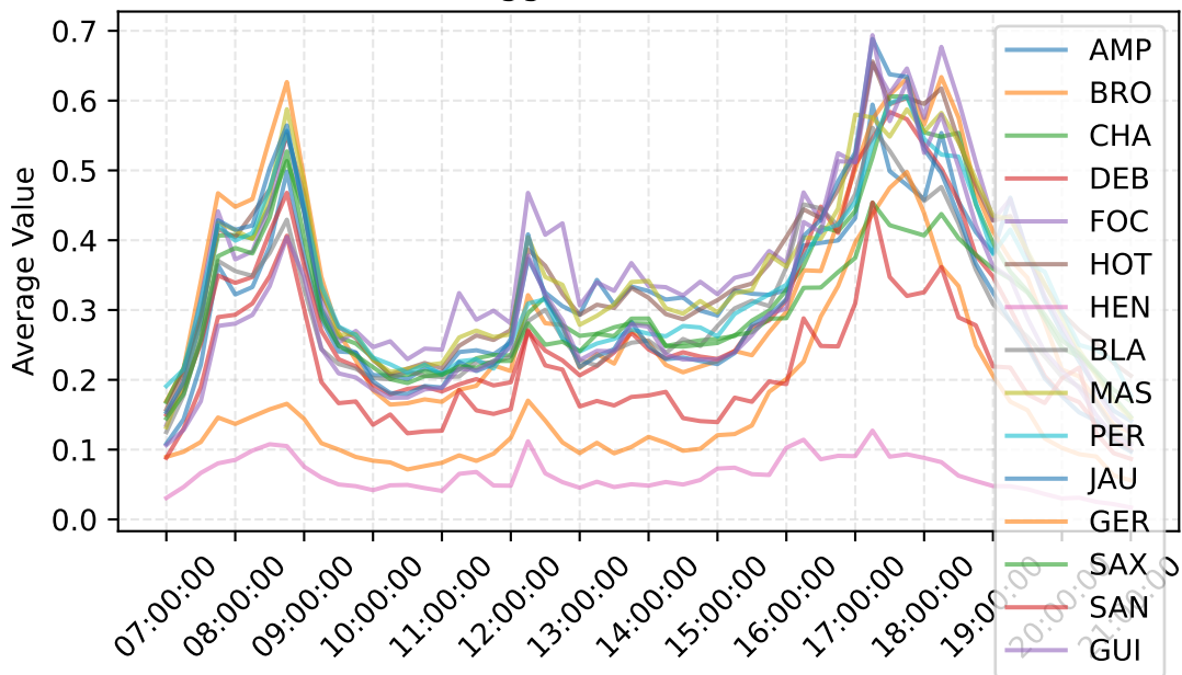
Cluster 0 (agglomerative-based Profiles)
