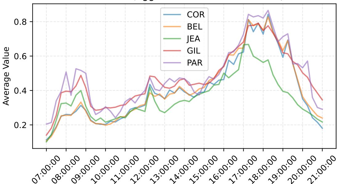
Cluster 2 (agglomerative-based Profiles)
