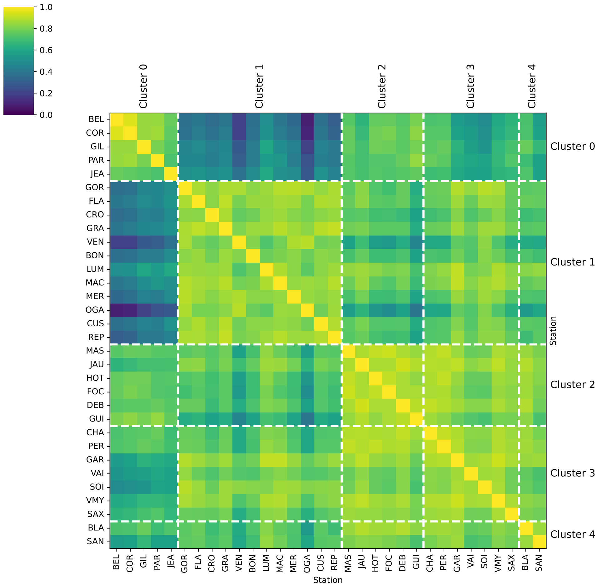
Correlation Matrix Heatmap (Ordered by Cluster)
