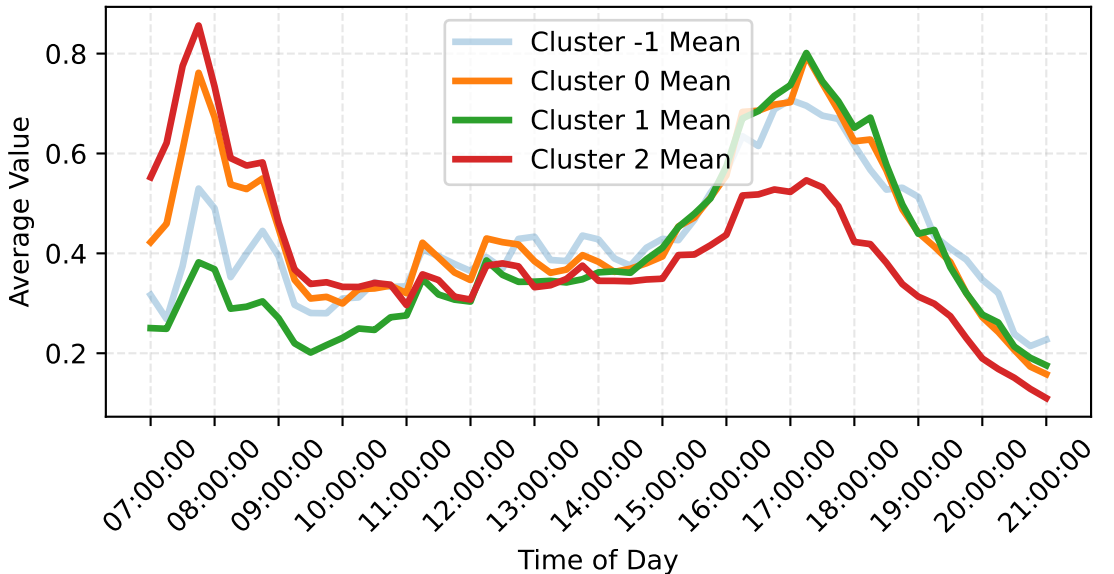
Comparison of Mean Profiles for Each Cluster
