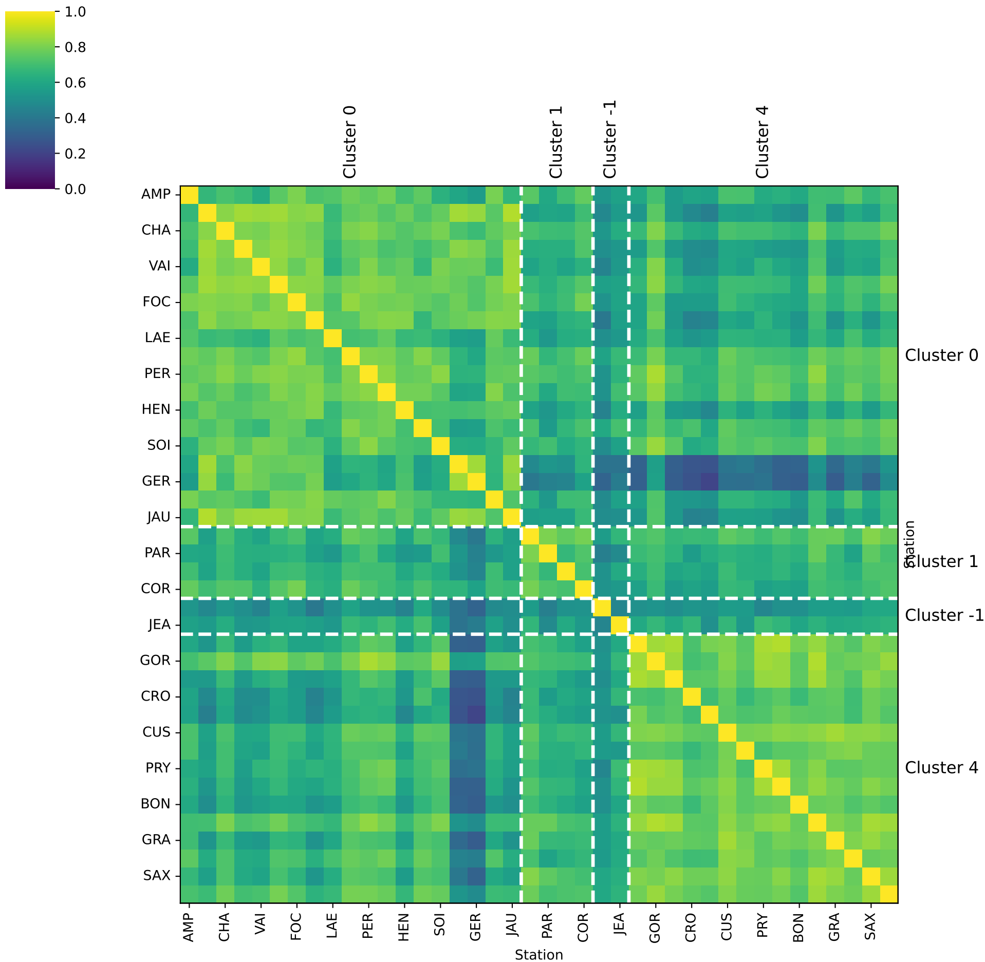
Correlation Matrix Heatmap (Ordered by Cluster)
