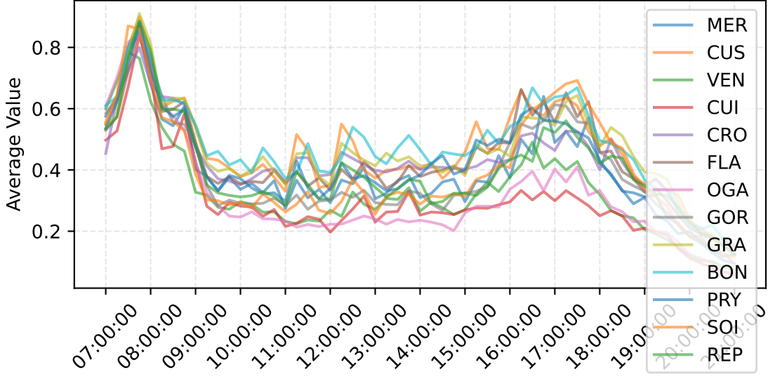
Cluster 2 (agglomerative-based Profiles)
