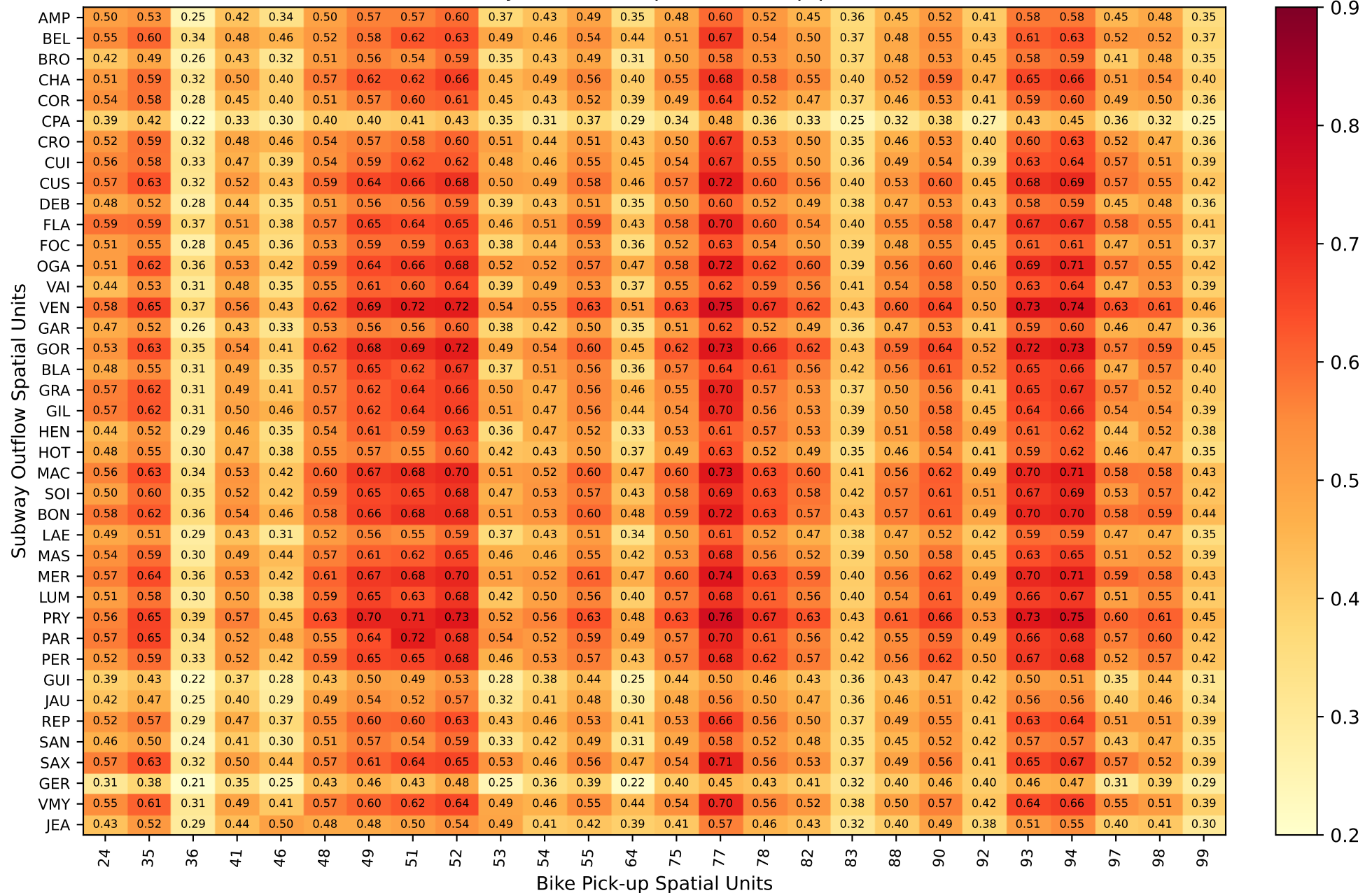
Lag: -3 - Correlation between Subway Outflow and lagged Bike Pick-up time-series - Lyon. Does Subway Outflow help Bike Pick-up prediction?
