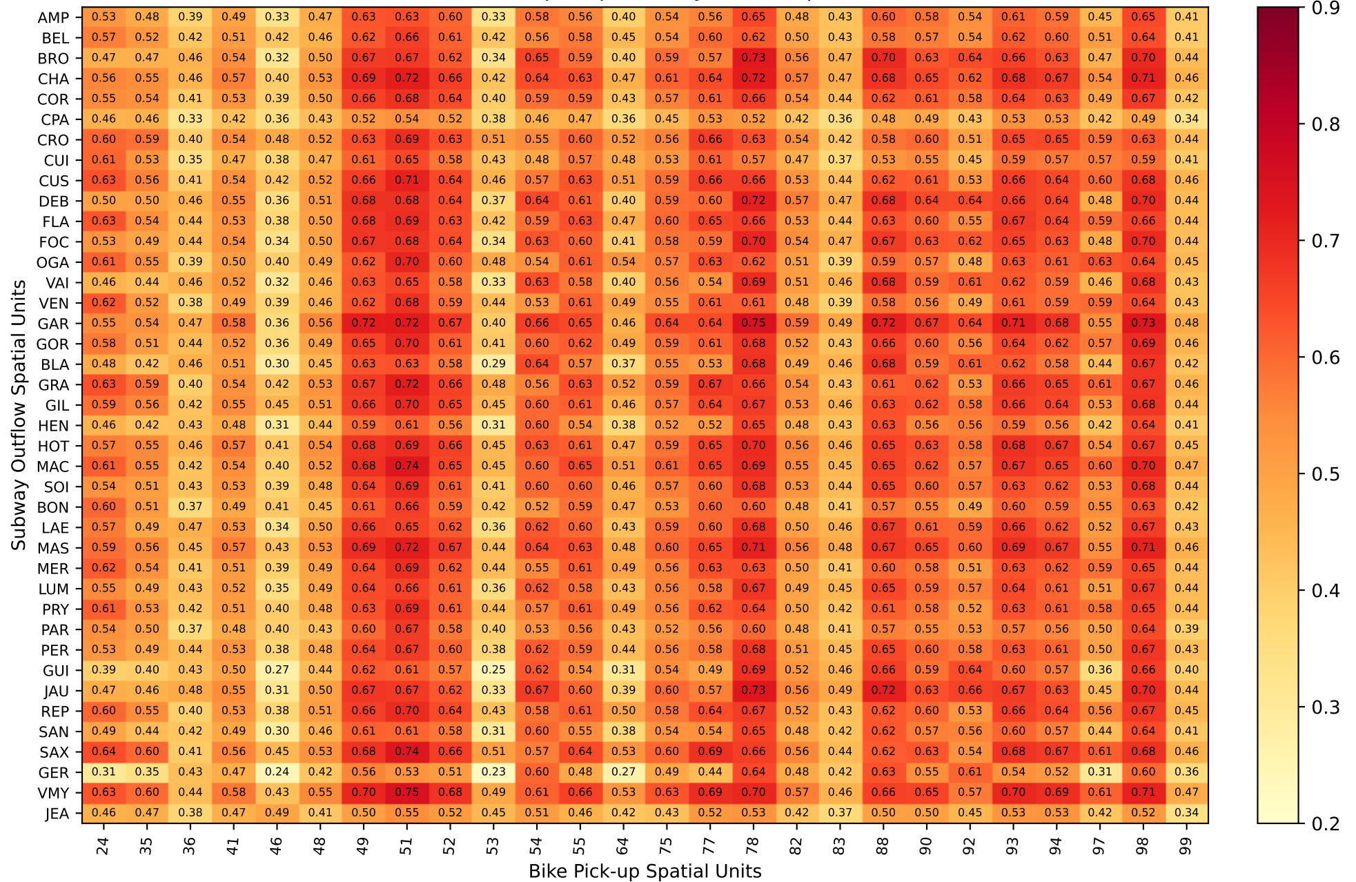
Does Bike Pick-up help Subway Outflow prediction?
