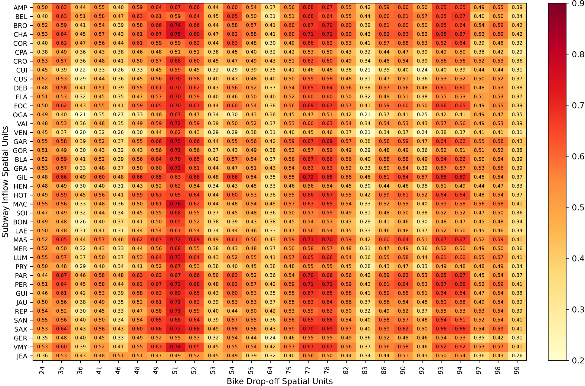
Does Bike Drop-off help Subway Inflow prediction?
