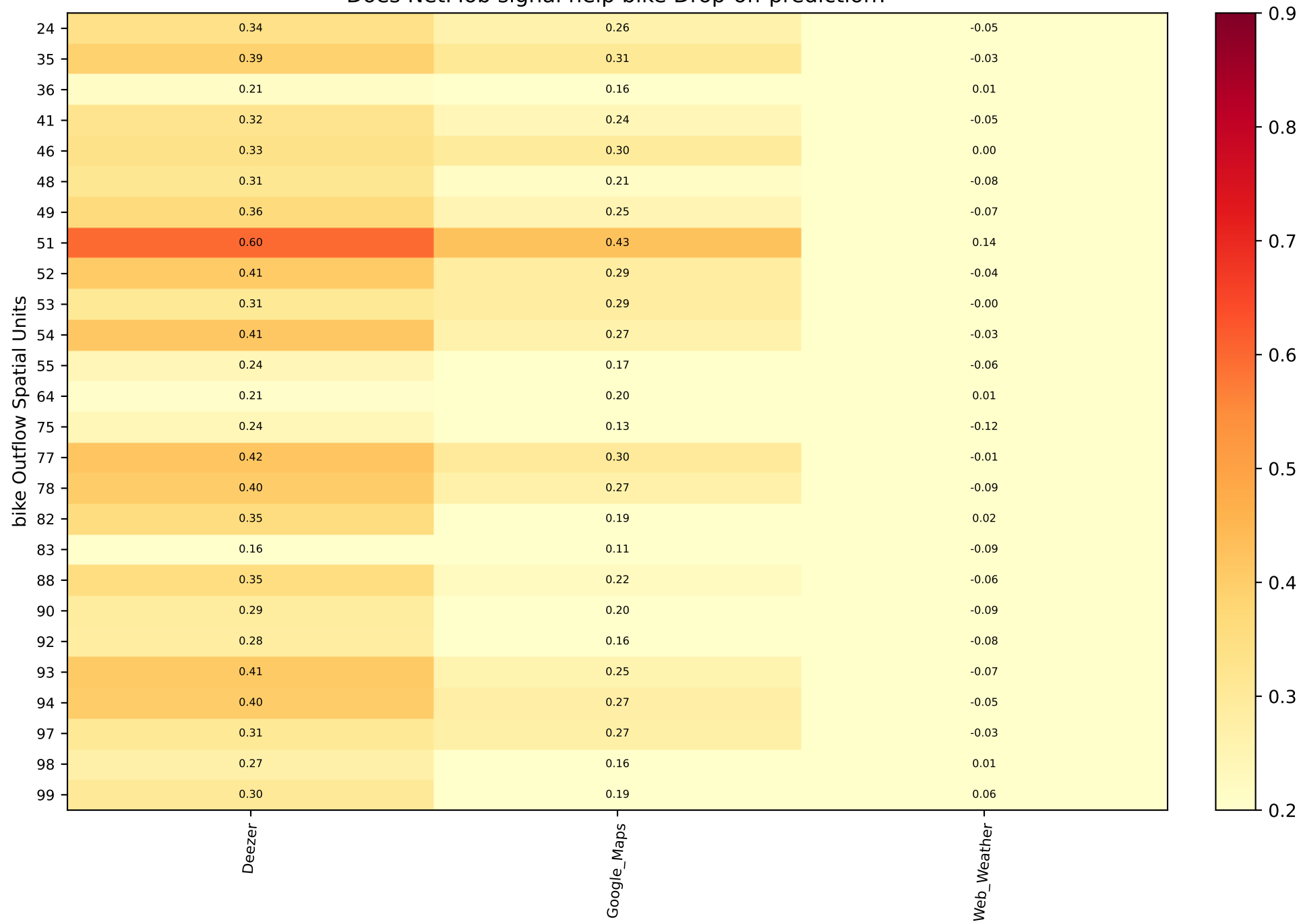
Lag: -15min - Correlation between bike Outflow and lagged NetMob time-series - Lyon. Does NetMob signal help bike Drop-off prediction?
