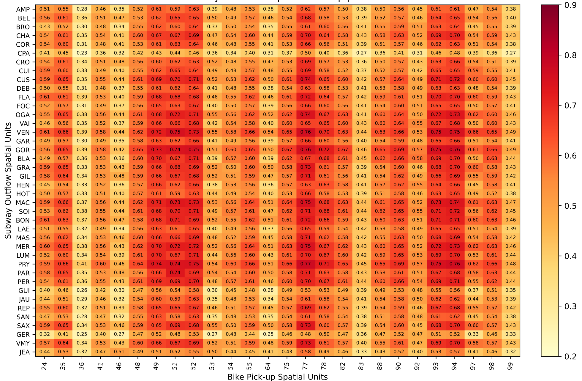
Lag: -2 - Correlation between Subway Outflow and lagged Bike Pick-up time-series - Lyon. Does Subway Outflow help Bike Pick-up prediction?
