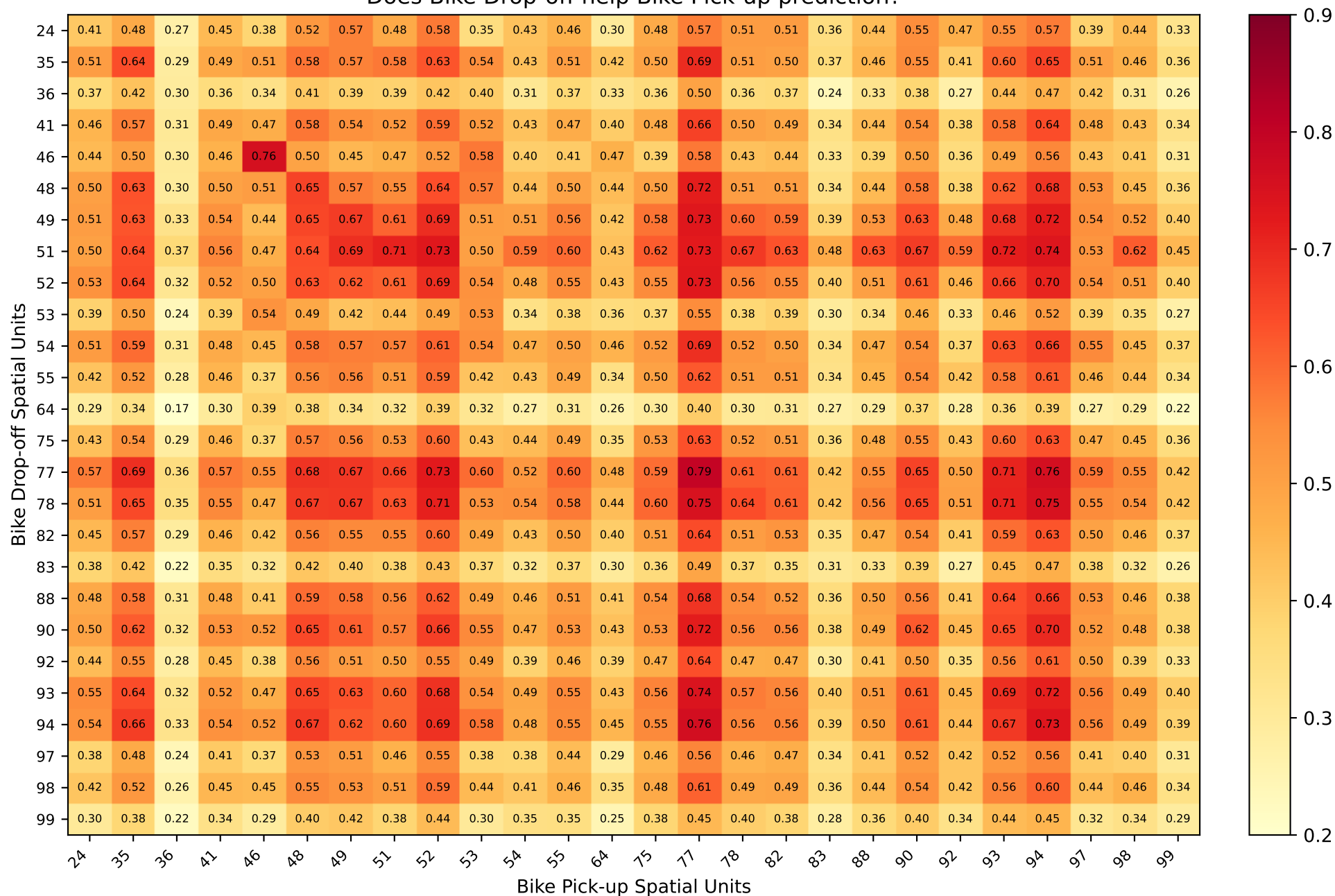
Lag: -45min - Correlation between Bike Drop-off and lagged Bike Pick-up time-series - Lyon. Does Bike Drop-off help Bike Pick-up prediction?
