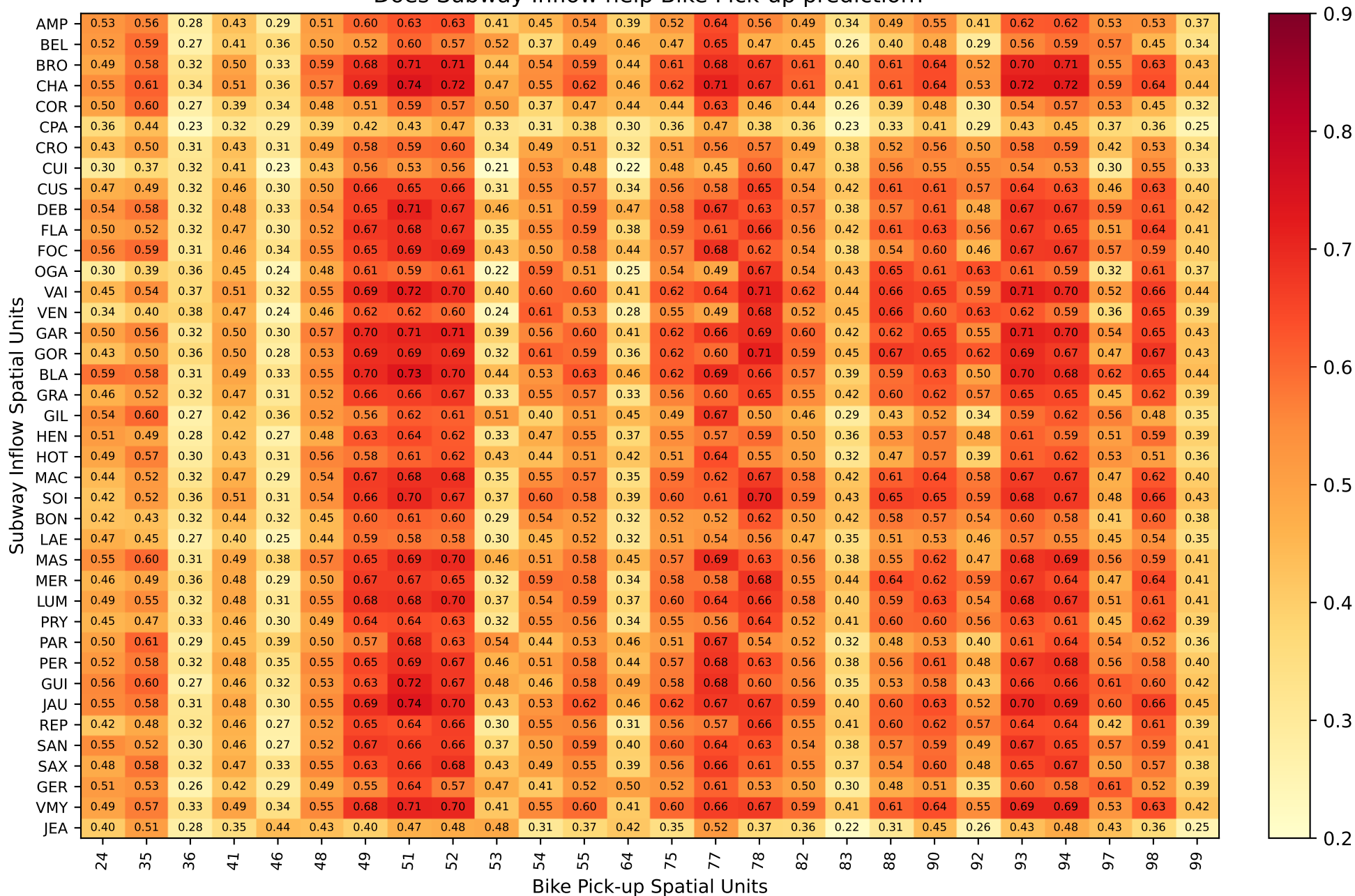
Lag: -15min - Correlation between Subway Inflow and lagged Bike Pick-up time-series - Lyon. Does Subway Inflow help Bike Pick-up prediction?
