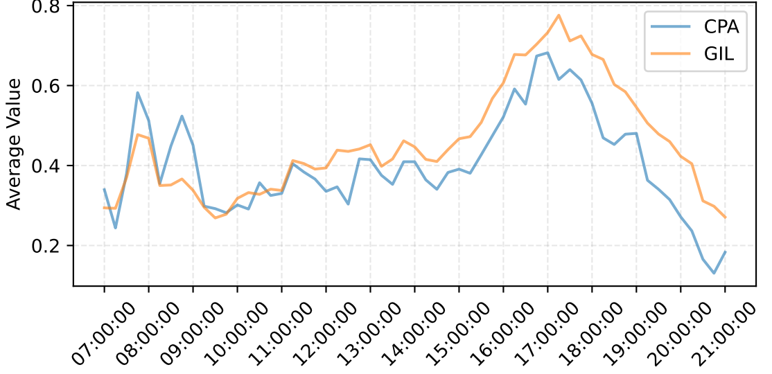
Cluster -1 (agglomerative-based Profiles)
