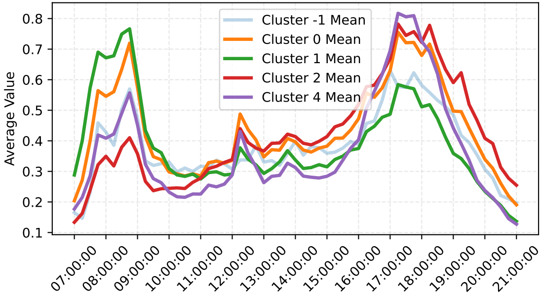
Comparison of Mean Profiles for Each Cluster
