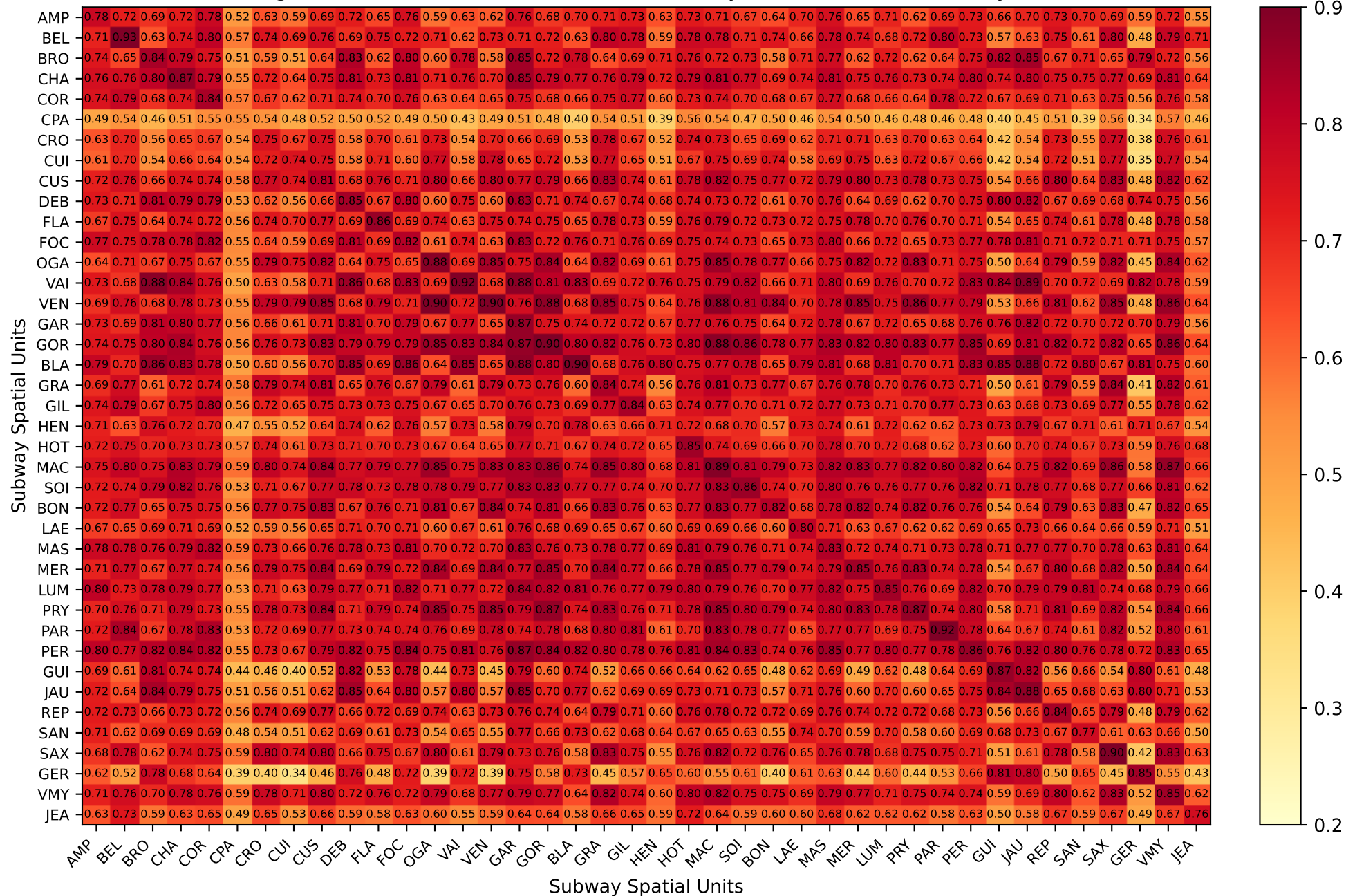
Lag: -15min - Autocorrelation within Subway Outflow time-series - Lyon.
