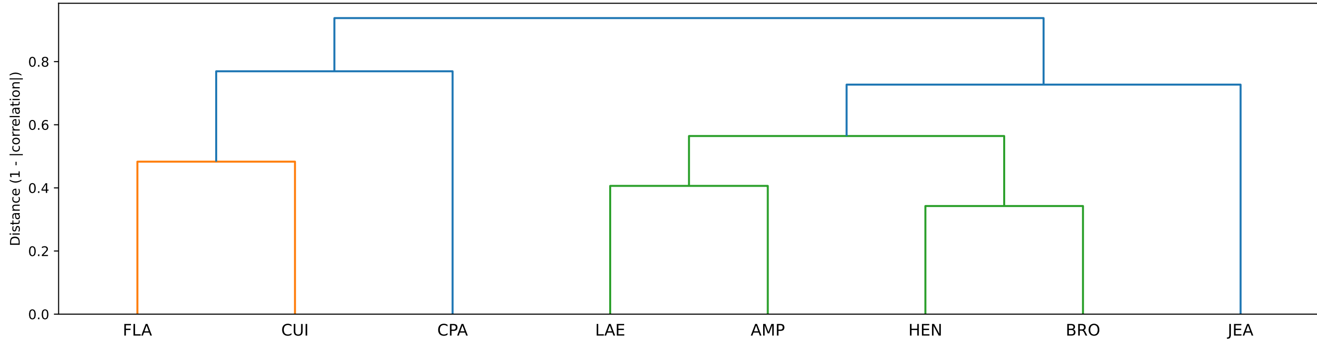
Dendrogram of Time Series
