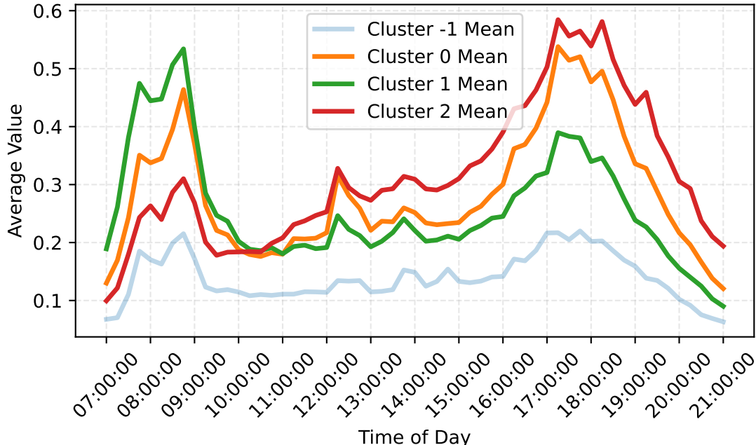
Comparison of Mean Profiles for Each Cluster
