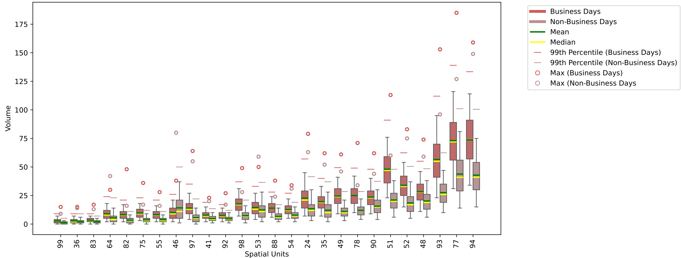
Boxplot of Volumes by Spatial Units and Evening Peak (4:30pm-7pm) period
