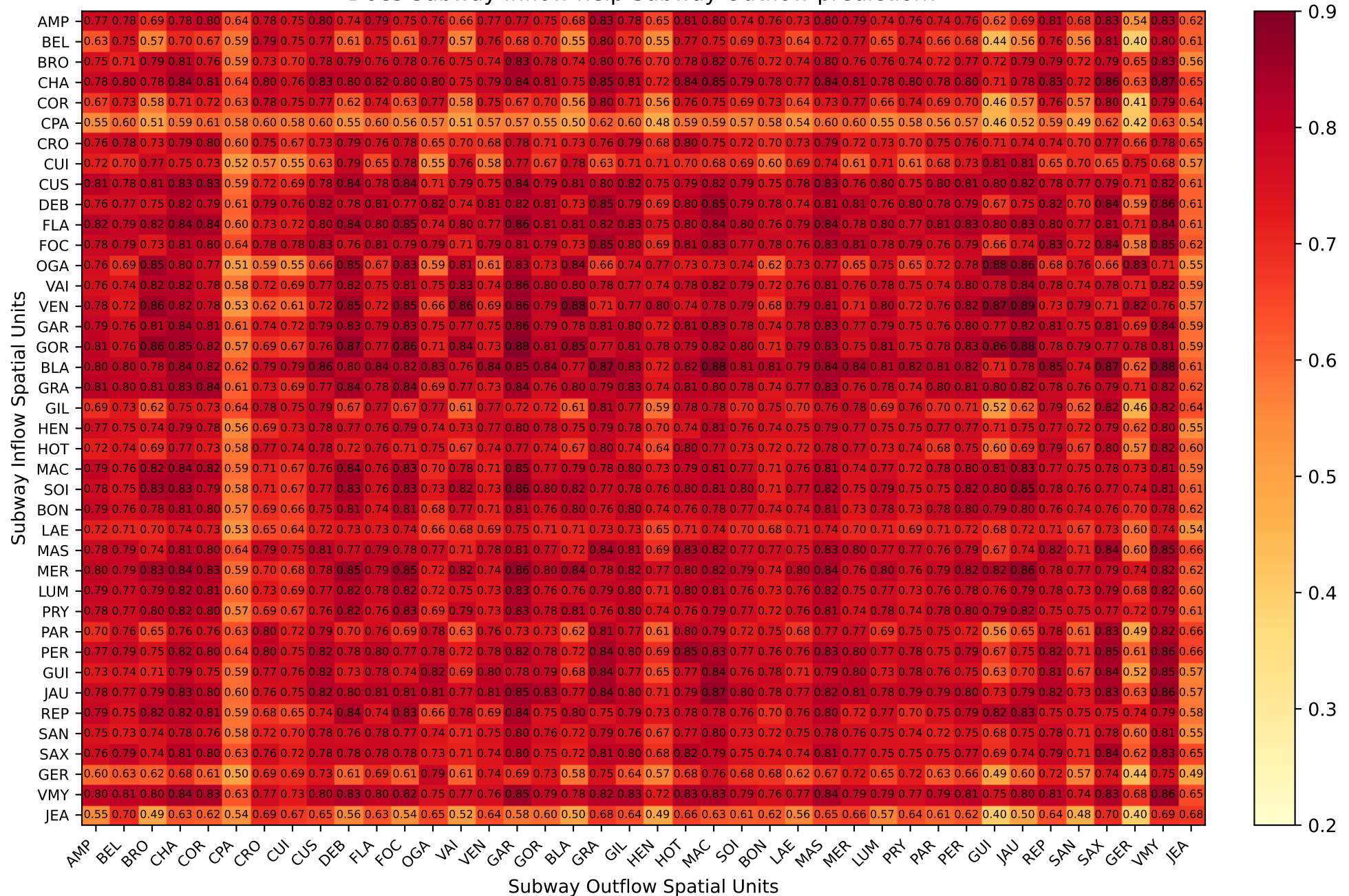
Lag: -45min - Correlation between Subway Inflow and lagged Subway Outflow time-series - Lyon. Does Subway Inflow help Subway Outflow prediction?
