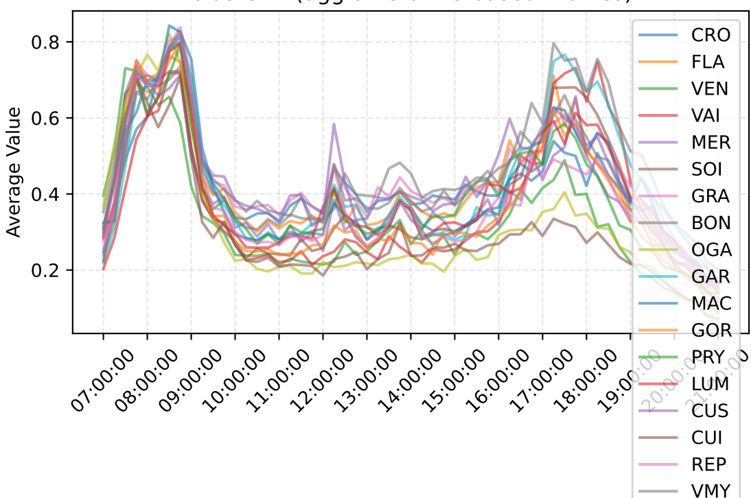
Cluster 2 (agglomerative-based Profiles)
