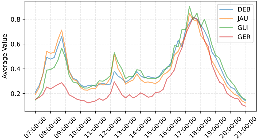
Cluster 4 (agglomerative-based Profiles)
