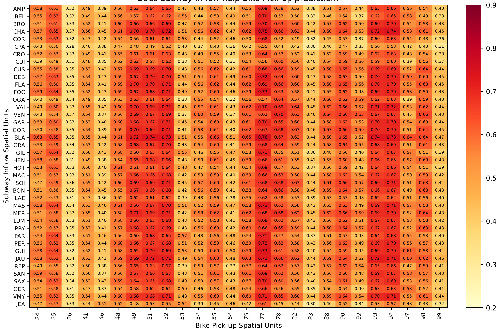
Lag: -3 - Correlation between Subway Inflow and lagged Bike Pick-up time-series - Lyon. Does Subway Inflow help Bike Pick-up prediction?
