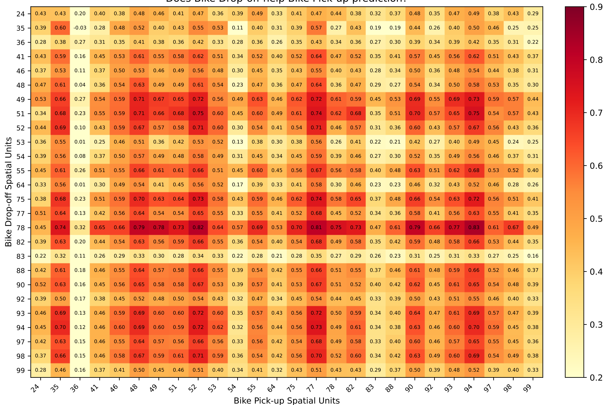
Lag: -15min - Correlation between Bike Drop-off and lagged Bike Pick-up time-series - Lyon. Does Bike Drop-off help Bike Pick-up prediction?
