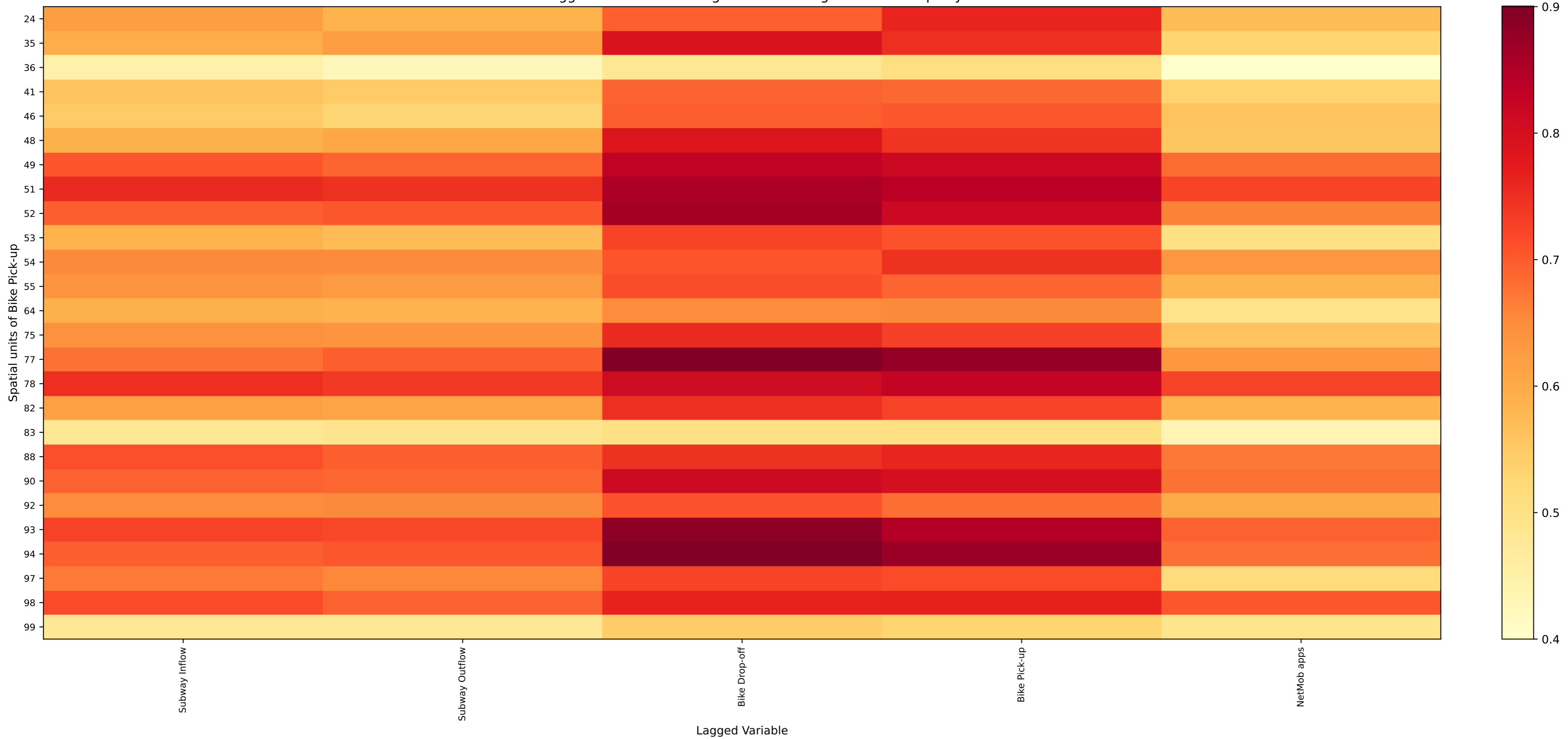
Cross-Lagged Correlation at Lag -15min for Target: Bike Pick-up - Lyon.
