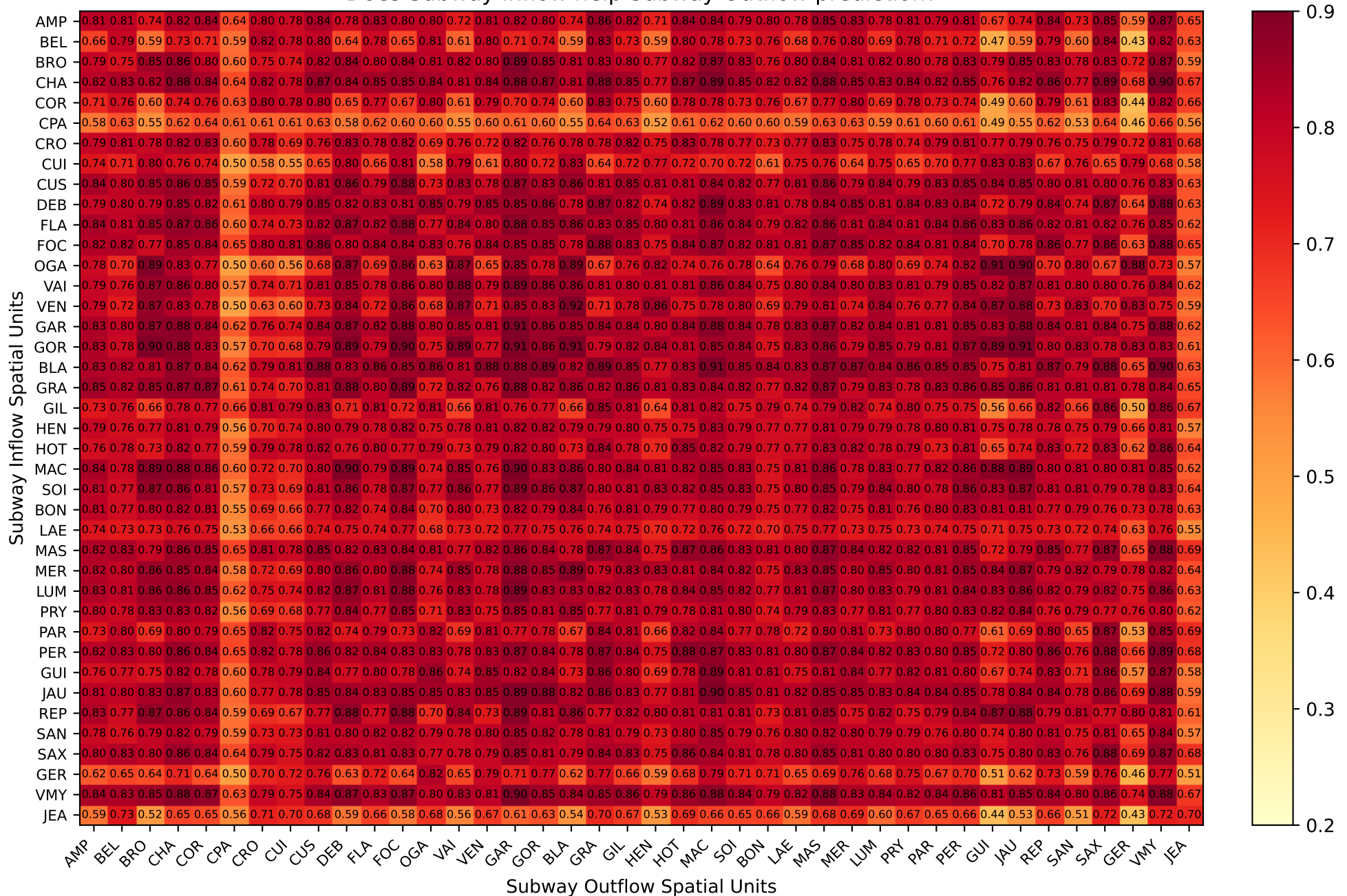
Lag: -30min - Correlation between Subway Inflow and lagged Subway Outflow time-series - Lyon. Does Subway Inflow help Subway Outflow prediction?
