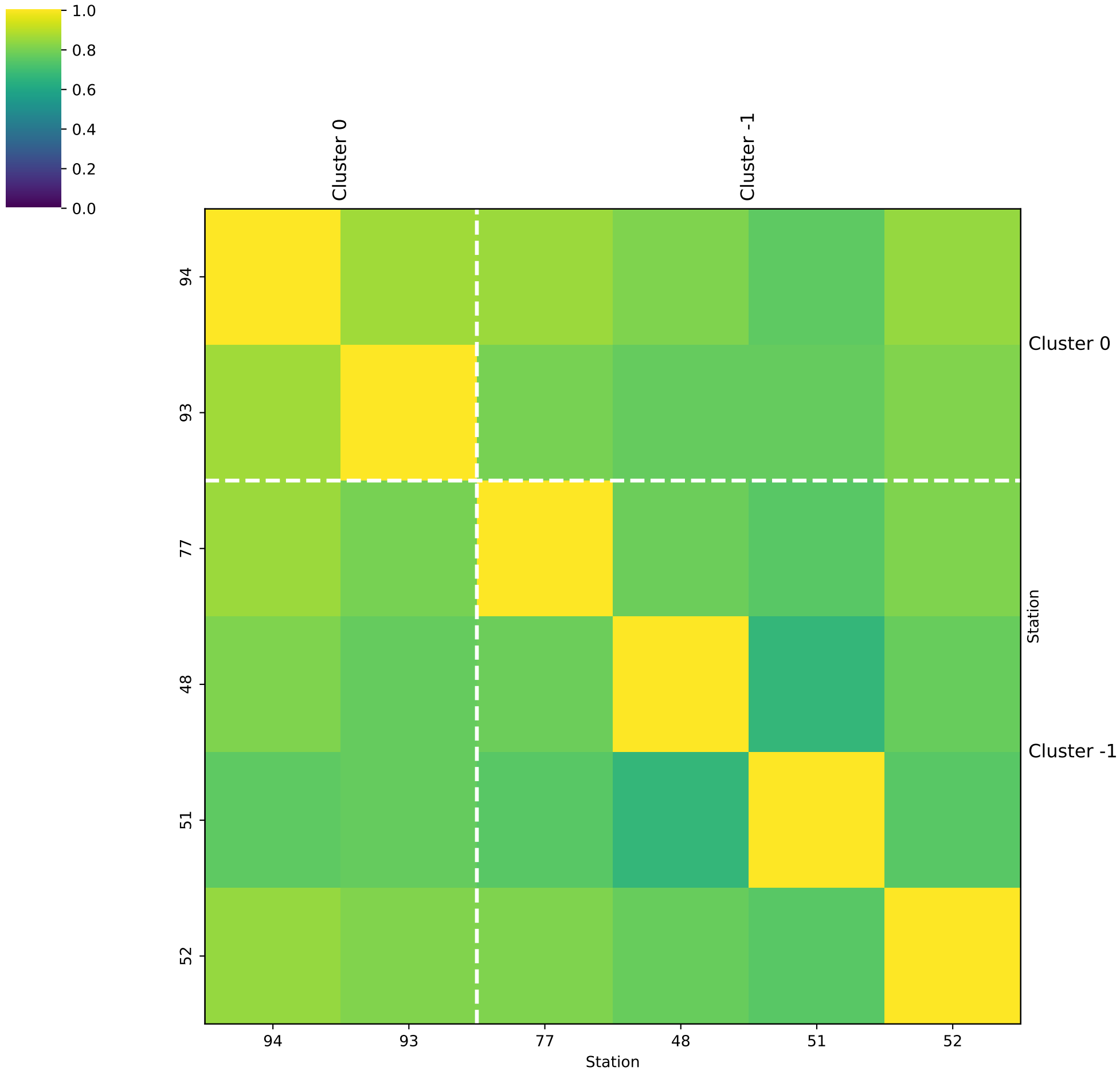
Correlation Matrix Heatmap (Ordered by Cluster)
