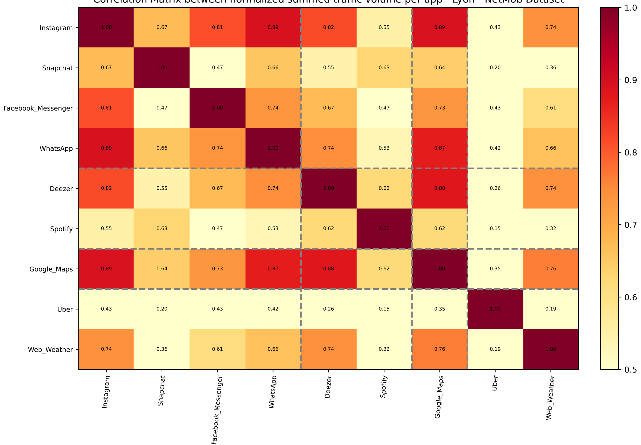
Correlation Matrix between normalized summed traffic volume per app - Lyon - NetMob Dataset
