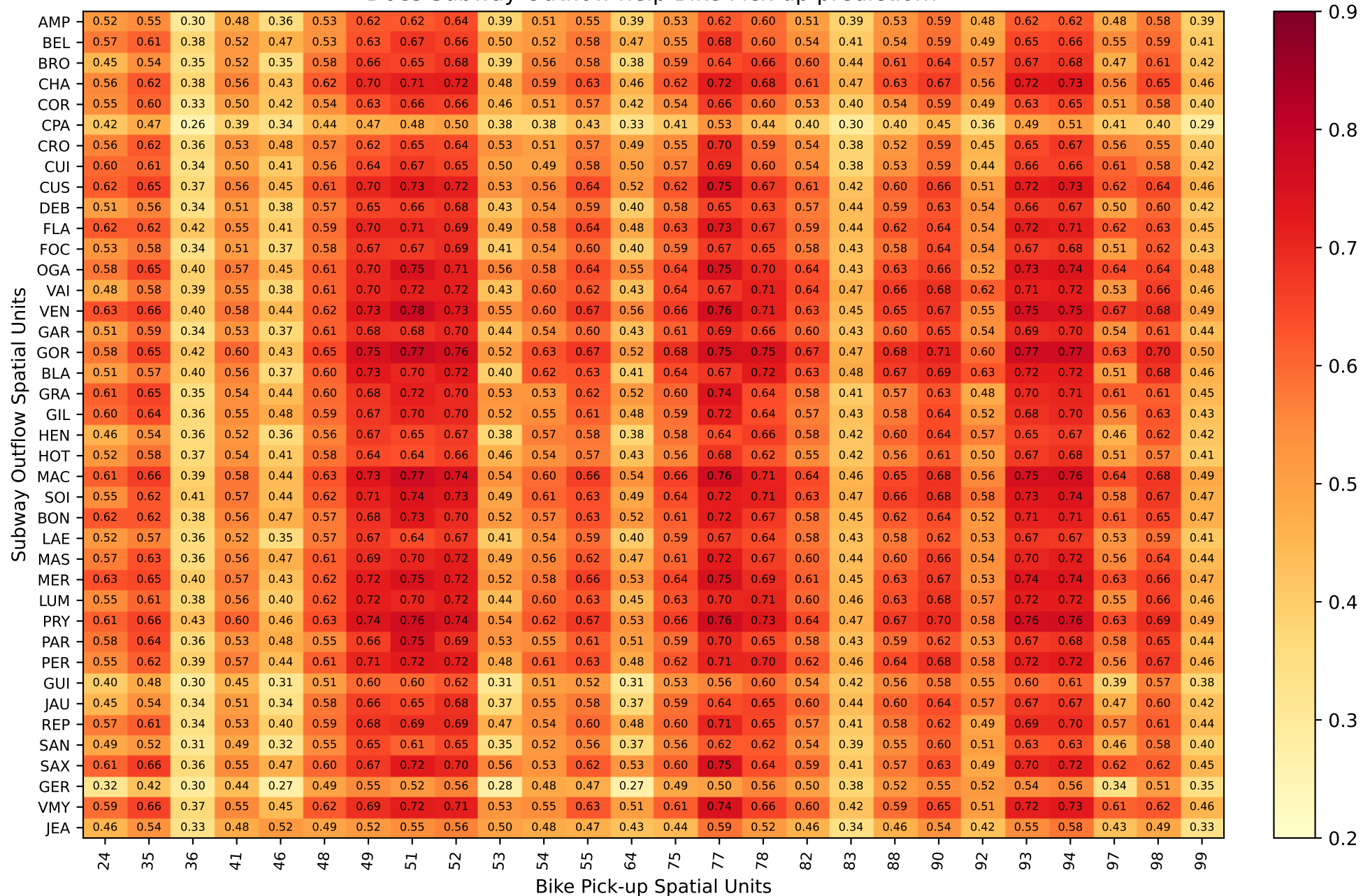
Lag: -15min - Correlation between Subway Outflow and lagged Bike Pick-up time-series - Lyon. Does Subway Outflow help Bike Pick-up prediction?
