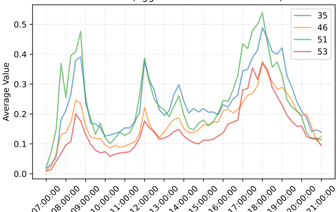
Cluster 1 (agglomerative-based Profiles)
