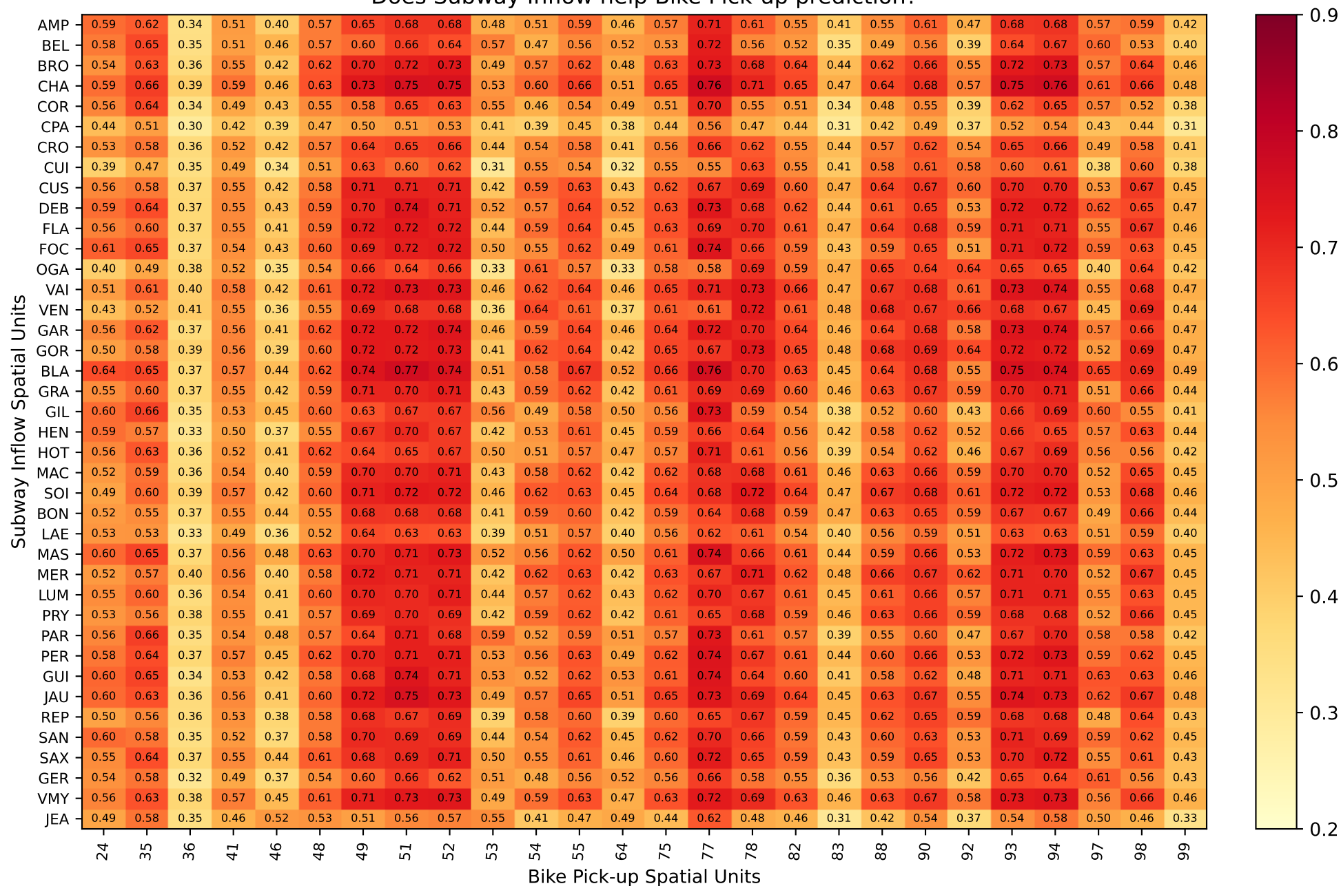
Lag: -2 - Correlation between Subway Inflow and lagged Bike Pick-up time-series - Lyon. Does Subway Inflow help Bike Pick-up prediction?
