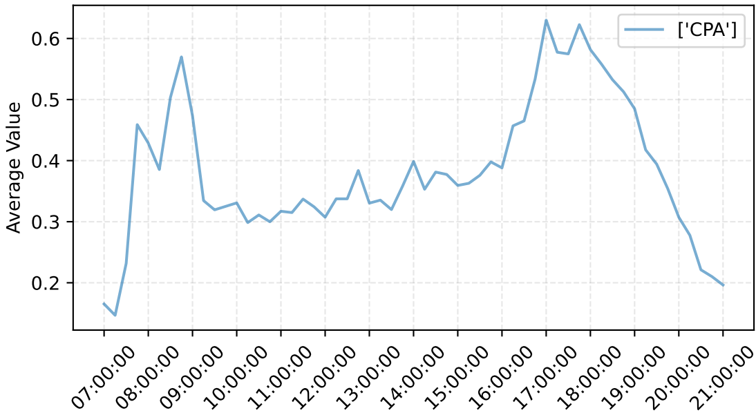
Cluster -1 (agglomerative-based Profiles)
