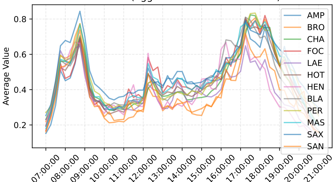
Cluster 0 (agglomerative-based Profiles)
