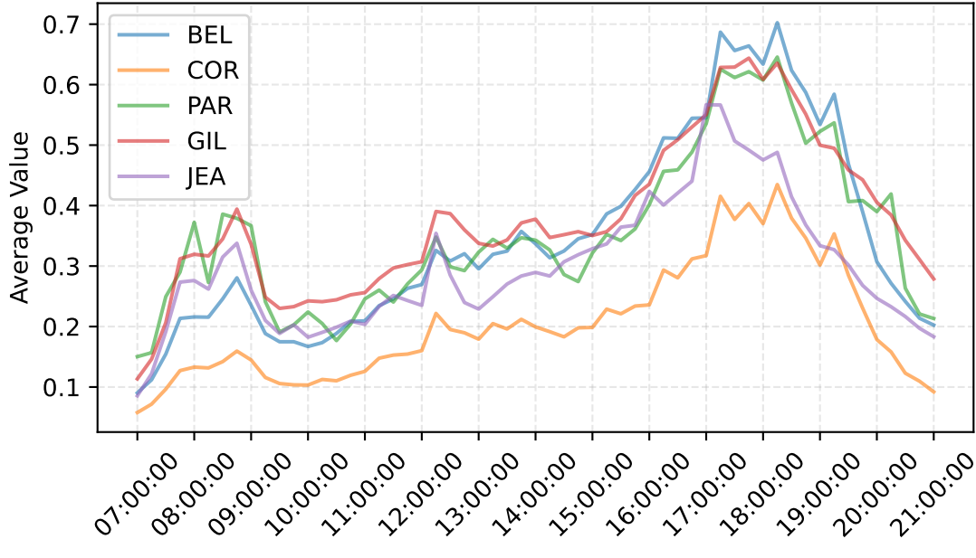
Cluster 2 (agglomerative-based Profiles)
