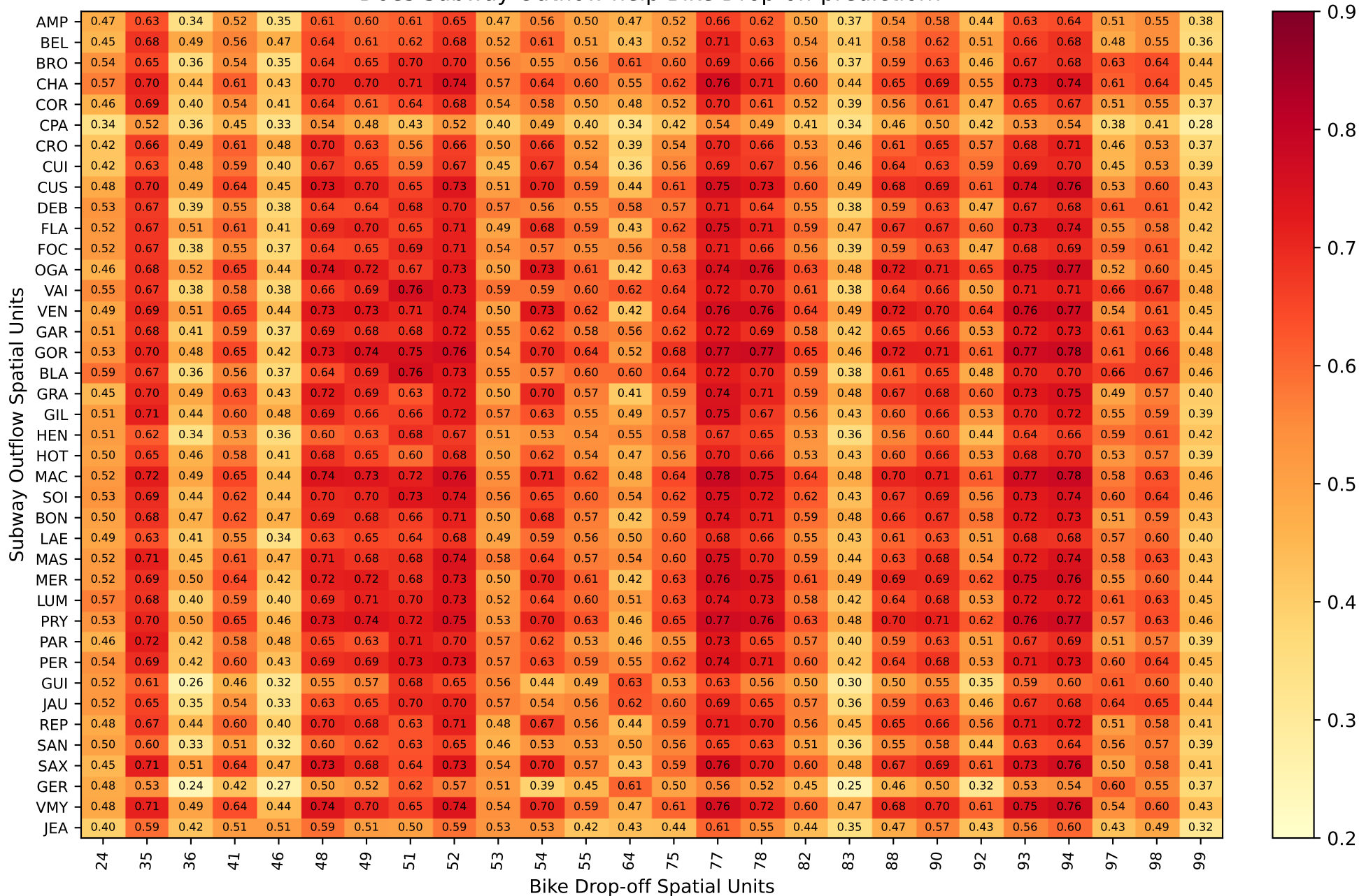
Lag: -15min - Correlation between Subway Outflow and lagged Bike Drop-off time-series - Lyon. Does Subway Outflow help Bike Drop-off prediction?
