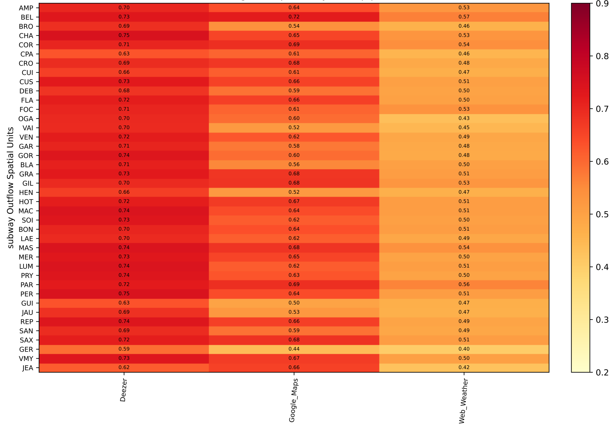
Lag: -15min - Correlation between subway Outflow and lagged NetMob time-series - Lyon. Does NetMob signal help subway Pick-up prediction?
