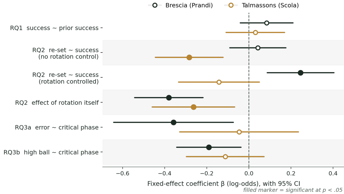
Figure 4. Fixed-effect coefficients with 95% confidence intervals for all models. Intervals crossing the dashed zero line are not statistically significant. The two middle rows show how the RQ2 results change after controlling for rotation: the negative effect for Talmassons is no longer significant, while a positive significant effect emerges for Brescia.
