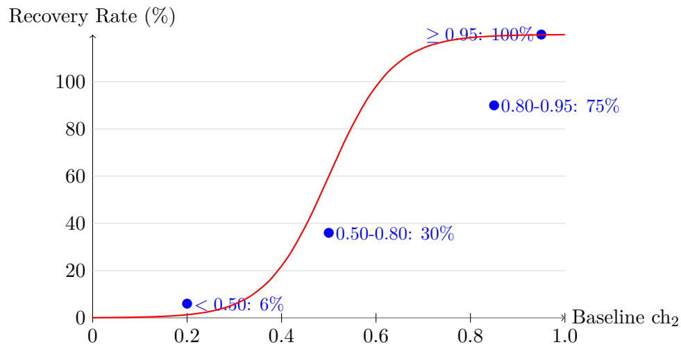
Figure 30.2: 6-month recovery rate vs. baseline ch_2^{\text{clinical}} . Strong dose-response relationship (logistic fit, AUC = 0.89).
