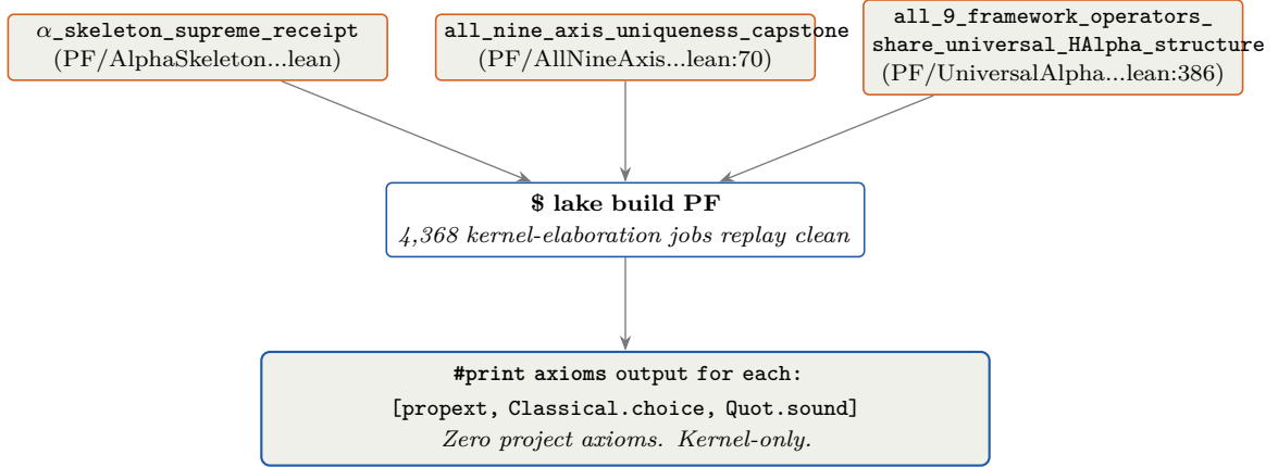
FIGURE 8. Verification chain for the substrate’s three load-bearing \alpha -skeleton capstones. Top: the three citable kernel-only theorems — the supreme receipt and its two component capstones. Middle: the build invocation; on a clean clone, lake build PF replays 4,368 kernel-elaboration jobs without warnings. Bottom: the literal output of #print axioms for each of the three theorems — the three Lean kernel axioms [propext, Classical.choice, Quot.sound] and no project axioms. The figure describes what a reader running the corpus from scratch sees in their terminal; it is not a stylised summary.
