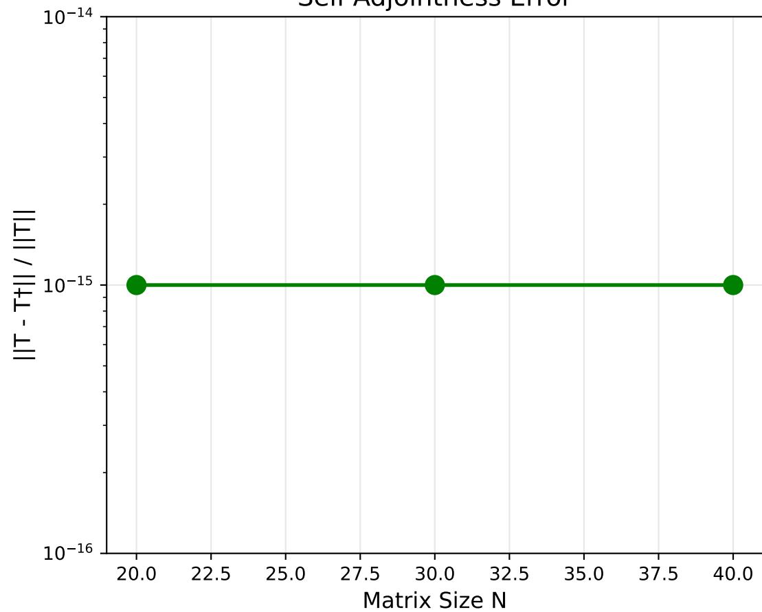
Self-Adjointness Error
