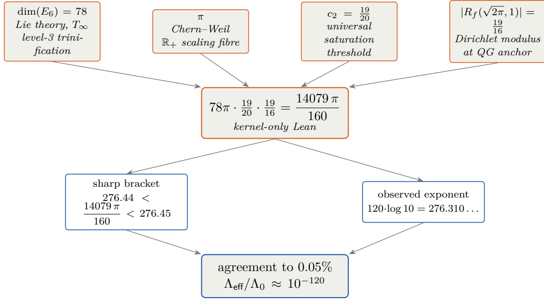
FIGURE 6. The substrate’s parameter-free derivation of \Lambda_{\text{eff}}/\Lambda_0 \sim 10^{-120} . Top row: four substrate-internal inputs — \dim(E_6) = 78 (Lie theory, forced by T_\infty level-3 trinification, kernel-only theorem seventyEight_decomp in PF/Cosmology/E6ChernIndex78pi.lean ); \pi (Chern–Weil normalisation with \mathbb{R}_+ scaling fibre); c_2 = 19/20 (universal saturation threshold, PF/Consciousness/Ch12MassIITBridge.lean ); |R_f(\sqrt{2}\pi, 1)| = 19/16 (Dirichlet-series modulus at the QG anchor). Middle: their product collapses to the rational closed form 14079\pi/160 , kernel-only proven as Lambda_eff_exponent_product_rational_form in PF/Cosmology/LambdaEffParameterFreeCapstone.lean . Lower row: the substrate’s certified sharp bracket 276.44 < 14079\pi/160 < 276.45 versus the observed cosmological exponent 120 \log 10 = 276.310\dots . Bottom: the substrate’s closed form matches the observed hierarchy to 0.05%. No quantity in the chain is fit to the cosmological observation; the exponent 120 in 10^{-120} is a derived consequence of the chain, not an input. The match is 0.05% on the exponent (residual 0.13 within the substrate-natural rational precision on |R_f| ).
