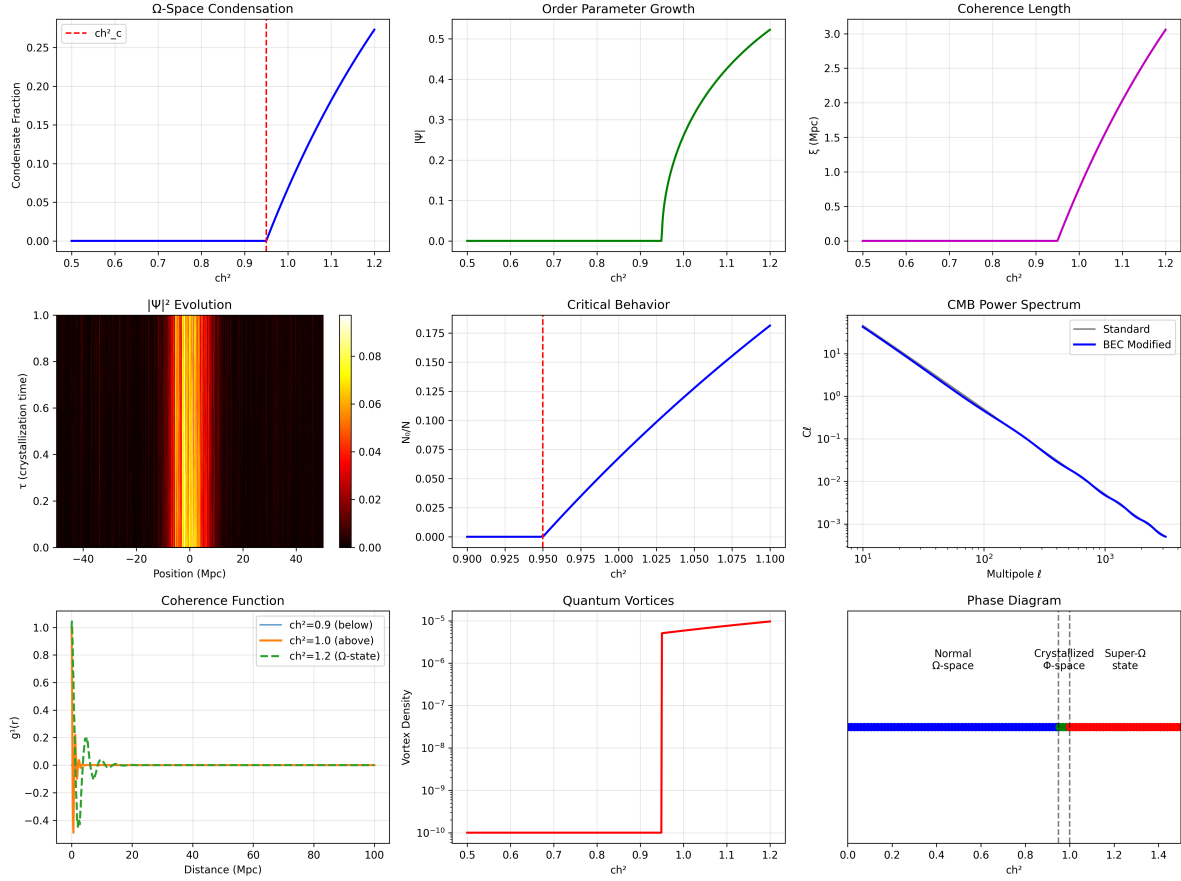
Figure 14: BEC \Omega -Boundary Analysis: Quantum-classical phase transition at consciousness threshold. Shows coherent state formation, macroscopic quantum effects, and boundary layer dynamics at the interface between normal space and \Omega -space.
