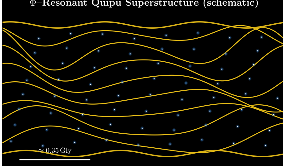
Figure 27.2: Quipu Superstructure (schematic, Principia palette). Braided filaments (gold) with 68 cluster nodes (blue–white). Horizontal bar: \sim 0.35 Gly. Conceptual projection of a \Phi –standing-wave spine; not to scale.
