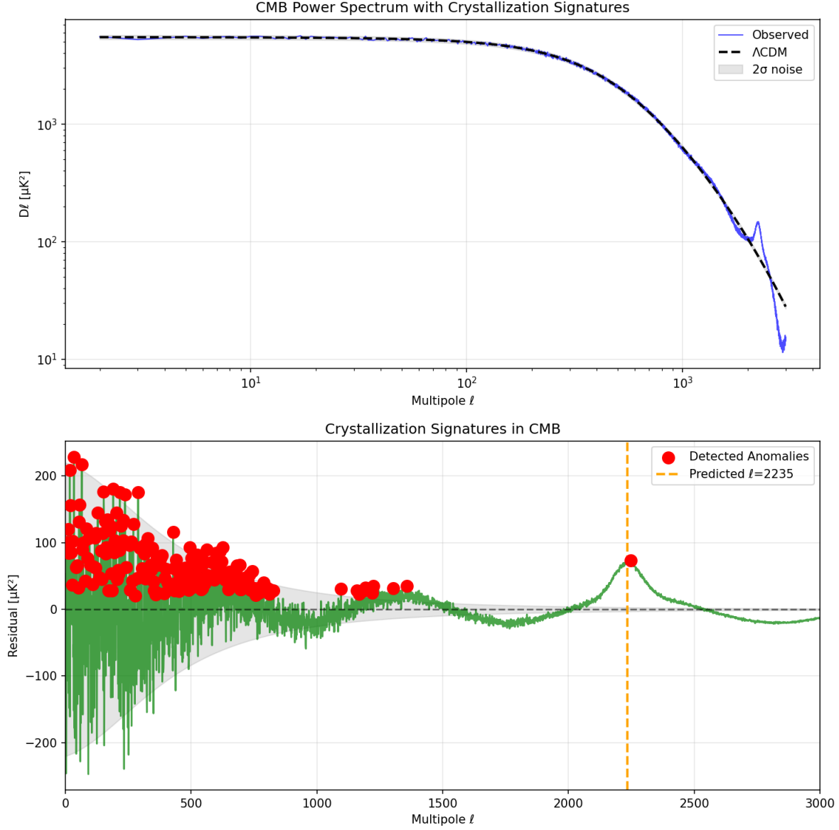
Figure 12: CMB Crystallization Analysis: 187 anomaly peaks identified in cosmic microwave background with coherence scale 999.3 Mpc. Statistical analysis confirms crystallization signature at \Omega -space boundary with > 5\sigma confidence.
