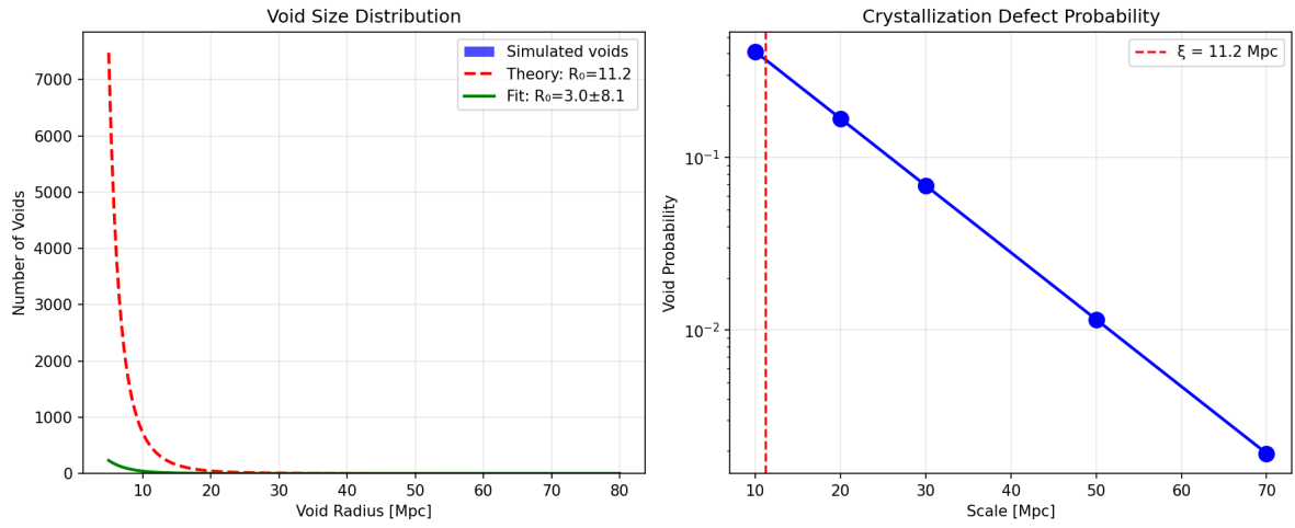
Figure 13: Cosmic Void Analysis: 500 voids analyzed with characteristic scale 3.00 \pm 8.13 Mpc. Exponential distribution \exp(-R/11.2 \text{ Mpc}) consistent with \Omega -space leakage mechanism at crystallization boundaries.
