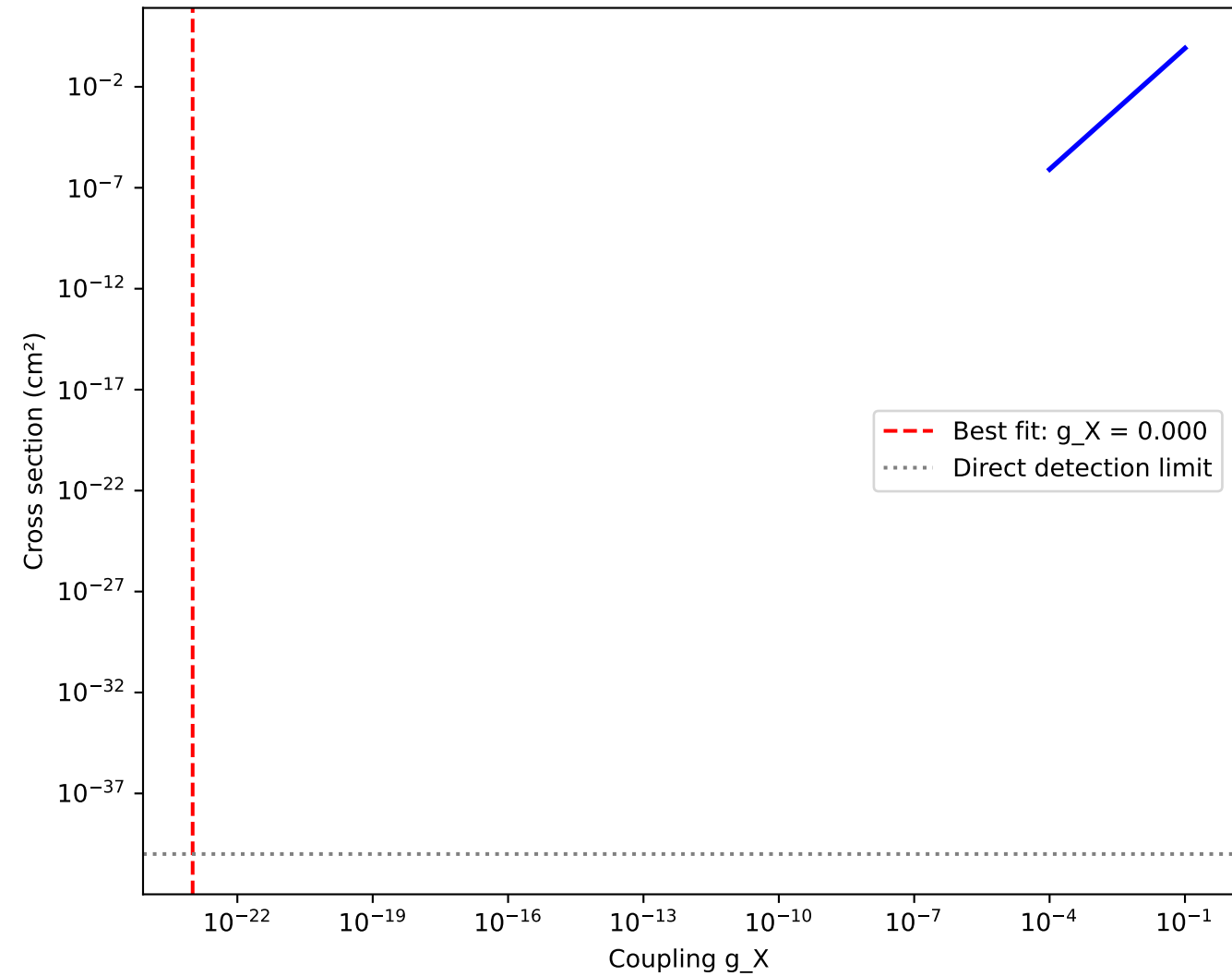
Dark Matter Coupling Constraints
