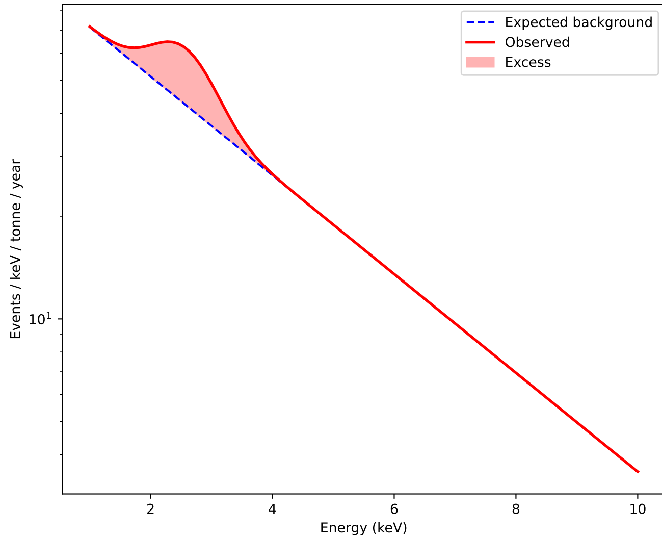
XENON1T Energy Spectrum
