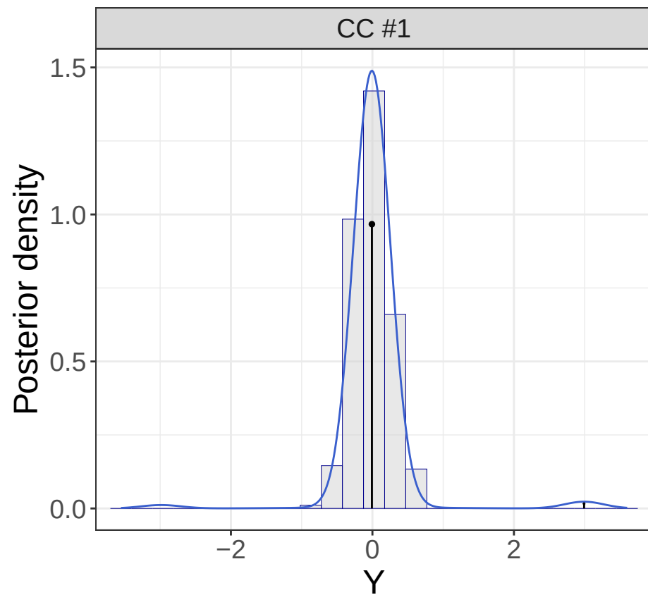
CC posterior density estimate with common atoms
