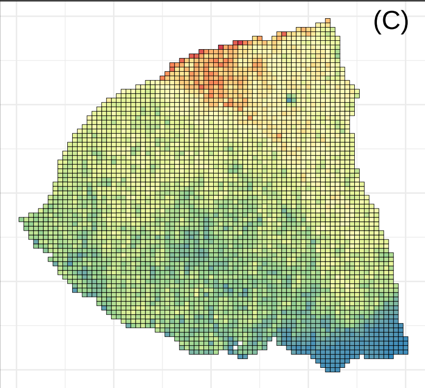
N-Glycans
