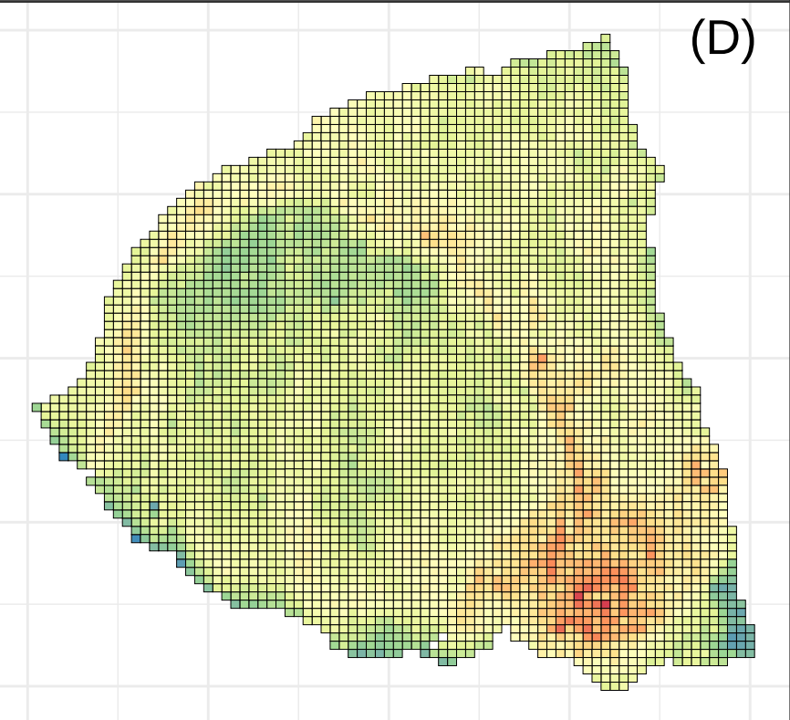
Peptides
