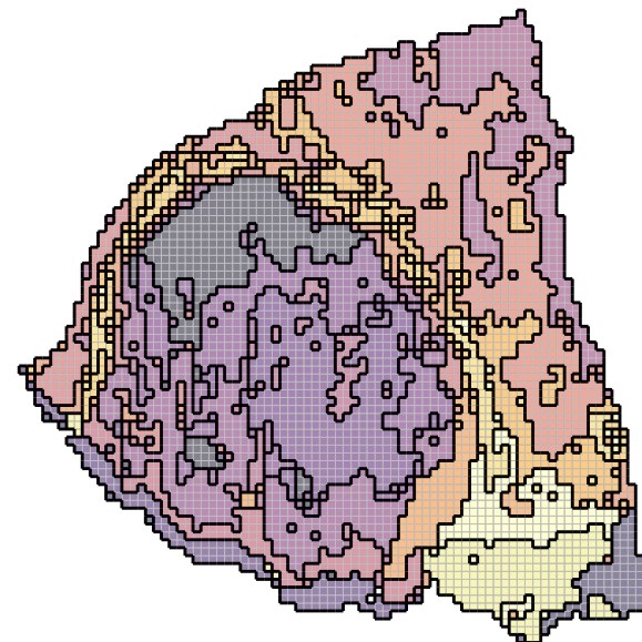
(E) Poseidon
