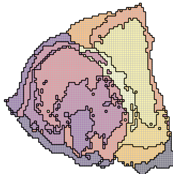
(E) Poseidon
