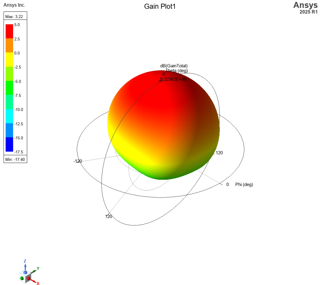
Figure 3.7: 3D gain, final circular patch
