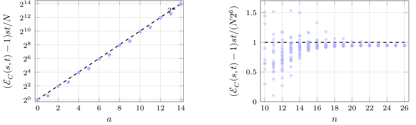
FIG. 4. Numerical check of the a = 0 base scaling in Eq. (E55) and of the dyadic extension in Eq. (E60). The data are obtained by exact state-vector evaluation at n = 26 for the fixed-phase HP-1 kernel, using s = 2^a u , t = 2^a v over 30 odd pairs (u, v) and a = 0, \dots, 14 . The left panel plots (\mathcal{E}_C(s, t) - 1)st/N , after removing the base N/(st) overlap scale; borderless light-blue circles are individual period-pair overlaps and the black dashed curve shows 2^a . The right panel fixes a = 6 and sweeps n = 10, \dots, 26 , plotting the normalized residual (\mathcal{E}_C(s, t) - 1)st/(N2^6) . The black dashed line marks the unit residual; apart from a few small- n finite-size outliers above the plotted range, the absence of exponential drift in n supports the shared 2-adic depth, rather than an additional n -exponential factor, as the leading statistical enhancement.
