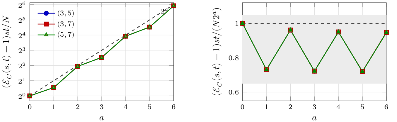
FIG. 4. Numerical check of the dyadic-resonance scaling in Eq. (E50). The data are obtained by exact CUDA state-vector evaluation at n = 20 for the fixed-phase HP -1 kernel, using the pairs s = 2^a u , t = 2^a v with (u, v) = (3, 5), (3, 7), (5, 7) and a = 0, \dots, 6 . The left panel plots (\mathcal{E}_C(s, t) - 1)st/N , after removing the base N/(st) overlap scale. The right panel divides the same quantity by 2^a ; the result remains order one up to finite-size fluctuations, supporting the shared 2-adic depth as the leading statistical enhancement.
