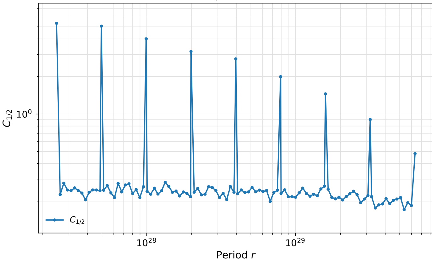
Fixed-phase HP-1 C_{1/2} scan, sampled r , n = 100
