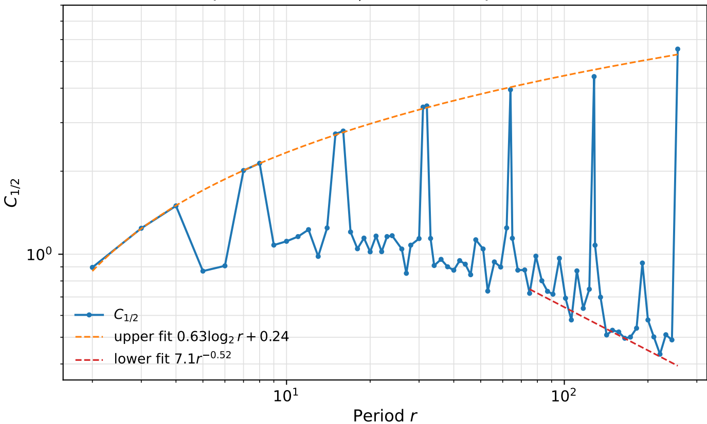
Fixed-phase HP-1 C_{1/2} scan, sampled r, n = 16
