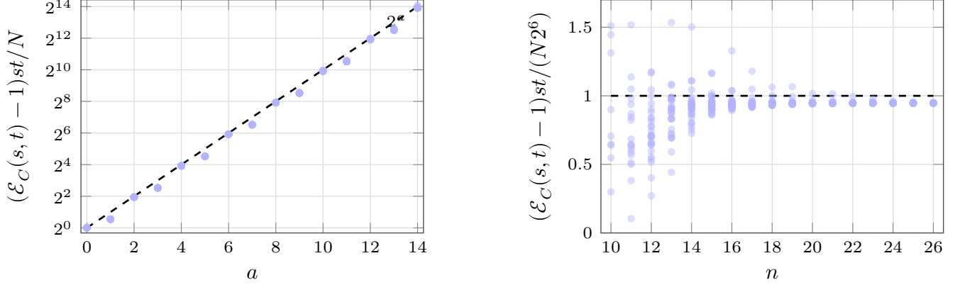
FIG. 4. Numerical check of the a = 0 base scaling in Eq. (E55) and of the dyadic extension in Eq. (E60). The data are obtained by exact state-vector evaluation at n = 26 for the fixed-phase HP - 1 kernel, using s = 2^a u , t = 2^a v over 30 odd pairs (u, v) and a = 0, \dots, 14 . The left panel plots (\mathcal{E}_C(s, t) - 1)st/N , after removing the base N/(st) overlap scale; borderless light-blue circles are individual period-pair overlaps and the black dashed curve shows 2^a . The right panel fixes a = 6 and sweeps n = 10, \dots, 26 , plotting the normalized residual (\mathcal{E}_C(s, t) - 1)st/(N2^6) . The black dashed line marks the unit residual; apart from a few small- n finite-size outliers above the plotted range, the absence of exponential drift in n supports the shared 2-adic depth, rather than an additional n -exponential factor, as the leading statistical enhancement.
