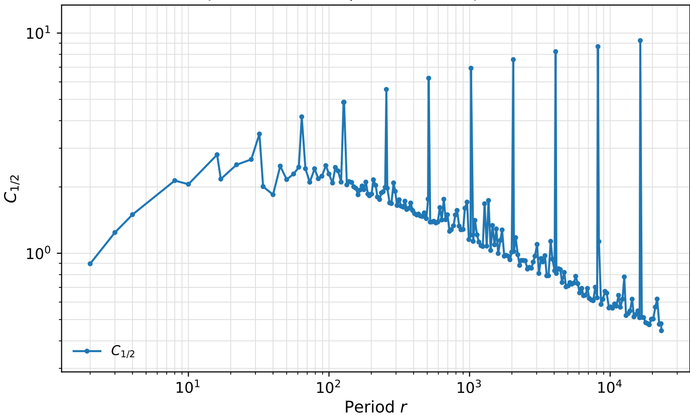
Fixed-phase HP-1 C_{1/2} scan, sampled r , n = 29
