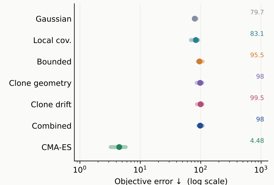
Rastrigin
