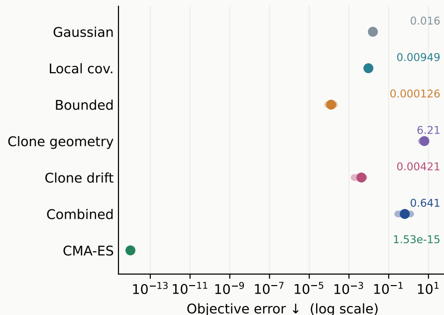
Quadratic bowl
