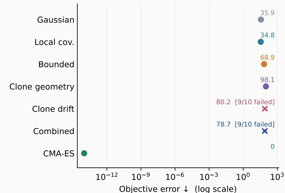
Boundary optimum
