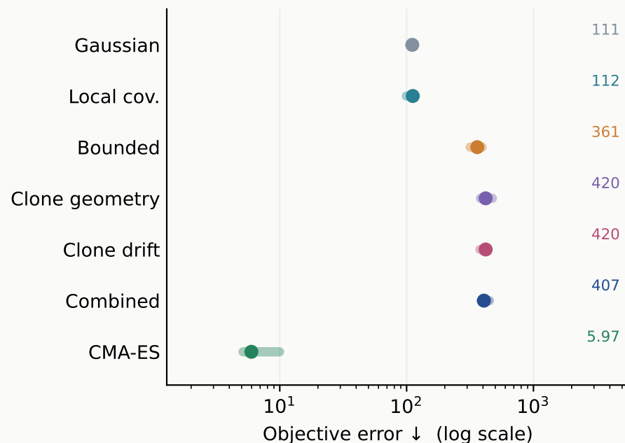
Rotated Rastrigin
