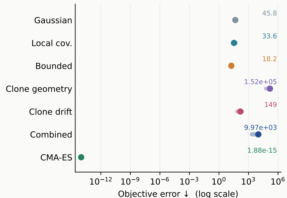
Rosenbrock
