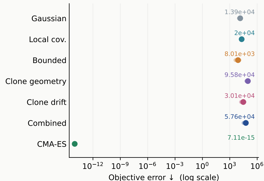
Rotated ellipsoid
