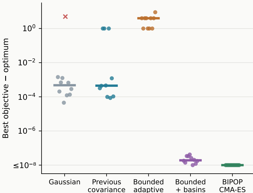
Rotated Rastrigin
