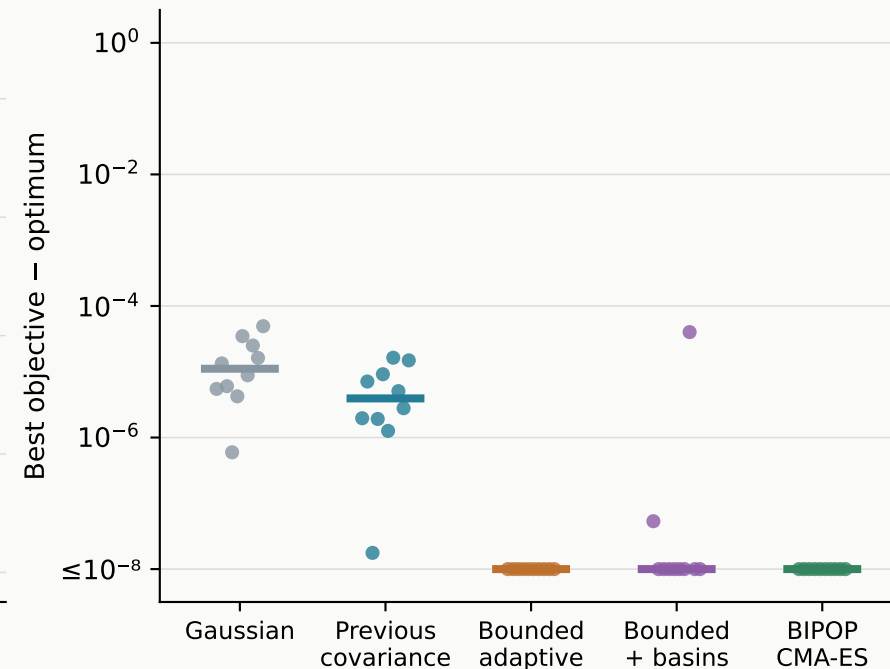
Rosenbrock
