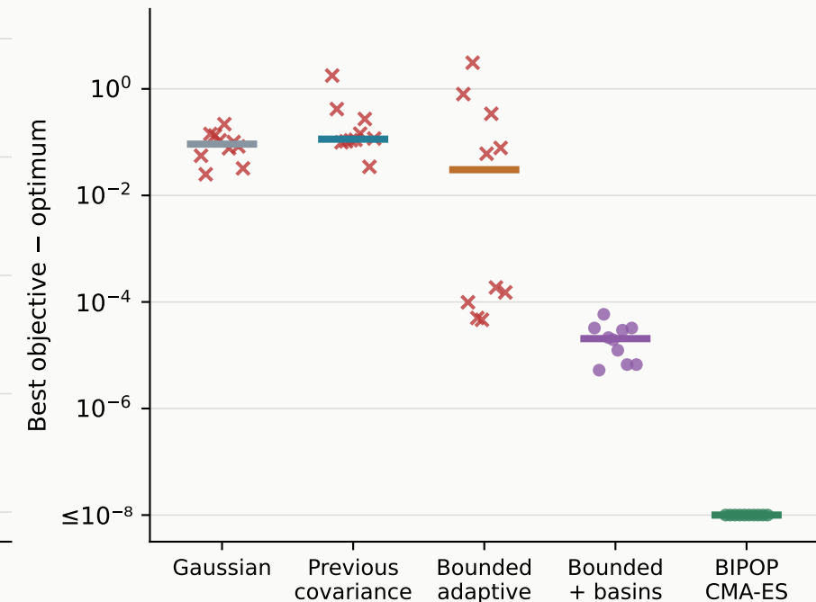
Boundary optimum
