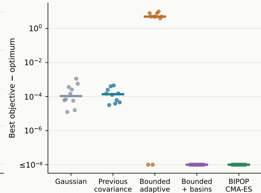
Boundary optimum
