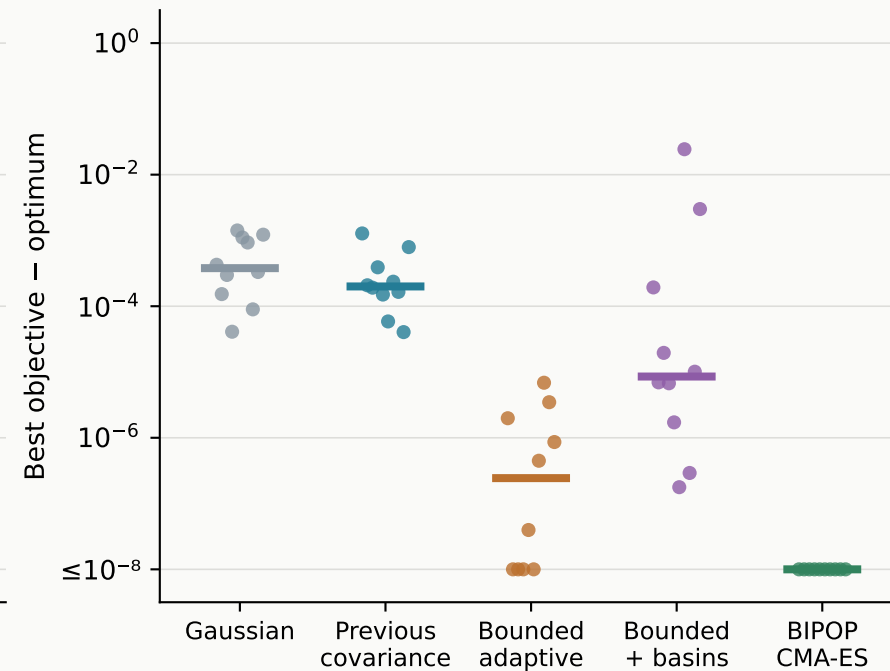
Rosenbrock
