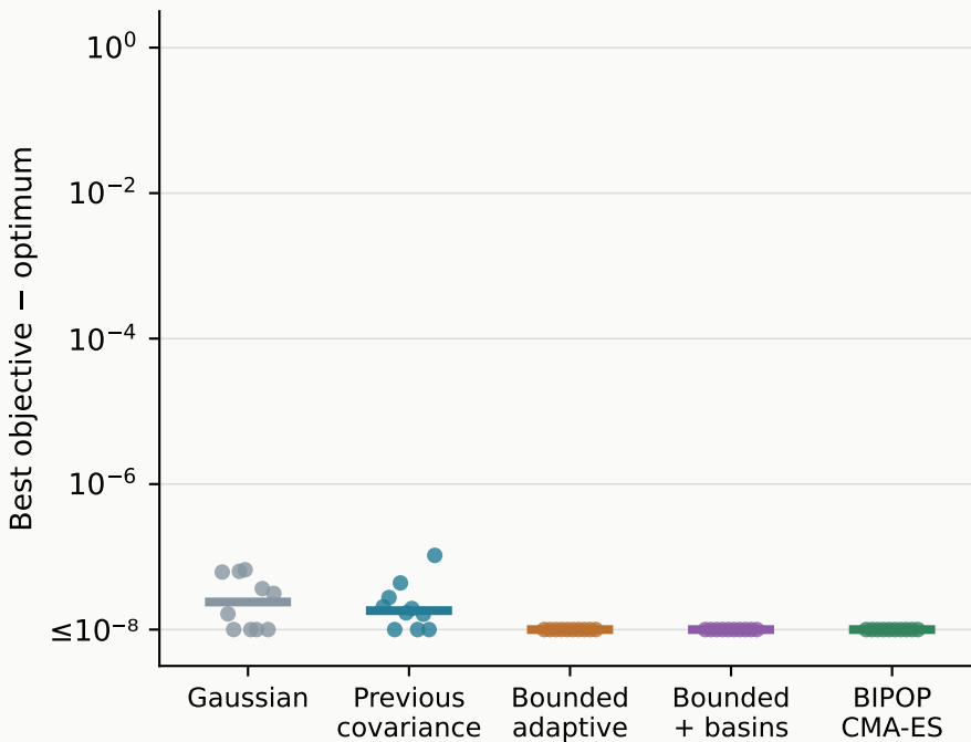
Rotated Rastrigin
