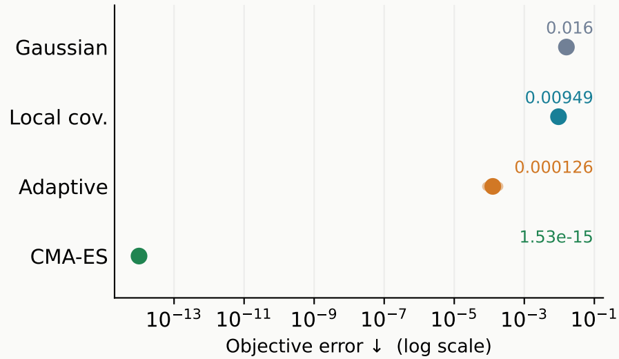
Quadratic bowl
