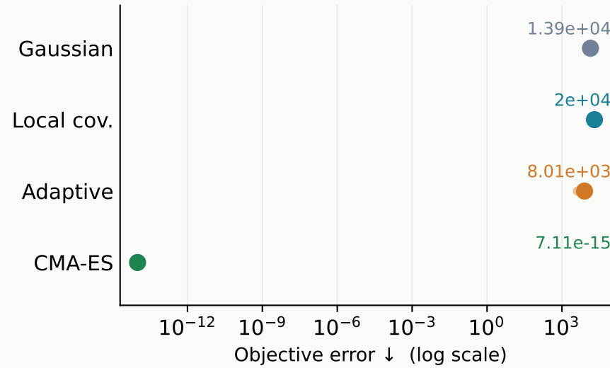
Rotated ellipsoid
