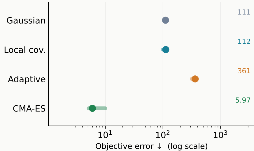
Rotated Rastrigin
