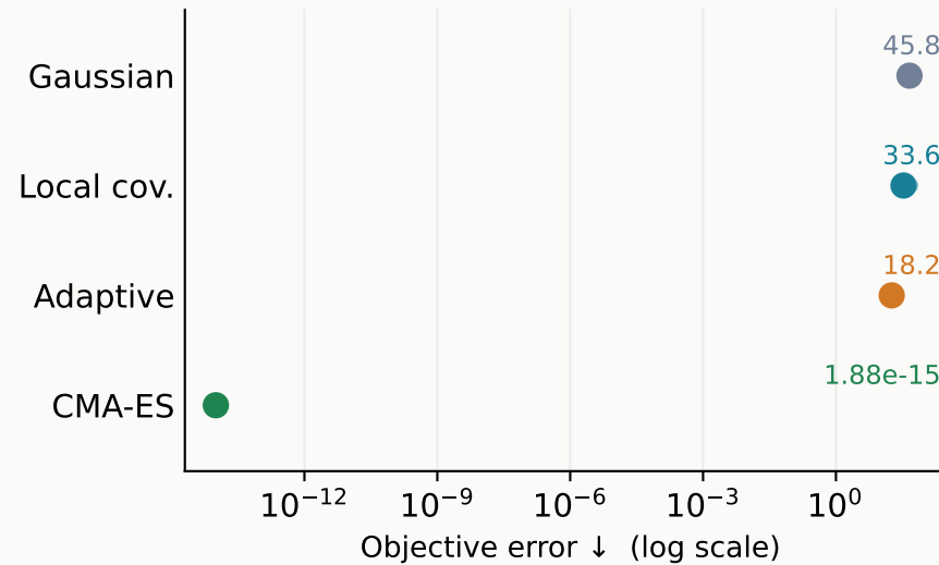
Rosenbrock
