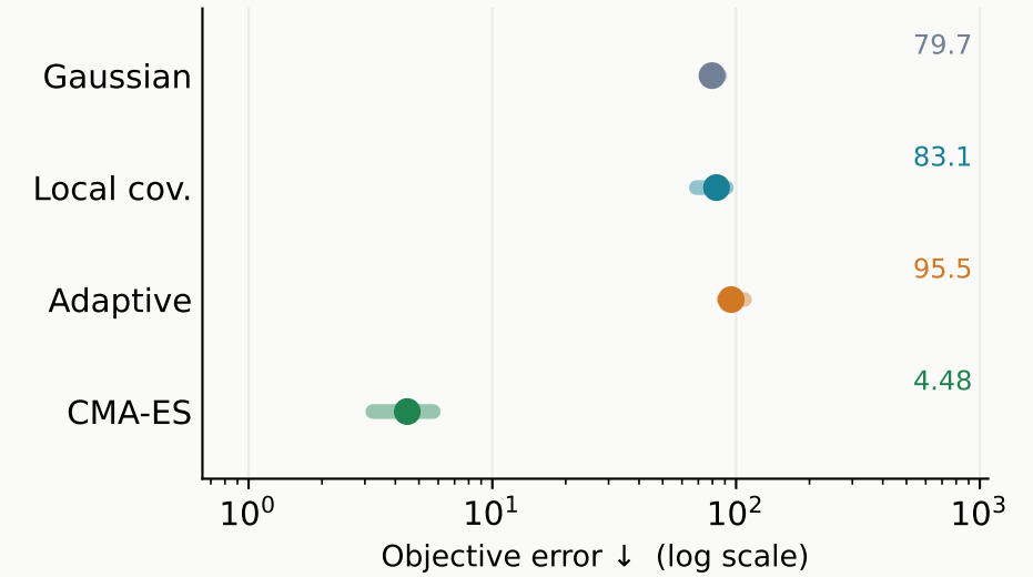
Rastrigin
