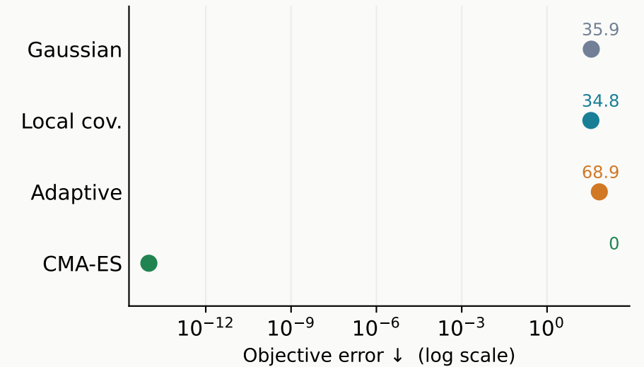
Boundary optimum
