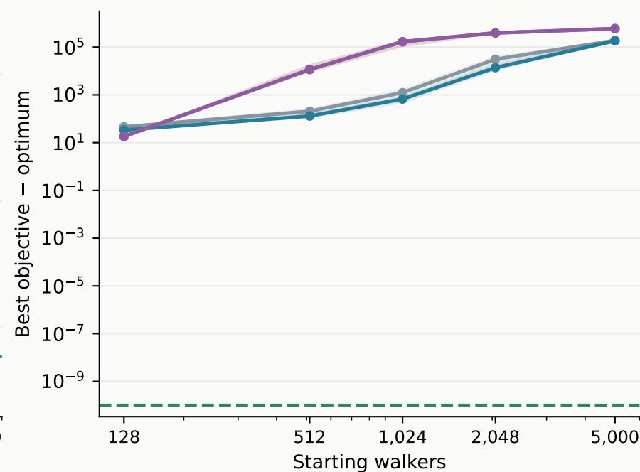
Rosenbrock
