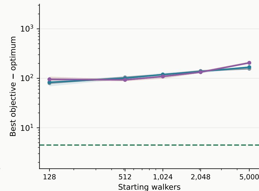
Boundary optimum
