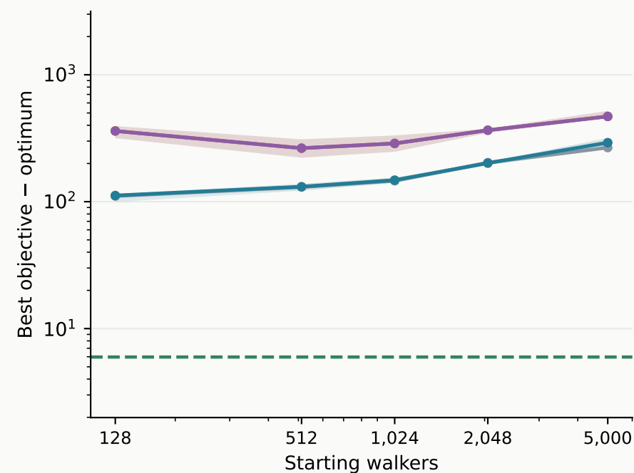
Rotated Rastrigin
