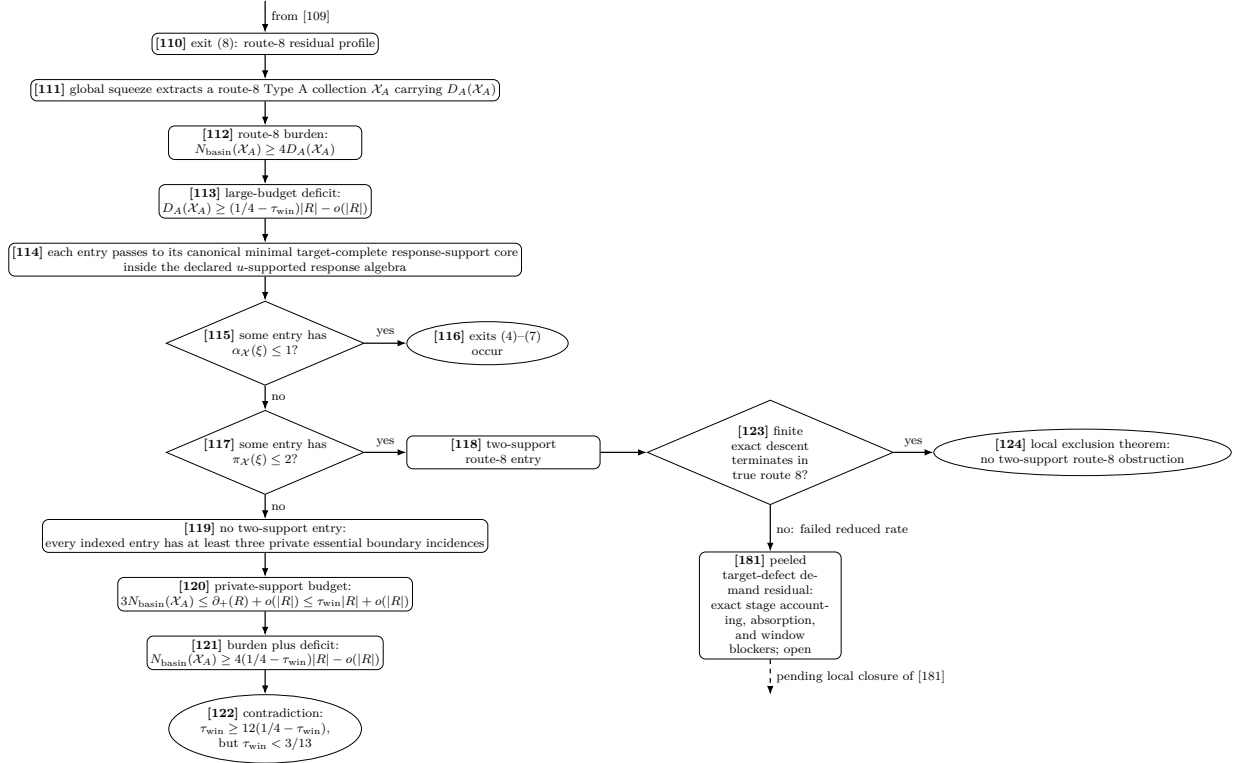
Figure 9: Proof-dependency diagram, Part IX. Rectangles, diamonds, ellipses, bracketed node numbers, and edge labels use the convention of Fig. 1. The figure expands exit (8) from Fig. 8 and records how it feeds the demand routing. On the derived spine branch, the route-8 response-support reduction closes the no-two-support branch: the global squeeze extracts \mathcal{X}_A carrying D_A , the route-8 burden gives N_{\text{basin}} \geq 4D_A , zero/one-essential-core entries trigger exits (4)–(7), and absence of a two-support entry gives 3N_{\text{basin}} \leq \tau_{\text{win}}|R| + o(|R|) , contradicting 3N_{\text{basin}} \geq 12(1/4 - \tau_{\text{win}})|R| - o(|R|) and \tau_{\text{win}} < 3/13 . A two-support entry enters the exhaustive decision at node [123]. Every target-defect peel decreases \Lambda_4 , and the exact identities \tilde{\Xi} = \tilde{\Xi}^{P_4} \dot{\cup} \tilde{P}_4 and 4\tilde{D}_A = 4\tilde{D}_A^{P_4} + p_4 retain its contribution. Termination in a true route-8 entry is sent to node [124], where the local exclusion theorem closes that branch. The complementary failed reduced-rate outcome runs the full demand, absorption, and unique-window blocker ledgers and publishes the still-open peeled target-defect demand residual at node [181]. The dashed arrow below [181] denotes the pending continuation only; it does not assert closure.
