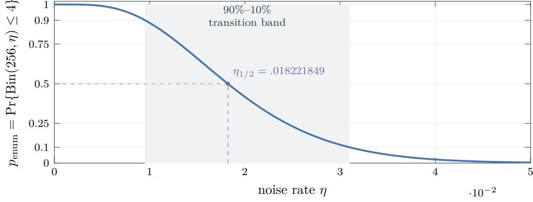
Figure 122: Exact binomial success transition for enumeration through error weight k_B = 4 with m = 256 samples. The curve is \sum_{j=0}^4 \binom{256}{j} \eta^j (1-\eta)^{256-j} . Its 90%, 50%, and 10% crossings are 0.009531622, 0.018221849, and 0.030981875, respectively. The general budget-dependent curve is Eq. (1190) with the exact affordable radius from Eq. (1189).
