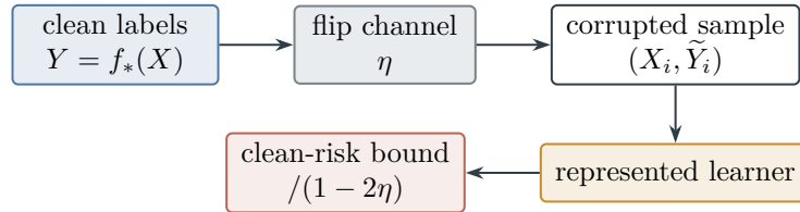
Figure 52: Symmetric corruption attenuates clean-label advantage by 1 - 2\eta . The represented learner pays the existing Rademacher, effective-dimension, PAC–Bayes, and operator-selection terms; dividing the resulting corrupted-risk certificate by the attenuation factor gives the clean-risk bound.
