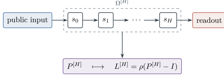
Figure 20: A bounded computation becomes a represented clocked transcript kernel and hence a positive generator by Lemma II.11.1.
