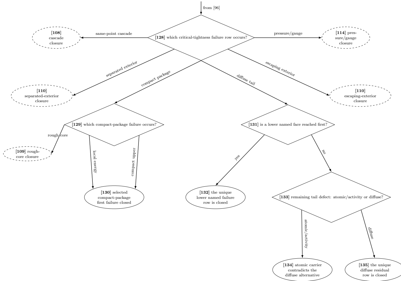
FIGURE 12. Proof-dependency diagram, Part XII. The six alternatives of lemma 10.103 leave [128] on separate edges. The compact-package and diffuse-tail cases are further split at [129] and [131]. The proof of lemma 10.104 tests for a lower named face first, then applies the atomic/diffuse dichotomy at [133]. Dashed ellipses refer to terminal closures already drawn in Parts IX–XI.
