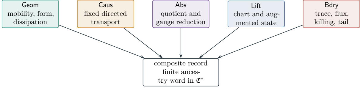
Figure 4: The five continuum source roles. The canonical native form split routes its positive symmetric output to Geom and its complete oriented bulk remainder to Caus. Abs and Lift record quotient and presentation currents, and Bdry records interface, exterior, and terminal currents. Composite records retain the union of their ancestries.
