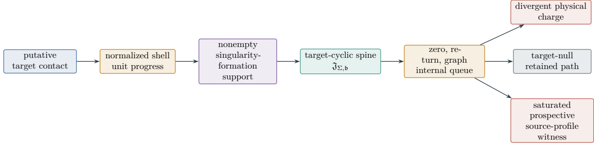
Figure 21: Compressed singularity-formation accounting. Contact exposes one target-aligned source cell. Projection-first saturation and signed gluing produce the target-cyclic feeding-storage spine. Zero-kernel restrictions, signed-dyadic return maps, and graph-boundary successors are internal queue transitions. On the contact-seeded branch the queue has three outputs: divergent physical charge, target-nullity, or a saturated prospective source-profile witness. Singular existence requires a separate independent-origin public-orbit realization.
