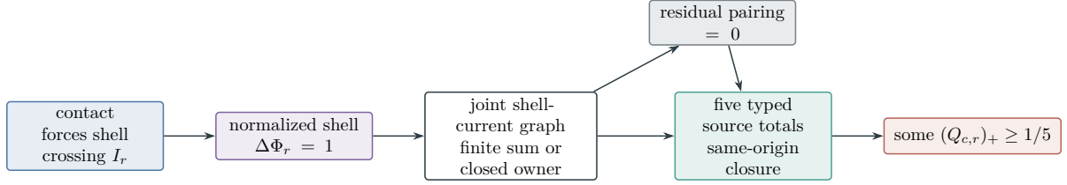
Figure 8: Normalized shell-crossing accountability. Contact forces a unit increase of the shell observable along the actual pre-contact current. The target-null residual contributes zero, so one of the five source integrals has positive part at least 1/5 .
