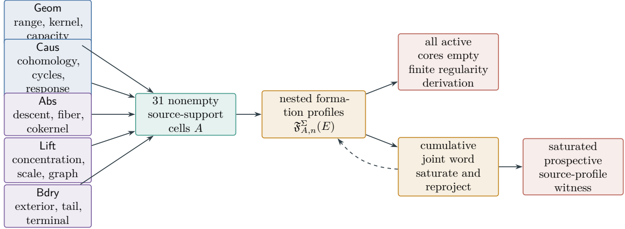
Figure 24: Direct continuum formation analysis. Each channel has a canonical target-local normal form and a finite invariant program. Their simultaneous supports produce 31 cells. Refinement either removes formation activity with stored identities or forms the cumulative joint word. Joint reprojection returns every newly exposed target component to its five-channel successor. A hypothetical joint fixed point carrying the unnormalized shell cocycle and complete source word is the saturated profile witness. Singular existence additionally requires independent origin and ordinary same-origin realization.
