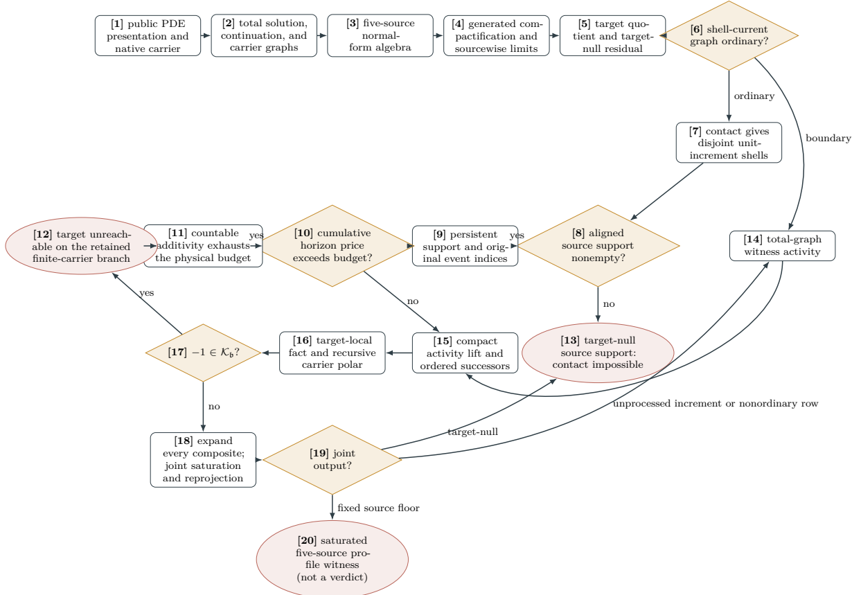
Figure 1: Target-reachability proof DAG. Public textbook data enter only at [1]. Nodes [2]–[6] generate the total graphs, source algebra, compactification, target quotient, and total shell graph. Its finite value gives the affine identity at [7], while every boundary value retains a positive owner and enters [14]. Thus [8] forces aligned support. Nodes [9]–[11] solve the unnormalized layered finite-horizon dual and close a branch as soon as its cumulative lower price exceeds the physical ceiling. Every ordinary or graph-boundary value also enters [14]; a bounded cumulative-price ledger joins it at [15]. Every invoked relation is restricted and source-factorized at [16] before it feeds the ordered cone at [17]. A checked finite identity gives [12]; the complementary order-unit functional generates a carrier-polar successor at [18]. Target-local polarity splitting, target-cyclic adjoint generation, recursive carrier-cone separation, covariant valuation, defect polarization, prospective reselection, and joint-prefix projection feed the exhaustive joint test at [19]. Its least unprocessed increment or nonordinary or nonfixed polar row returns to [14], while a target-null cumulative projection closes at [13]. A cofinal refinement retains the unnormalized shell cocycle and is reprojected as one saturated joint record. Only its simultaneously primal–polar fixed five-channel atom with its unnormalized source floor reaches [20]. Its contact-derived origin remains hypothetical; singular existence requires the independent approximation–orbit realization gate. No semantic compact-set assertion is used as an exclusion proof, and no analytic label is presented as a terminal.
