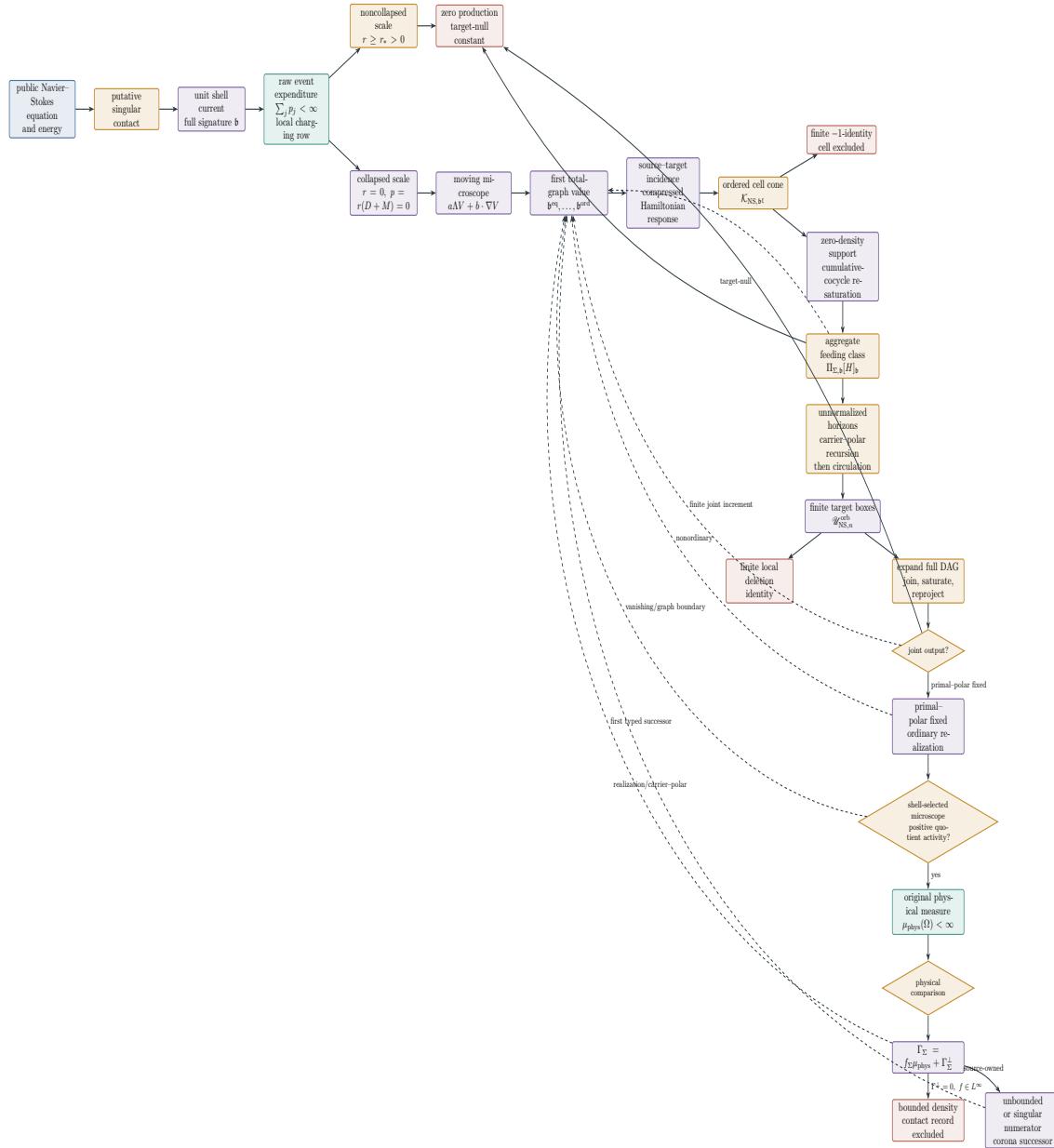
Figure 25: Navier–Stokes unit test. The microscope retains scale current; signed gluing precedes positive parts; incidence and carrier–polar descent process the five source owners; and every composite retains its full unnormalized cocycle. A fixed joint state enters the shell-selected same-origin microscope. Positive quotient activity gives the displayed scale-dependent price; vanishing activity or a graph boundary returns to the target-local successor cells. Exact financing retains the cumulative current, while persistent current undergoes first-scale rebasing and exhaustive critical-tail accounting. Every finite failure returns to a typed source cell; the diagonal tail is compared with the original physical carrier. Bounded density excludes that contact record; an unbounded or carrier-singular numerator is a source-owned corona successor returned to carrier–polar and ordinary-realization evaluation.
